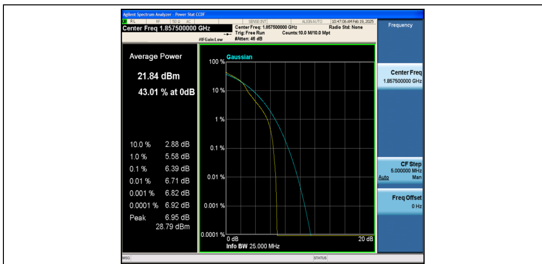
Band2-15MHz-16QAM-18675-1RB#0-PASS
