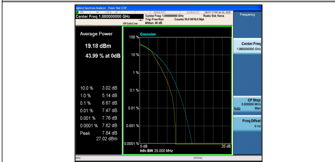
Band2-1.4MHz-16QAM-18900-6RB#0-PASS
