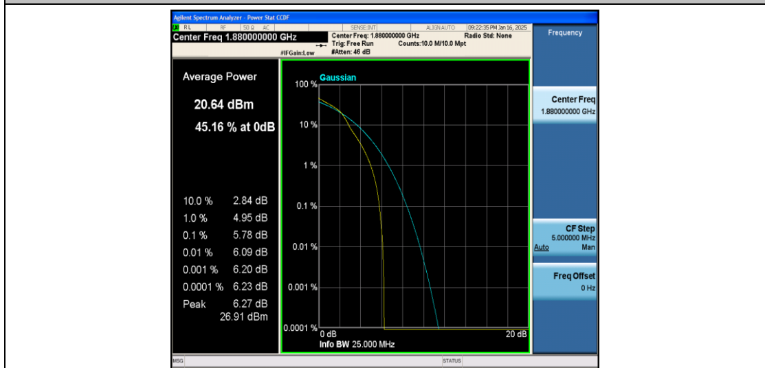
Band2-5MHz-16QAM-18900-1RB#0-PASS
