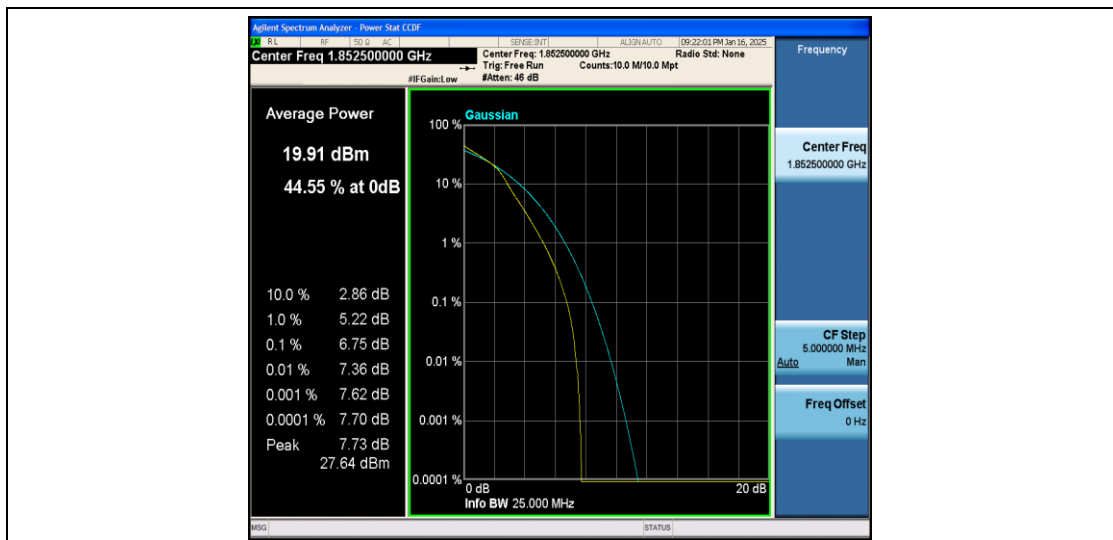
Band2-5MHz-16QAM-18625-25RB#0-PASS
