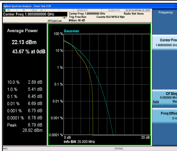
Band2-10MHz-16QAM-19150-1RB#0-PASS
