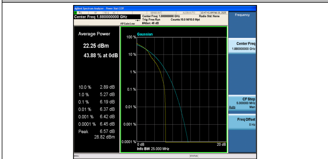
Band2-15MHz-16QAM-18900-1RB#0-PASS
