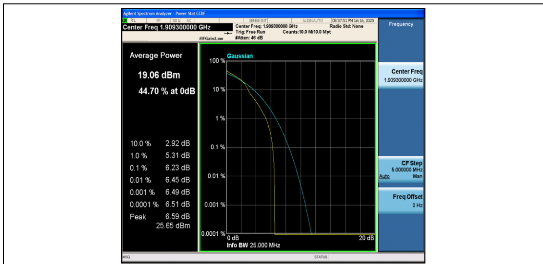
Band2-1.4MHz-16QAM-19193-1RB#0-PASS
