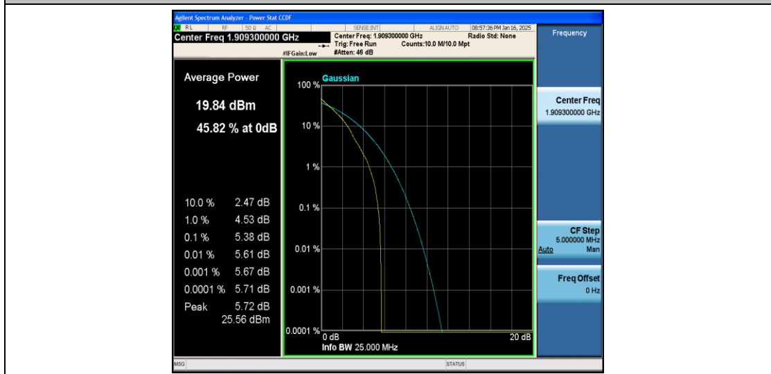
Band2-1.4MHz-QPSK-19193-1RB#0-PASS
