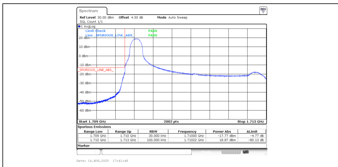
Band66_3MHz_QPSK_131987_1RB#0
