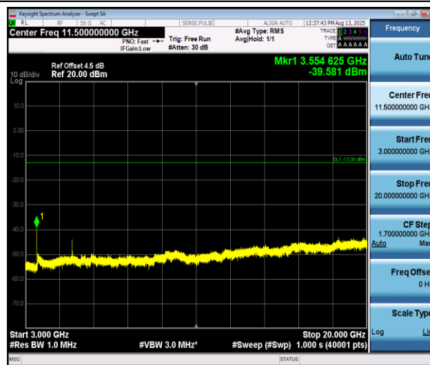
Band66_3MHz_16QAM_132657_1RB#0_3000~131022_3000~131022
