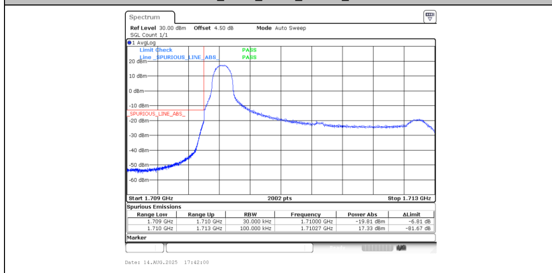
Band66_3MHz_16QAM_131987_1RB#0
