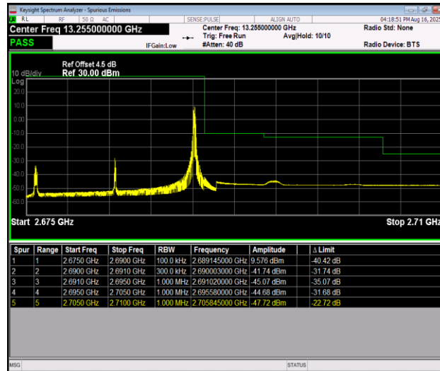
Band41_15MHz_16QAM_41515_1RB#74
