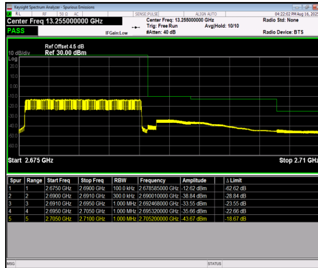
Band41_15MHz_16QAM_41515_75RB#0
