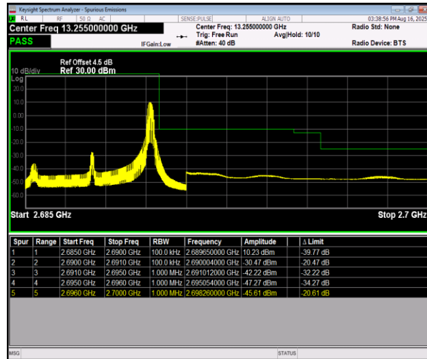
Band41_5MHz_QPSK_41565_1RB#24
