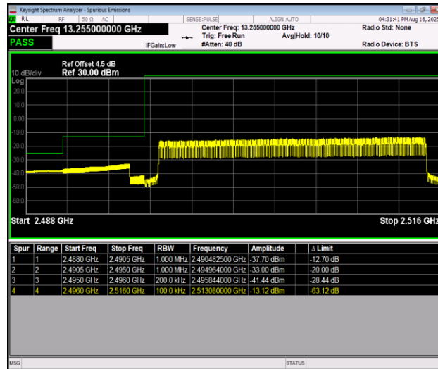
Band41_20MHz_16QAM_39750_100RB#0
