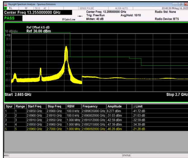
Band41_5MHz_16QAM_41565_1RB#24
