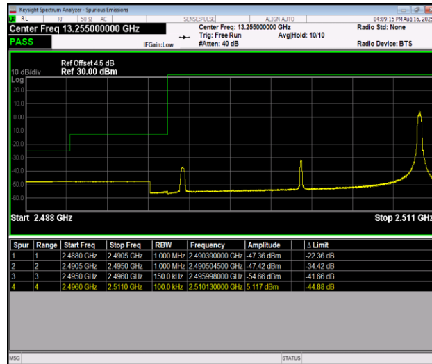
Band41_15MHz_16QAM_39725_1RB#74
