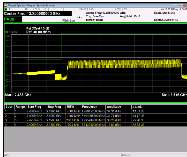
Band41_20MHz_QPSK_39750_100RB#0
