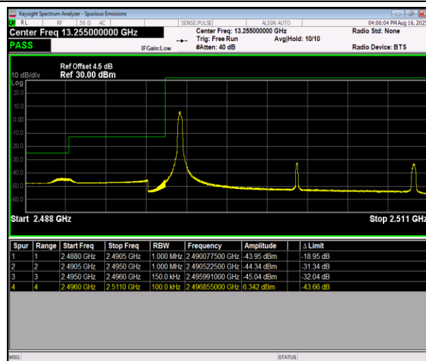
Band41_15MHz_16QAM_39725_1RB#0
