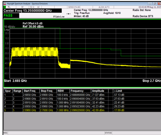
Band41_5MHz_16QAM_41565_25RB#0
