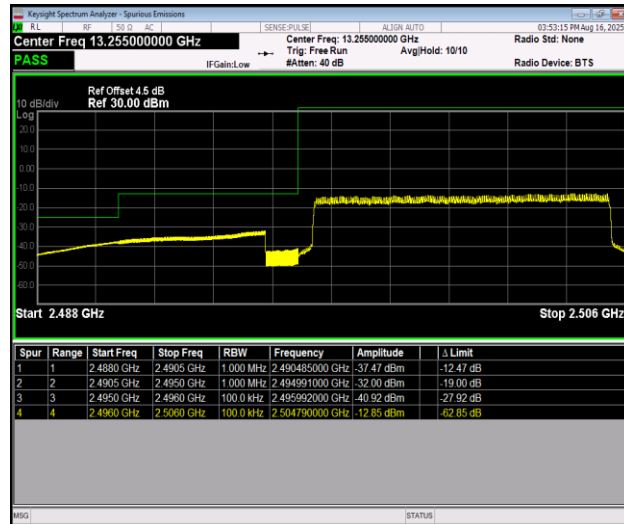
Band41_10MHz_16QAM_39700_50RB#0
