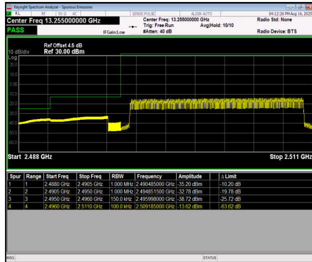
Band41_15MHz_16QAM_39725_75RB#0
