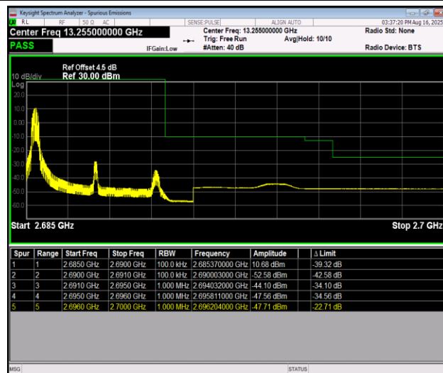
Band41_5MHz_16QAM_41565_1RB#0
