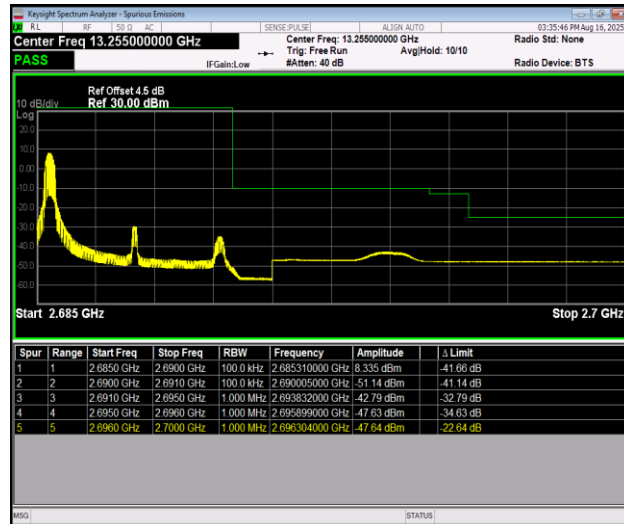
Band41_5MHz_QPSK_41565_1RB#0
