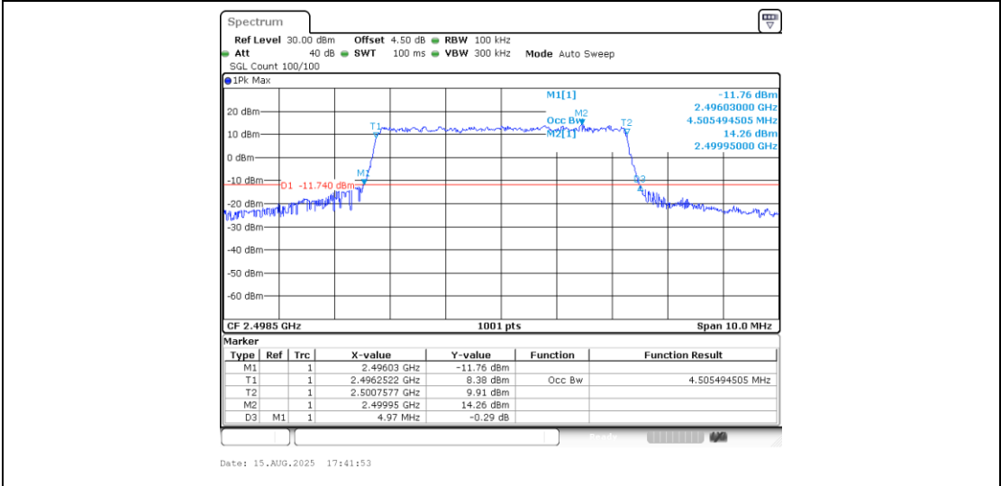
Band41-5MHz-QPSK-39675-25RB#0-PASS
