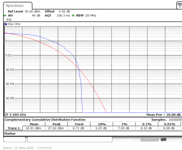
Band41-5MHz-QPSK-40620-1RB#0-PASS
