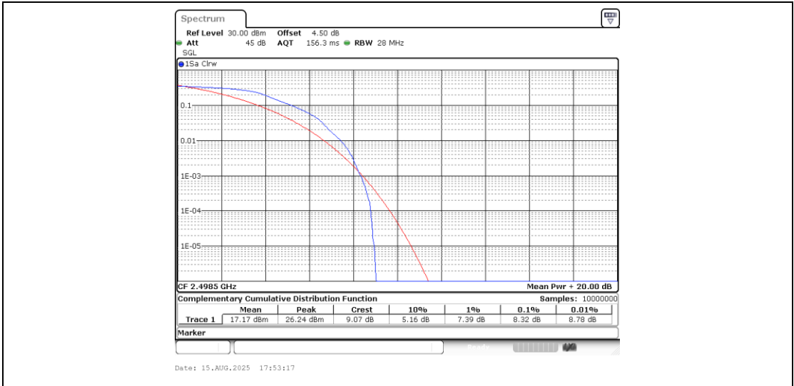
Band41-5MHz-QPSK-39675-1RB#0-PASS
