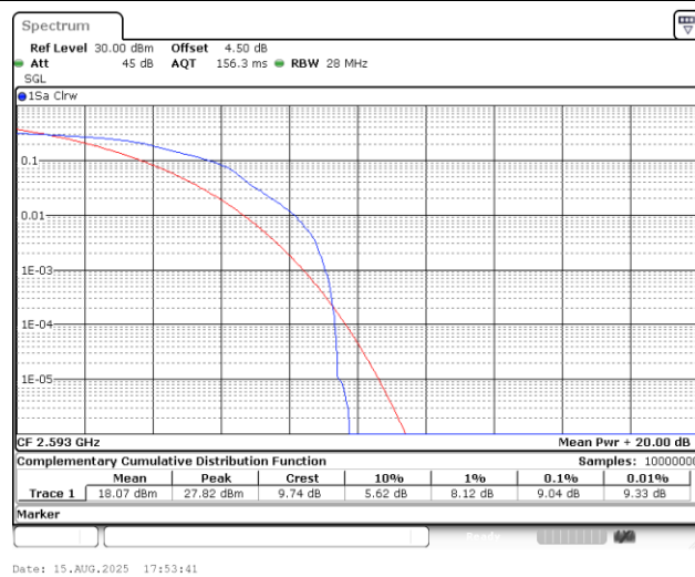
Band41-5MHz-16QAM-40620-1RB#0-PASS
