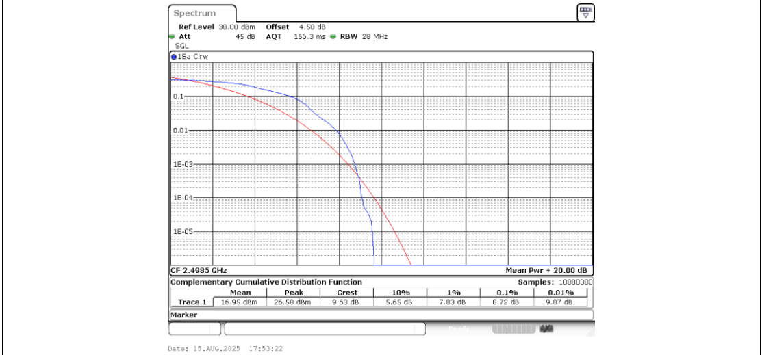
Band41-5MHz-16QAM-39675-1RB#0-PASS
