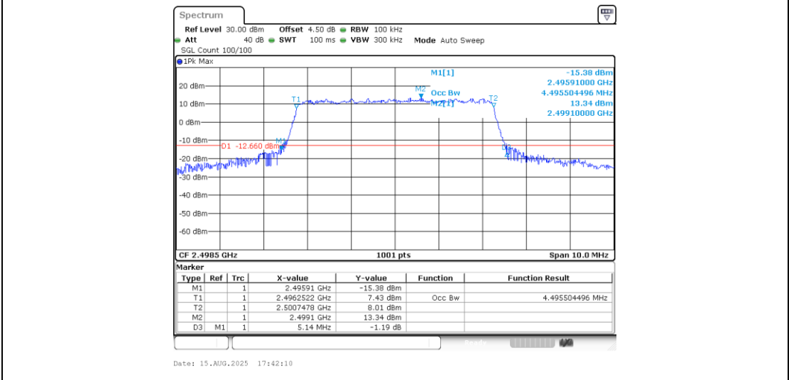
Band41-5MHz-16QAM-39675-25RB#0-PASS
