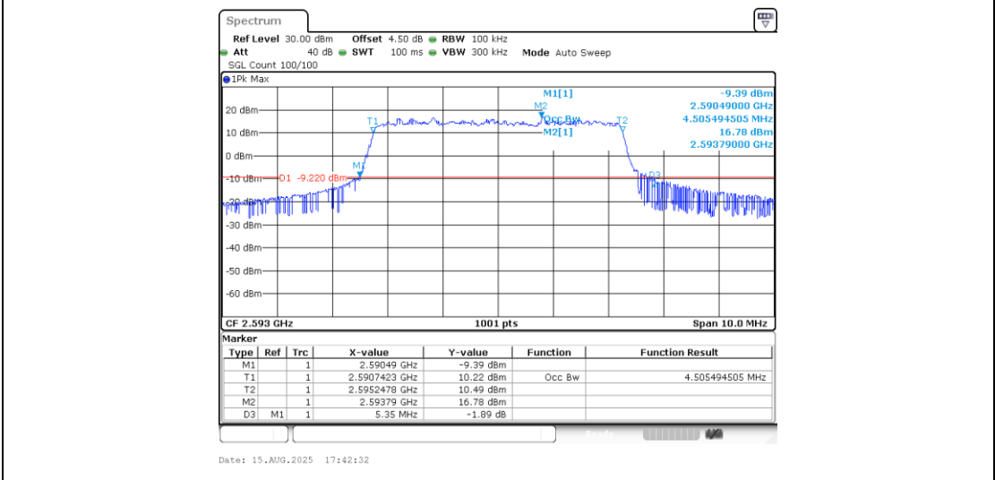
Band41-5MHz-QPSK-40620-25RB#0-PASS
