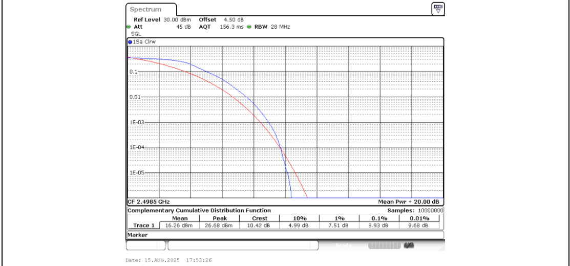
Band41-5MHz-QPSK-39675-25RB#0-PASS
