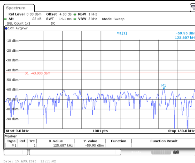
Band25_20MHz_QPSK_26365_1RB#0_0.009~0.15_0.009~0.15
