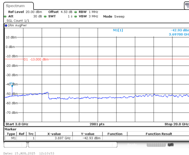
Band25_20MHz_16QAM_26140_1RB#0_3000~20000_3000~20000
