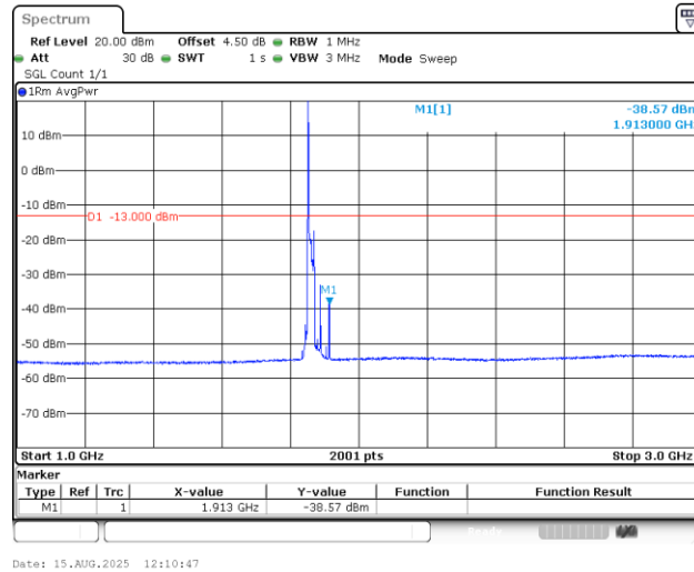
Band25_20MHz_16QAM_26140_1RB#0_1000~3000_1000~3000
