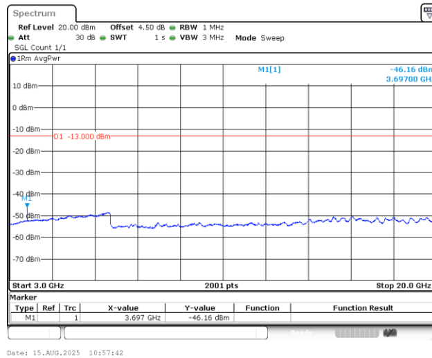
Band25_5MHz_16QAM_26065_1RB#0_3000~20000_3000~20000
