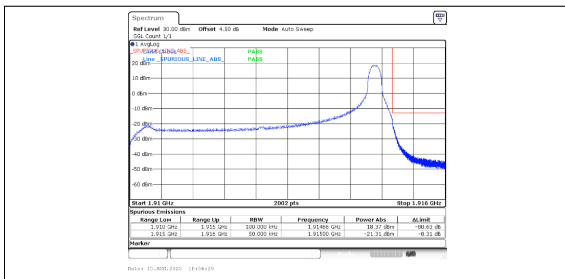
Band25_5MHz_16QAM_26665_1RB#24
