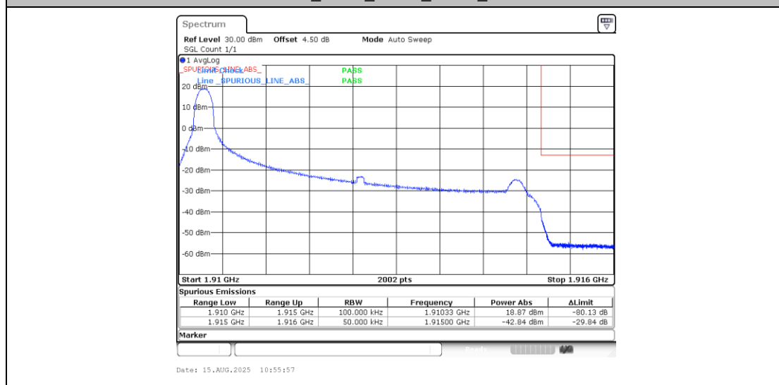
Band25_5MHz_16QAM_26665_1RB#0
