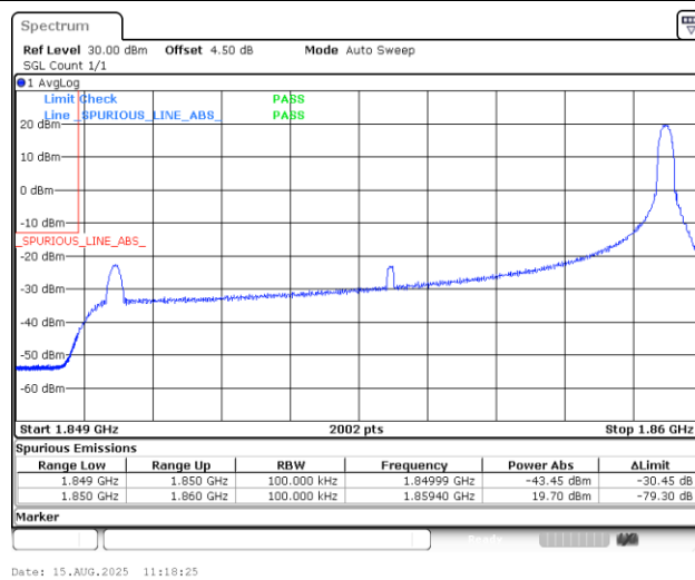
Band25_10MHz_QPSK_26090_1RB#49
