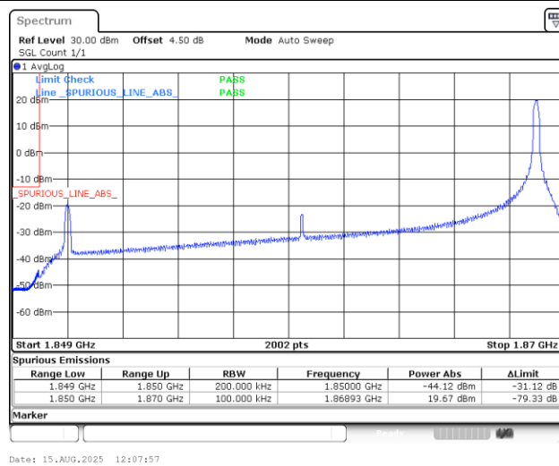
Band25_20MHz_QPSK_26140_1RB#99
