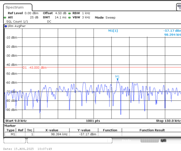
Band25_1.4MHz_QPSK_26365_1RB#0_0.009~0.15_0.009~0.15
