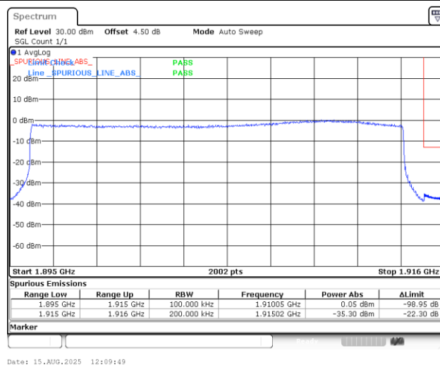
Band25_20MHz_16QAM_26590_100RB#0
