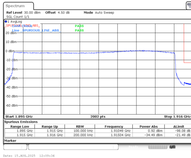
Band25_20MHz_QPSK_26590_100RB#0
