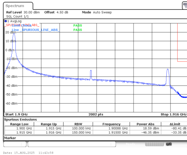
Band25_15MHz_16QAM_26615_1RB#0
