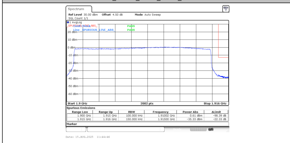
Band25_15MHz_16QAM_26615_75RB#0
