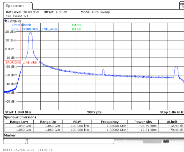
Band25_10MHz_16QAM_26090_1RB#0
