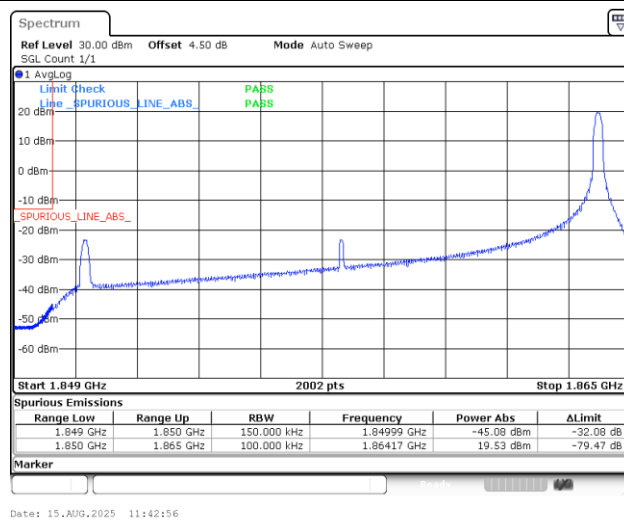
Band25_15MHz_QPSK_26115_1RB#74
