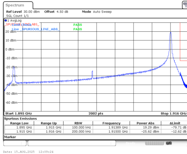
Band25_20MHz_16QAM_26590_1RB#99
