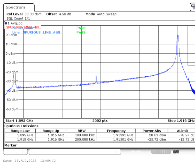
Band25_20MHz_QPSK_26590_1RB#99
