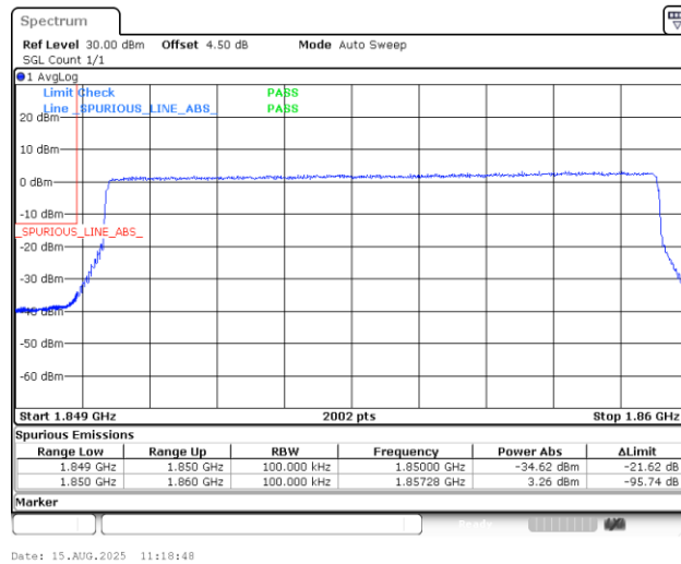
Band25_10MHz_QPSK_26090_50RB#0
