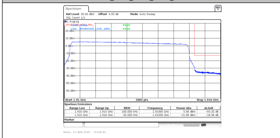
Band25_5MHz_16QAM_26665_25RB#0
