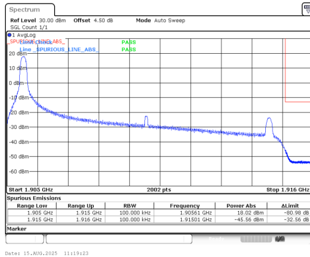
Band25_10MHz_16QAM_26640_1RB#0
