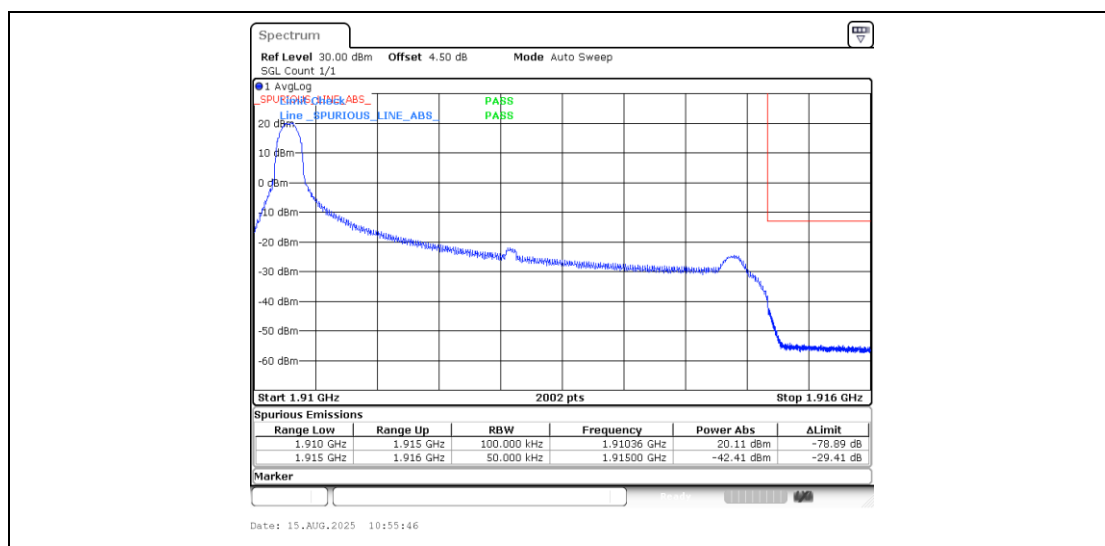
Band25_5MHz_QPSK_26665_1RB#0
