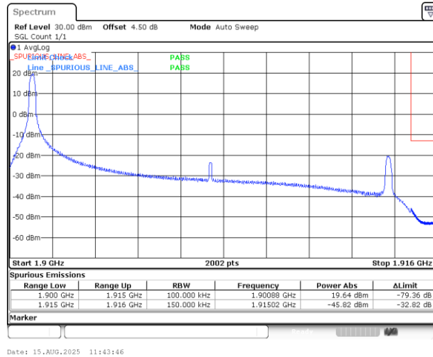
Band25_15MHz_QPSK_26615_1RB#0
