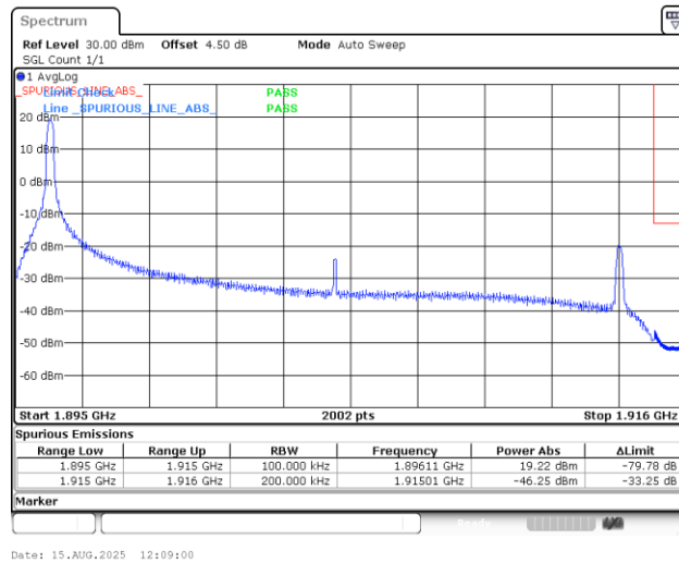
Band25_20MHz_16QAM_26590_1RB#0
