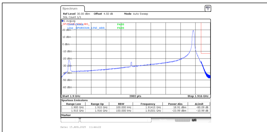
Band25_15MHz_16QAM_26615_1RB#74
