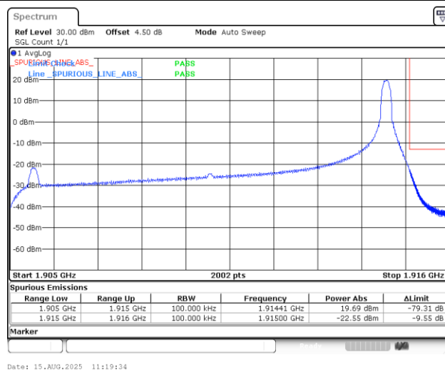
Band25_10MHz_QPSK_26640_1RB#49
