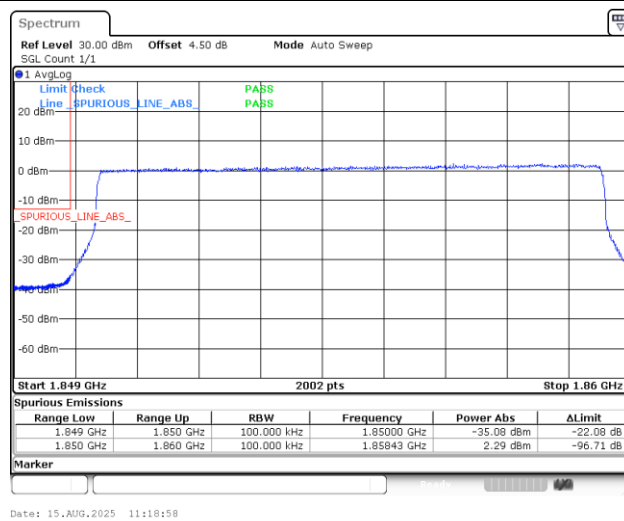
Band25_10MHz_16QAM_26090_50RB#0
