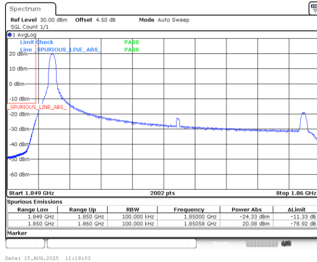
Band25_10MHz_QPSK_26090_1RB#0
