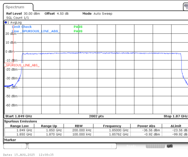
Band25_20MHz_16QAM_26140_100RB#0
