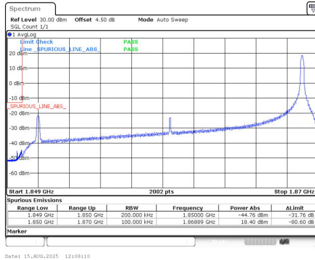
Band25_20MHz_16QAM_26140_1RB#99
