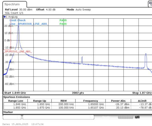
Band25_20MHz_QPSK_26140_1RB#0
