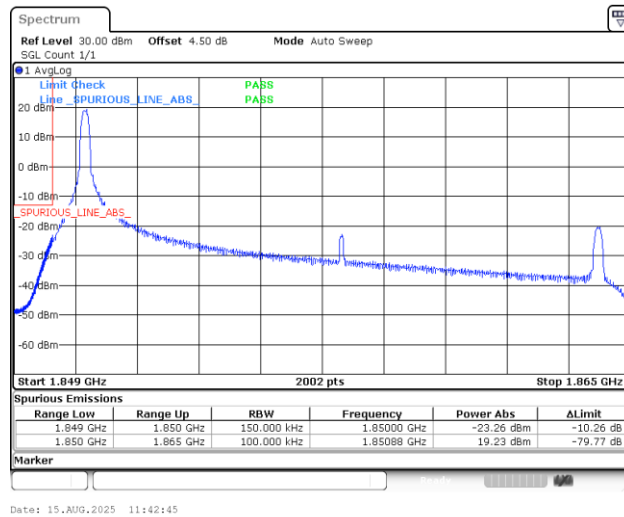
Band25_15MHz_16QAM_26115_1RB#0
