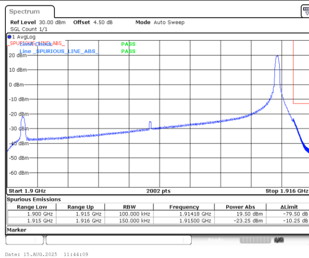
Band25_15MHz_QPSK_26615_1RB#74
