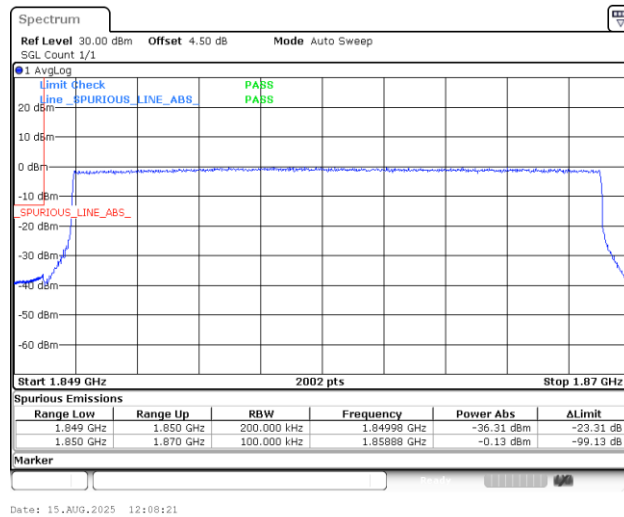
Band25_20MHz_QPSK_26140_100RB#0
