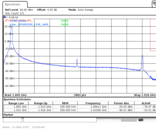
Band25_20MHz_QPSK_26590_1RB#0
