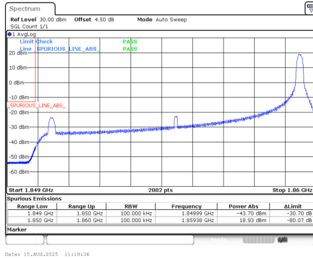
Band25_10MHz_16QAM_26090_1RB#49
