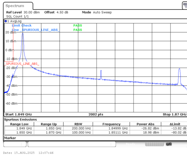
Band25_20MHz_16QAM_26140_1RB#0
