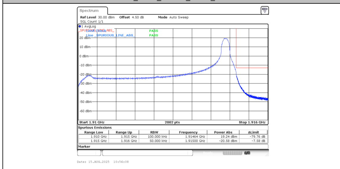
Band25_5MHz_QPSK_26665_1RB#24
