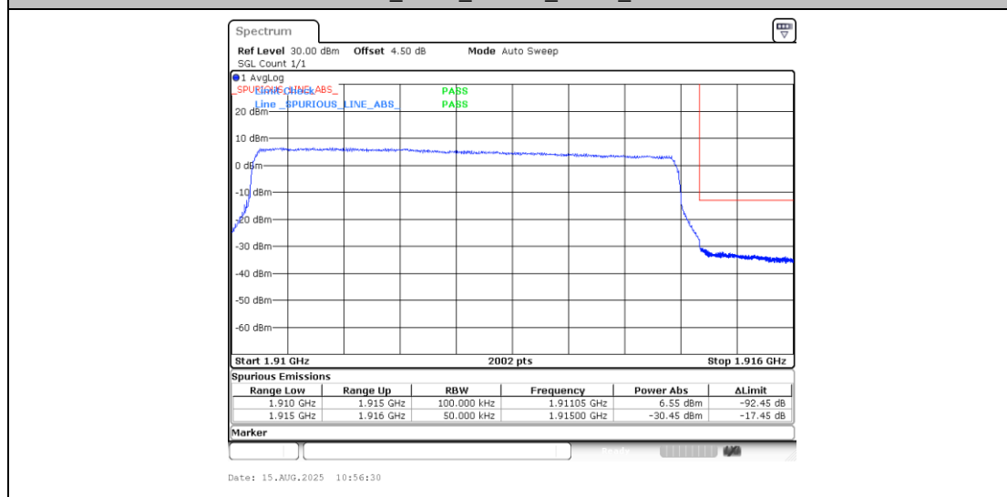
Band25_5MHz_QPSK_26665_25RB#0
