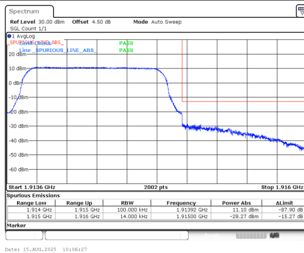
Band25_1.4MHz_16QAM_26683_6RB#0
