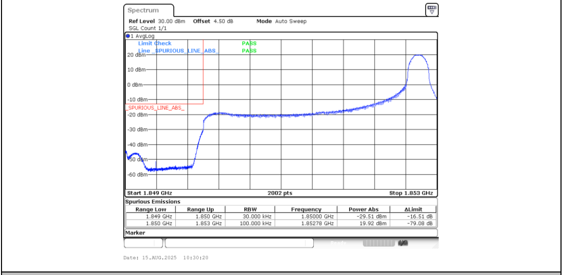
Band25_3MHz_QPSK_26055_1RB#14
