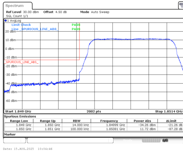
Band25_1.4MHz_QPSK_26047_6RB#0
