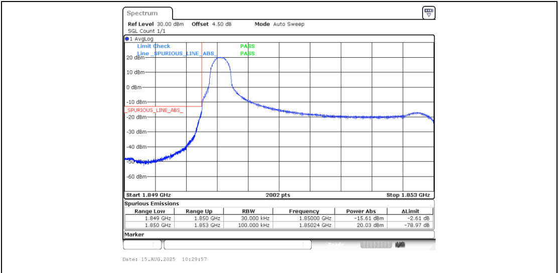
Band25_3MHz_QPSK_26055_1RB#0
