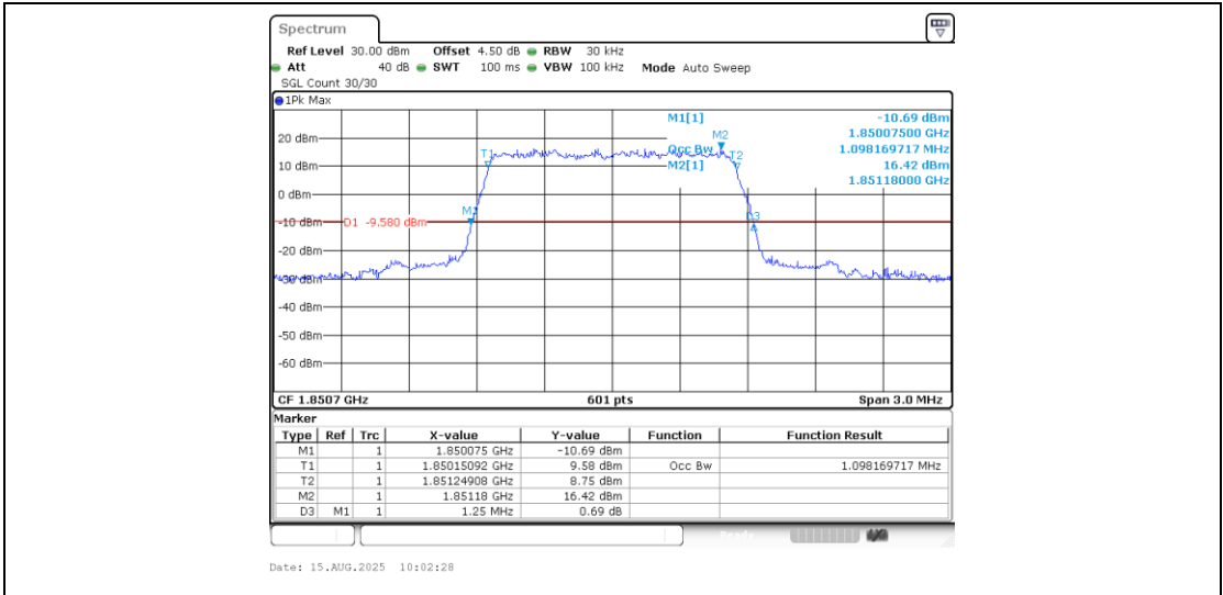
Band25-1.4MHz-QPSK-26047-6RB#0-PASS
