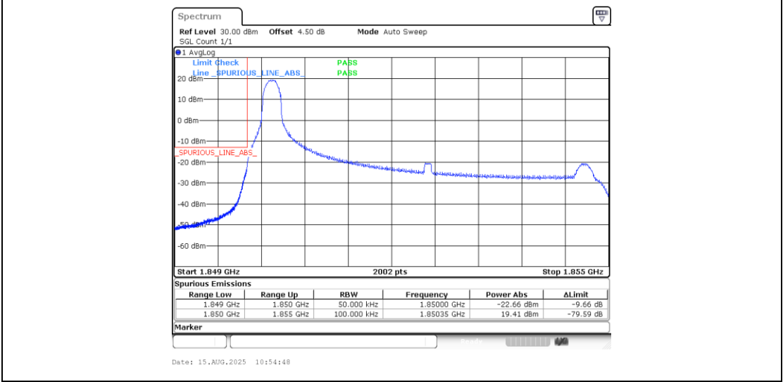
Band25_5MHz_16QAM_26065_1RB#0
