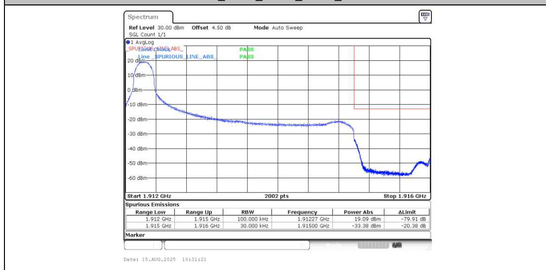
Band25_3MHz_16QAM_26675_1RB#0
