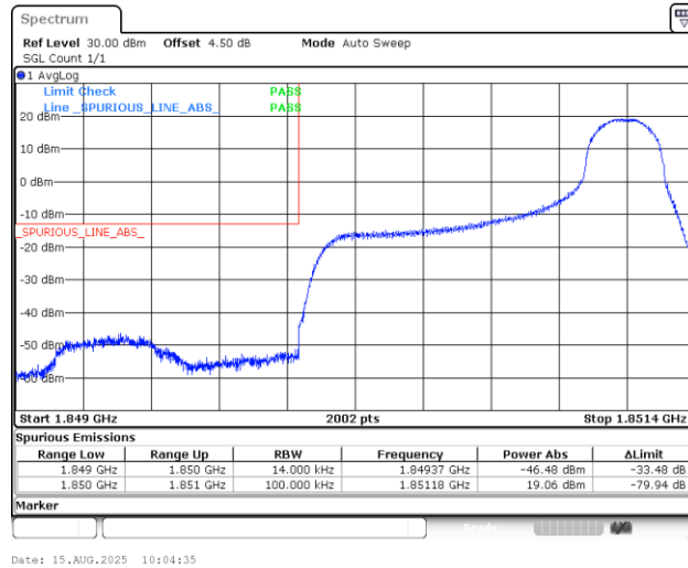
Band25_1.4MHz_16QAM_26047_1RB#5
