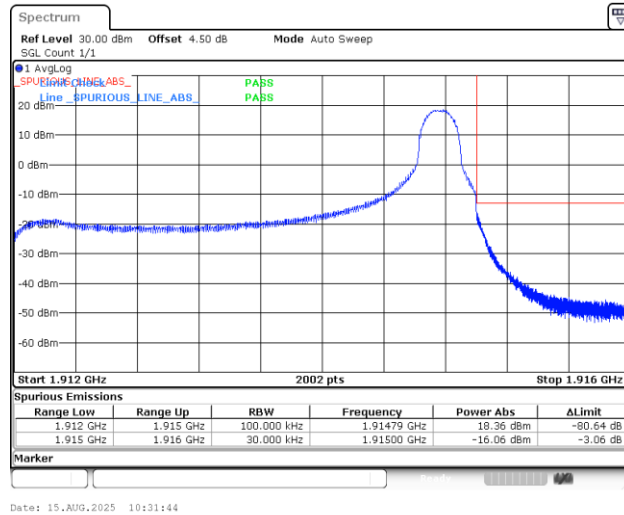
Band25_3MHz_16QAM_26675_1RB#14
