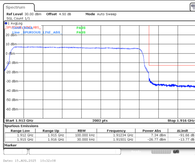
Band25_3MHz_16QAM_26675_15RB#0
