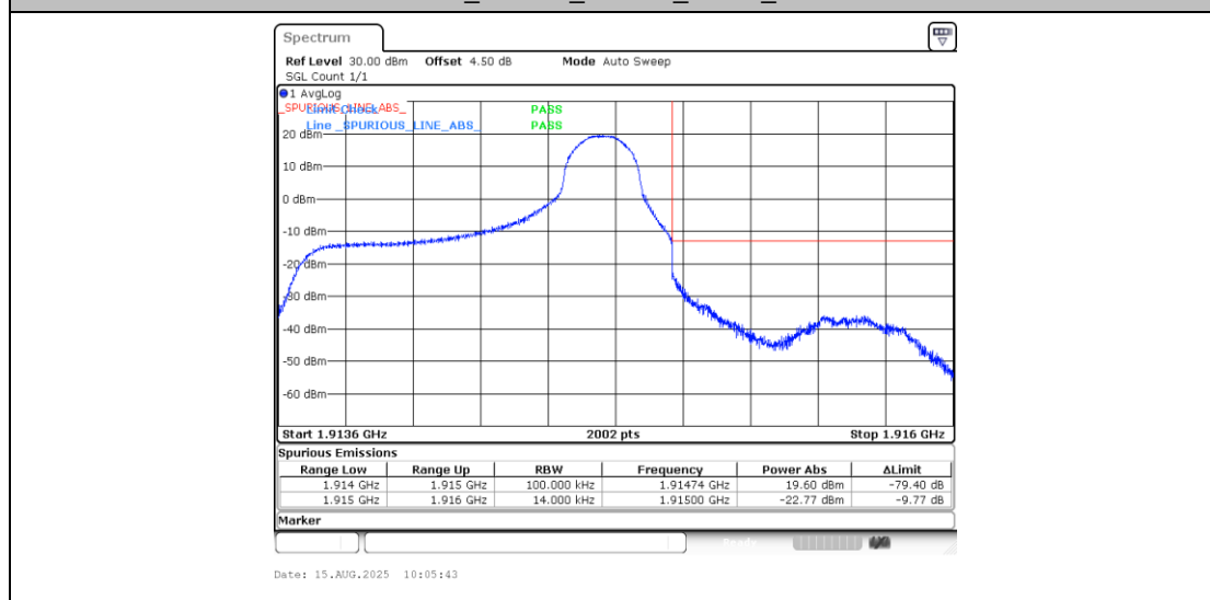
Band25_1.4MHz_QPSK_26683_1RB#5
