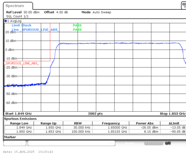
Band25_3MHz_QPSK_26055_15RB#0
