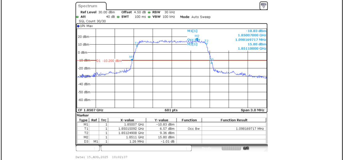
Band25-1.4MHz-16QAM-26047-6RB#0-PASS
