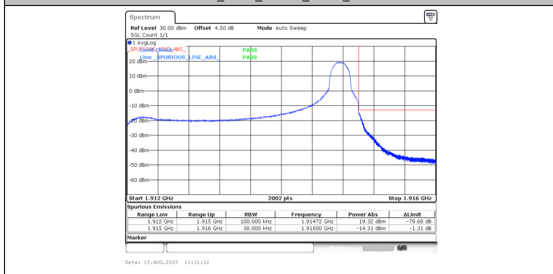
Band25_3MHz_QPSK_26675_1RB#14
