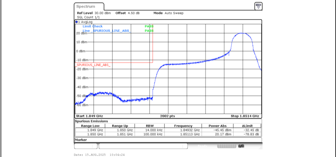
Band25_1.4MHz_QPSK_26047_1RB#5
