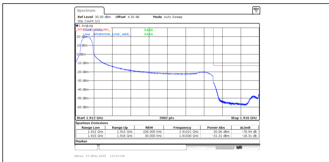
Band25_3MHz_QPSK_26675_1RB#0
