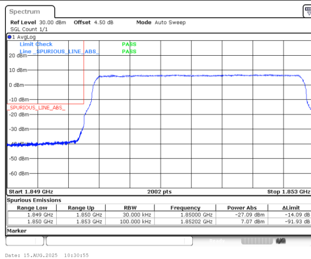
Band25_3MHz_16QAM_26055_15RB#0
