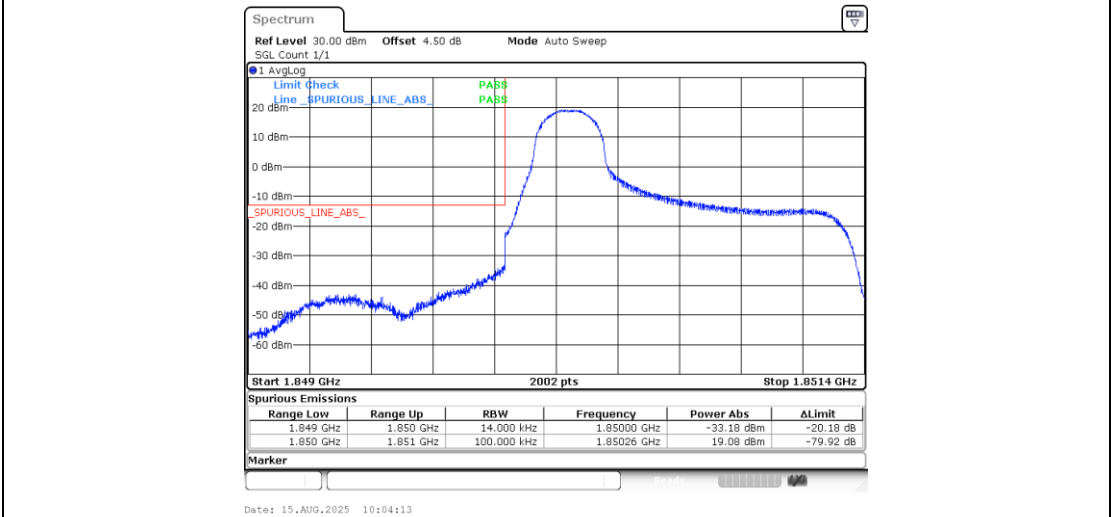
Band25_1.4MHz_16QAM_26047_1RB#0
