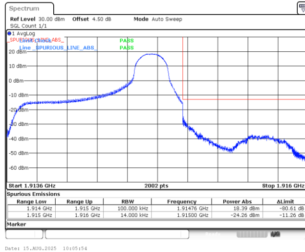
Band25_1.4MHz_16QAM_26683_1RB#5
