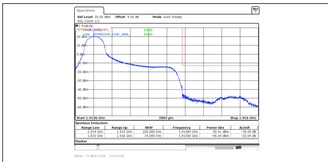
Band25_1.4MHz_QPSK_26683_1RB#0
