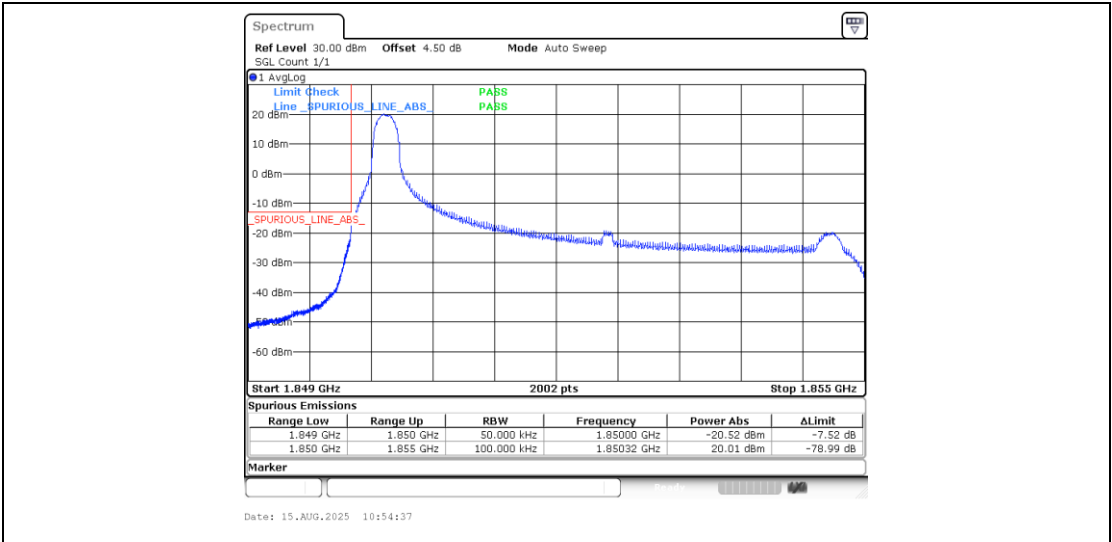
Band25_5MHz_QPSK_26065_1RB#0
