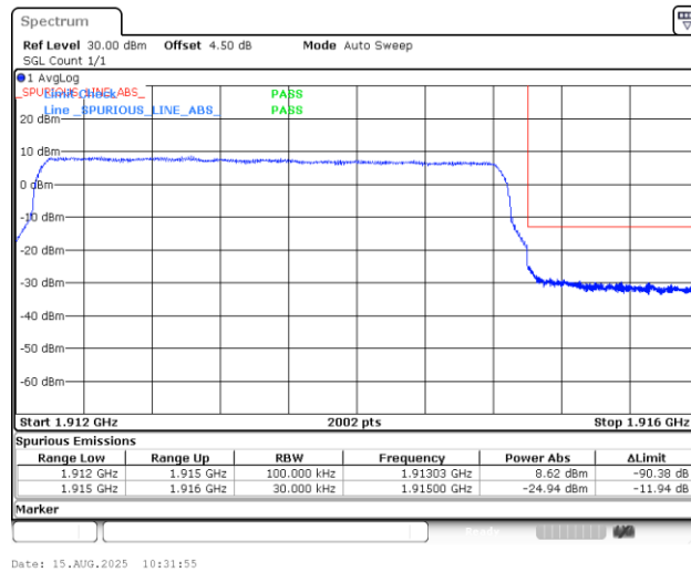
Band25_3MHz_QPSK_26675_15RB#0
