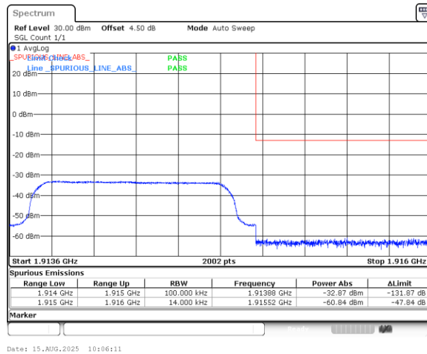
Band25_1.4MHz_QPSK_26683_6RB#0
