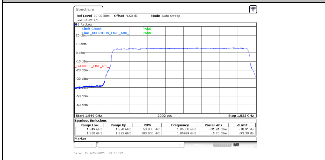
Band25_5MHz_QPSK_26065_25RB#0
