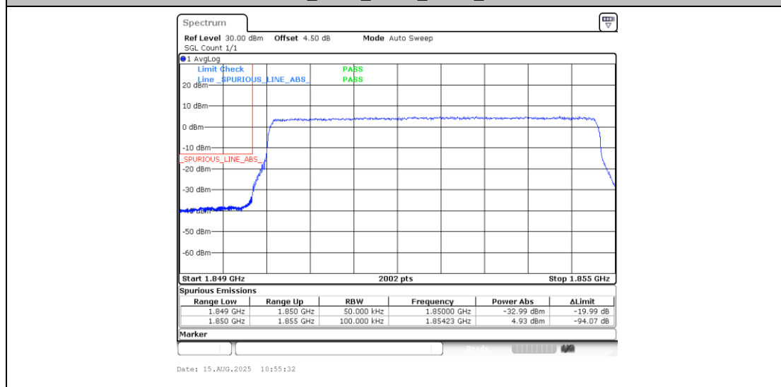
Band25_5MHz_16QAM_26065_25RB#0
