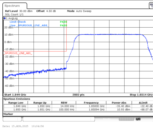
Band25_1.4MHz_16QAM_26047_6RB#0
