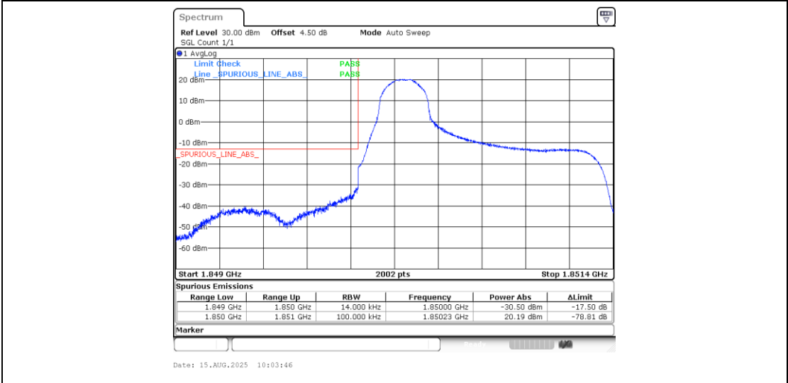
Band25_1.4MHz_QPSK_26047_1RB#0
