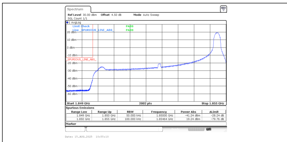
Band25_5MHz_16QAM_26065_1RB#24
