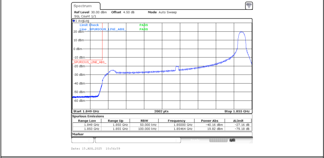
Band25_5MHz_QPSK_26065_1RB#24
