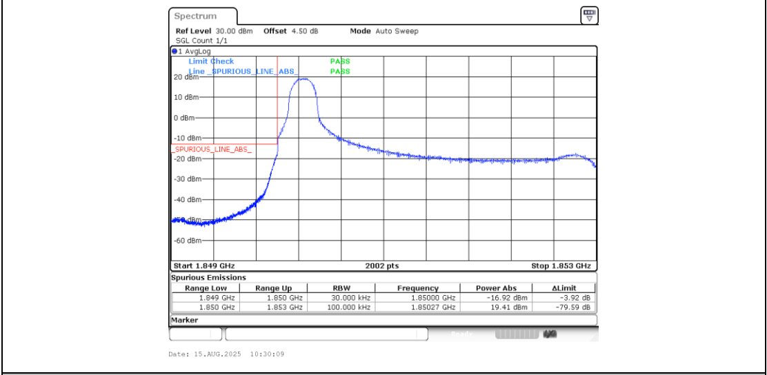
Band25_3MHz_16QAM_26055_1RB#0
