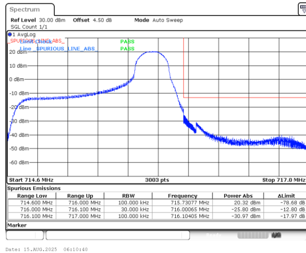
Band12_1.4MHz_16QAM_23173_1RB#5
