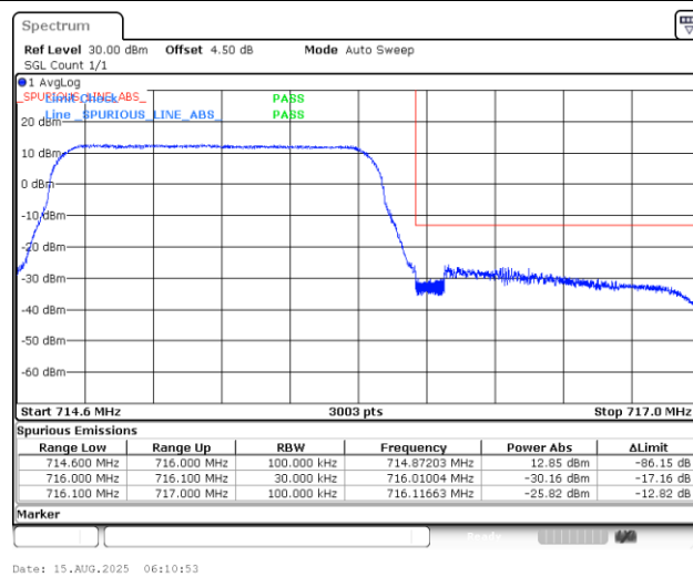
Band12_1.4MHz_QPSK_23173_6RB#0
