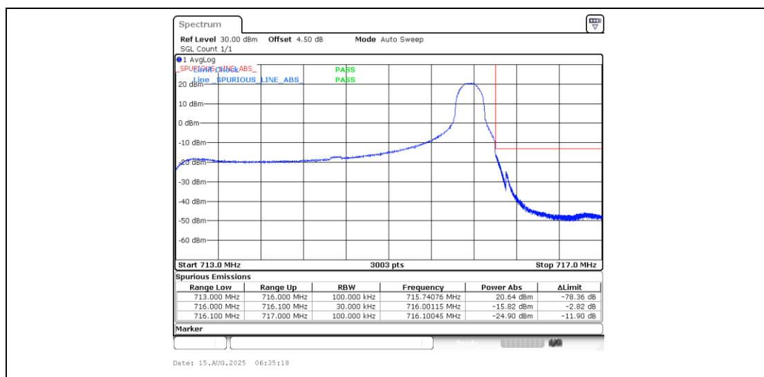
Band12_3MHz_QPSK_23165_1RB#14
