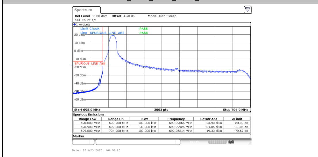
Band12_5MHz_16QAM_23035_1RB#0
