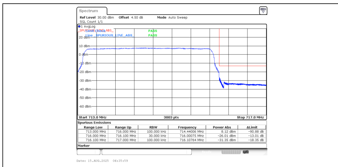
Band12_3MHz_16QAM_23165_15RB#0
