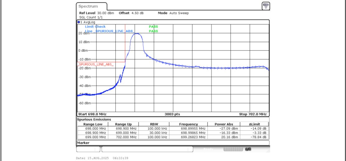
Band12_3MHz_16QAM_23025_1RB#0
