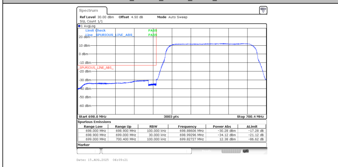
Band12_1.4MHz_QPSK_23017_6RB#0
