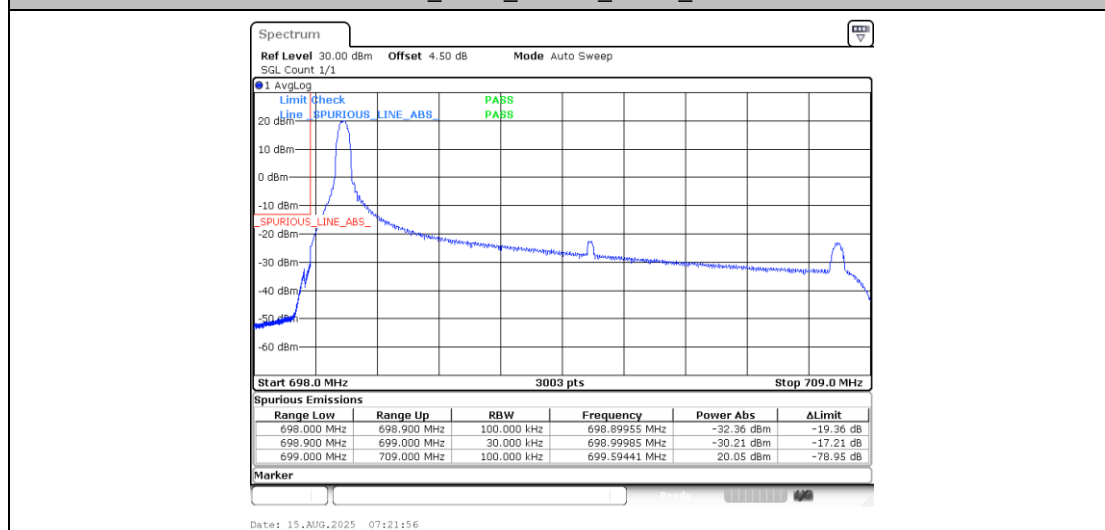
Band12_10MHz_QPSK_23060_1RB#0
