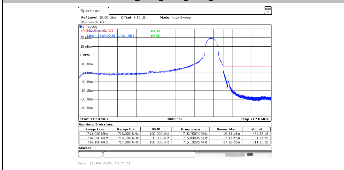
Band12_3MHz_16QAM_23165_1RB#14
