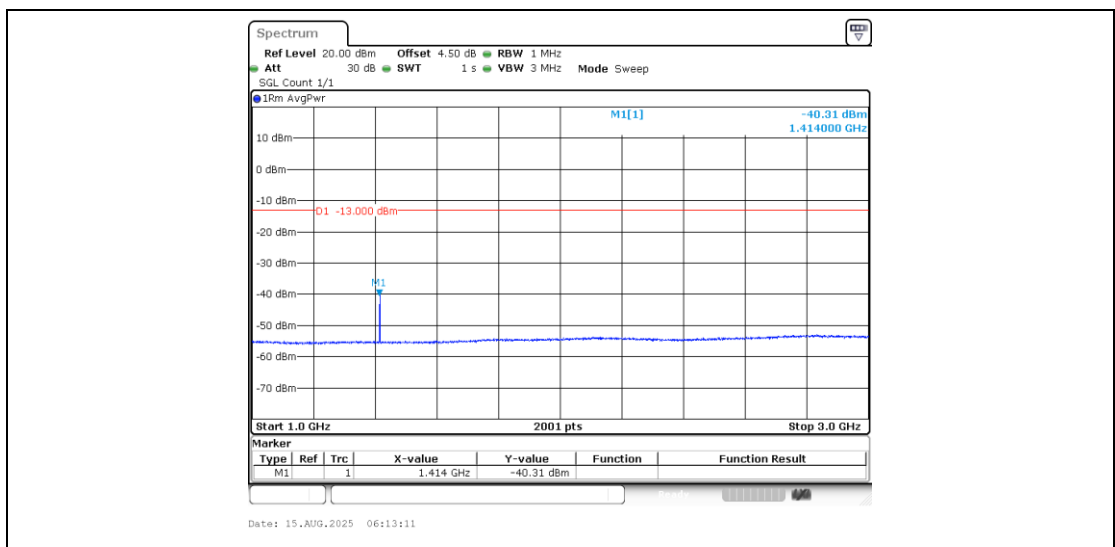
Band12_1.4MHz_16QAM_23095_1RB#0_1000~3000_1000~3000
