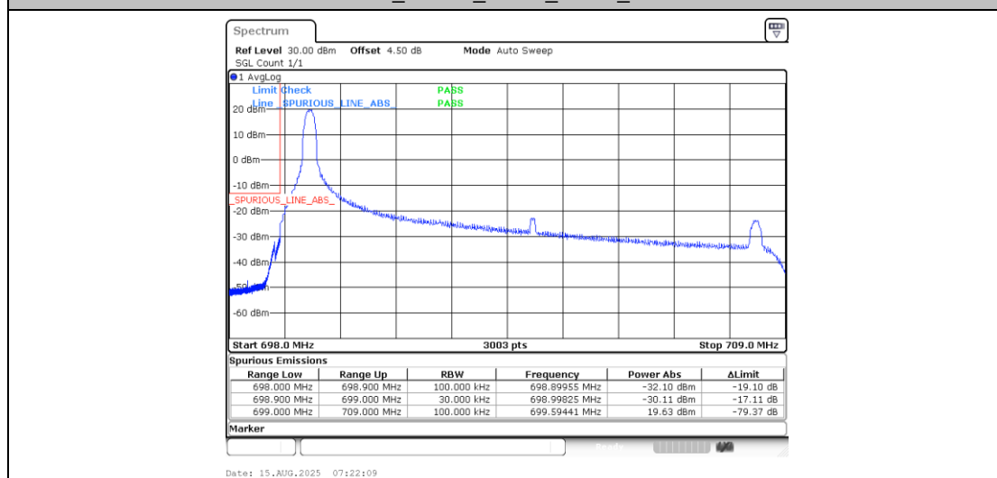
Band12_10MHz_16QAM_23060_1RB#0
