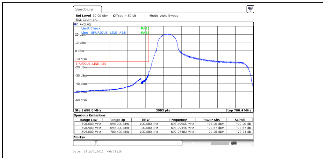
Band12_1.4MHz_QPSK_23017_1RB#0
