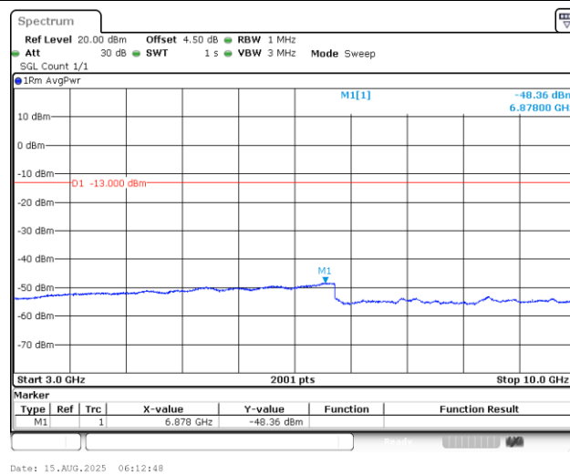
Band12_1.4MHz_QPSK_23095_1RB#0_3000~10000_3000~10000
