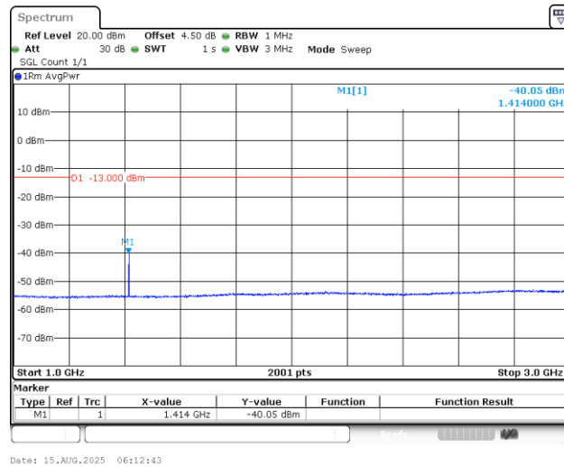
Band12_1.4MHz_QPSK_23095_1RB#0_1000~3000_1000~3000
