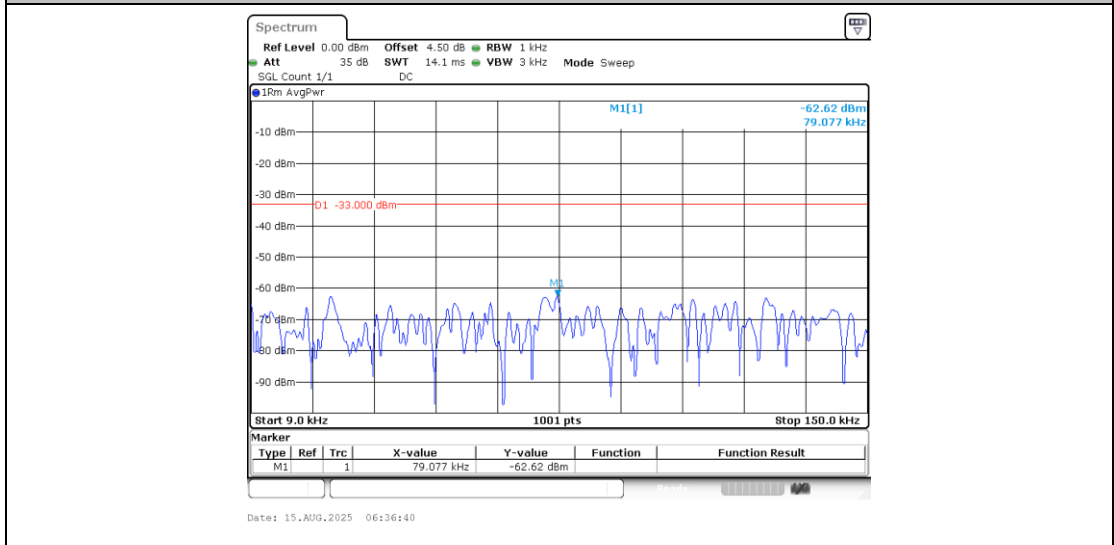
Band12_3MHz_16QAM_23025_1RB#0_0.009~0.15_0.009~0.15
