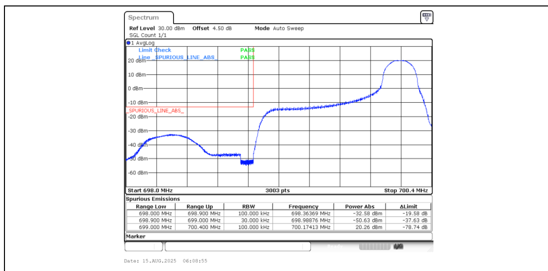
Band12_1.4MHz_QPSK_23017_1RB#5
