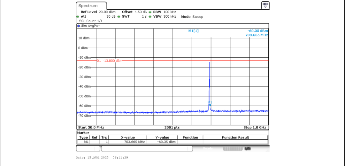
Band12_1.4MHz_QPSK_23017_1RB#0_30~1000_30~1000
