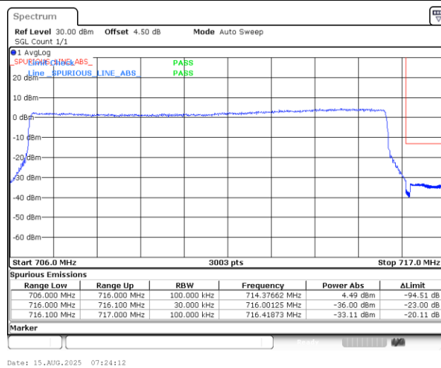
Band12_10MHz_QPSK_23130_50RB#0
