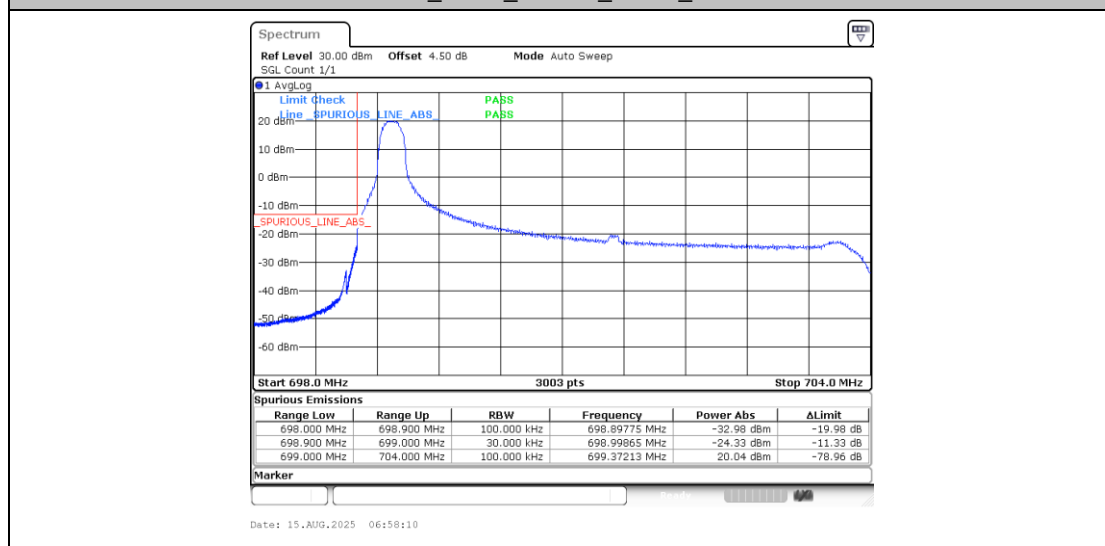
Band12_5MHz_QPSK_23035_1RB#0
