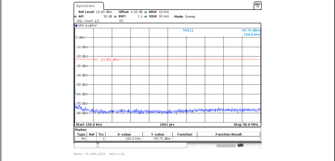
Band12_1.4MHz_QPSK_23017_1RB#0_0.15~30_0.15~30
