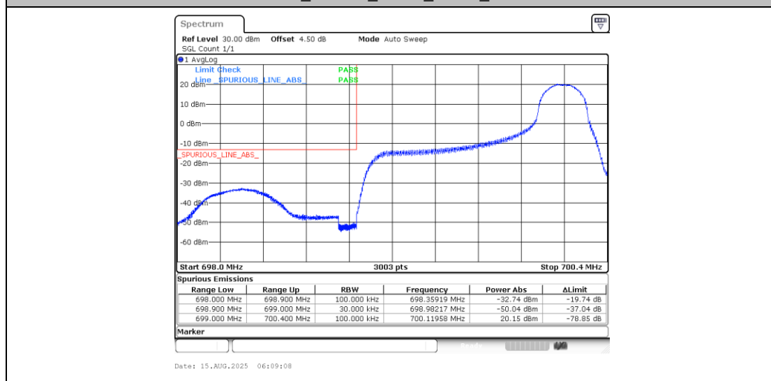
Band12_1.4MHz_16QAM_23017_1RB#5
