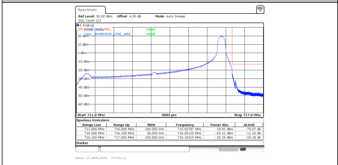
Band12_5MHz_16QAM_23155_1RB#24
