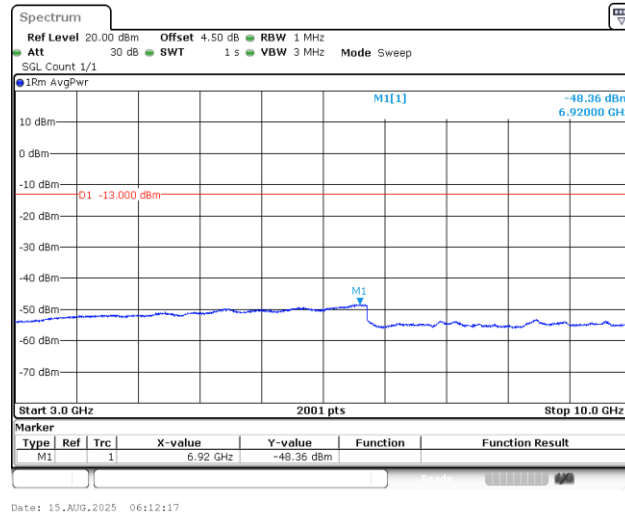
Band12_1.4MHz_16QAM_23017_1RB#0_3000~10000_3000~10000
