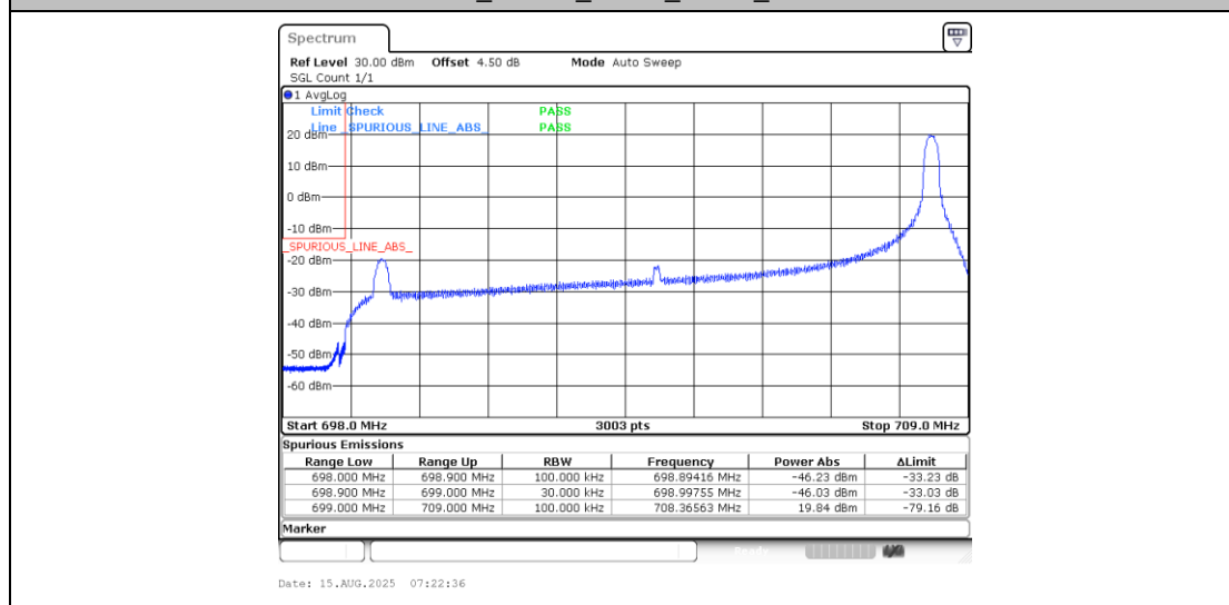
Band12_10MHz_16QAM_23060_1RB#49
