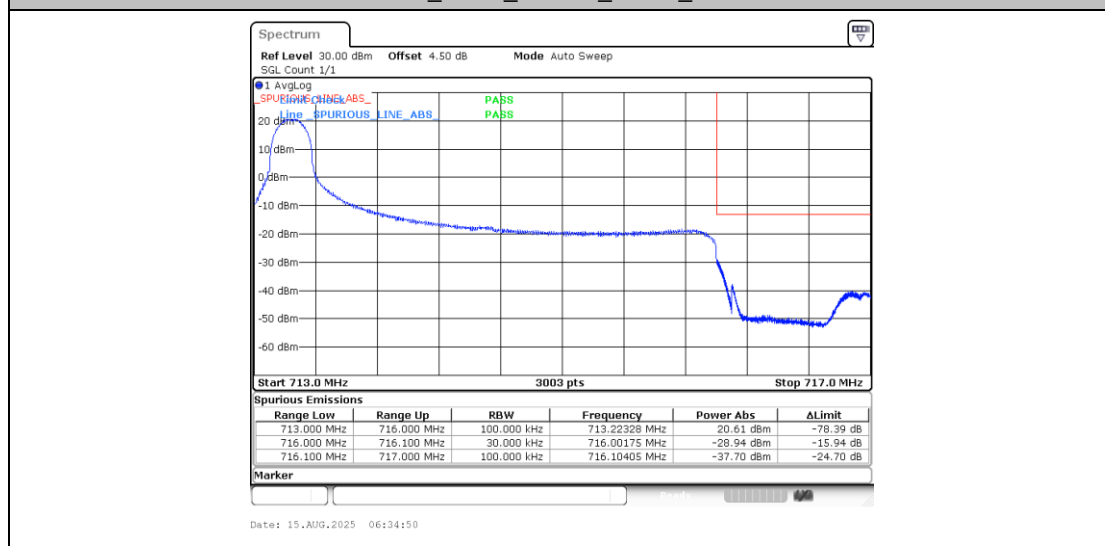
Band12_3MHz_QPSK_23165_1RB#0
