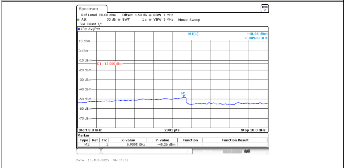
Band12_3MHz_QPSK_23025_1RB#0_3000~10000_3000~10000
