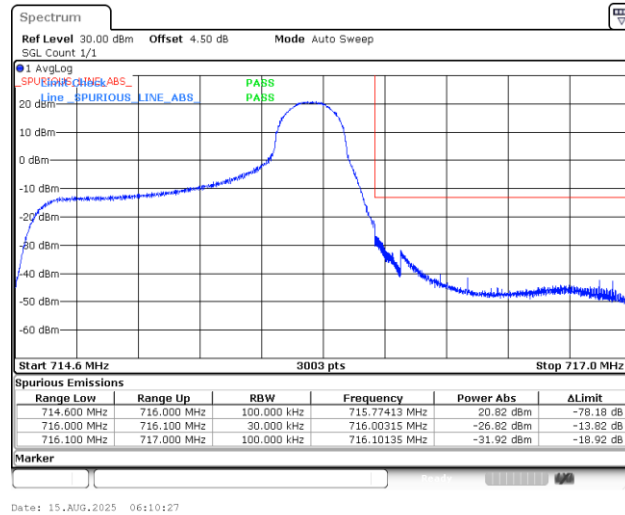
Band12_1.4MHz_QPSK_23173_1RB#5
