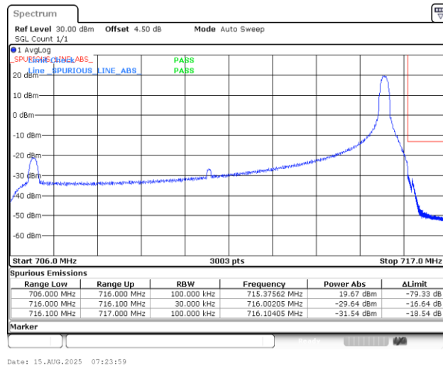
Band12_10MHz_16QAM_23130_1RB#49
