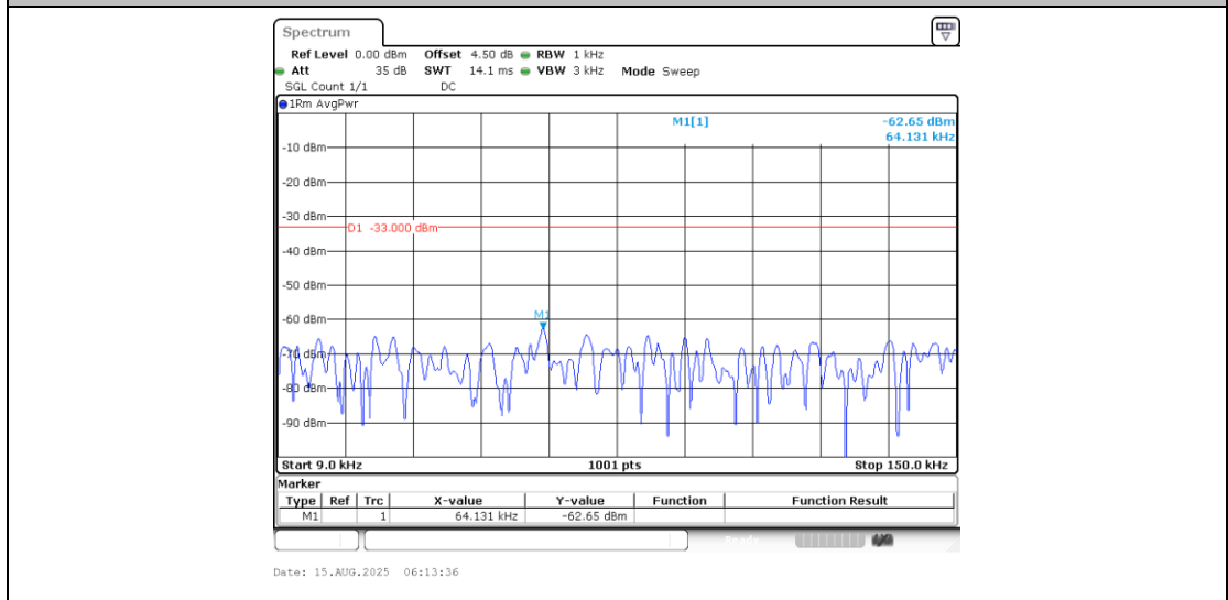
Band12_1.4MHz_QPSK_23173_1RB#0_0.009~0.15_0.009~0.15
