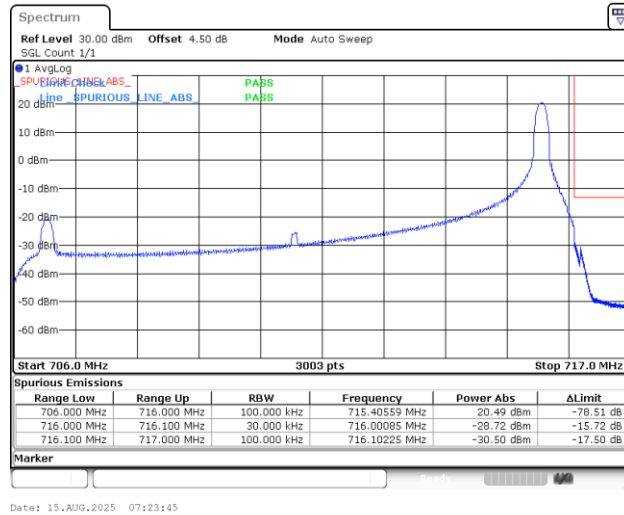
Band12_10MHz_QPSK_23130_1RB#49
