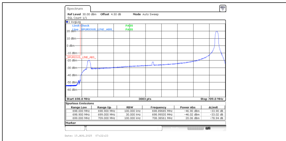
Band12_10MHz_QPSK_23060_1RB#49
