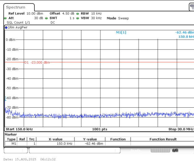
Band12_1.4MHz_QPSK_23095_1RB#0_0.15~30_0.15~30
