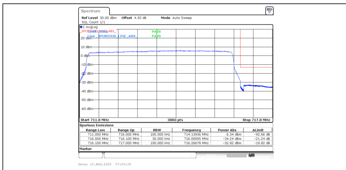
Band12_5MHz_16QAM_23155_25RB#0
