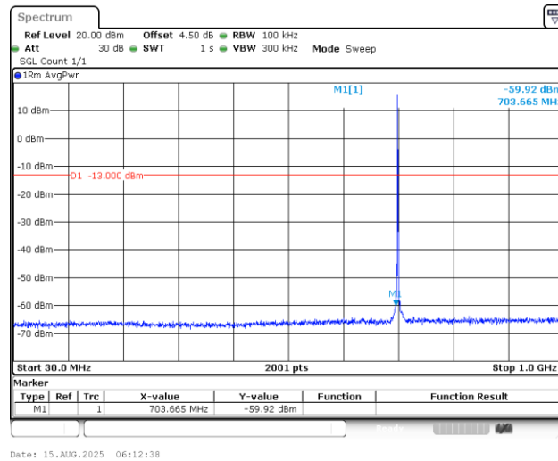
Band12_1.4MHz_QPSK_23095_1RB#0_30~1000_30~1000
