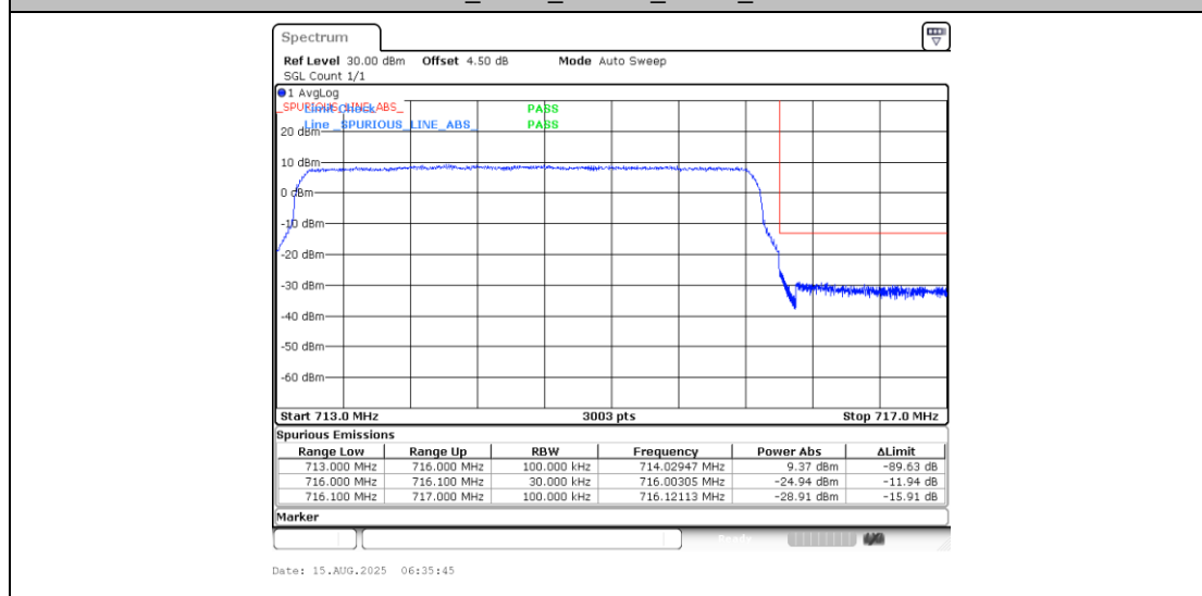
Band12_3MHz_QPSK_23165_15RB#0
