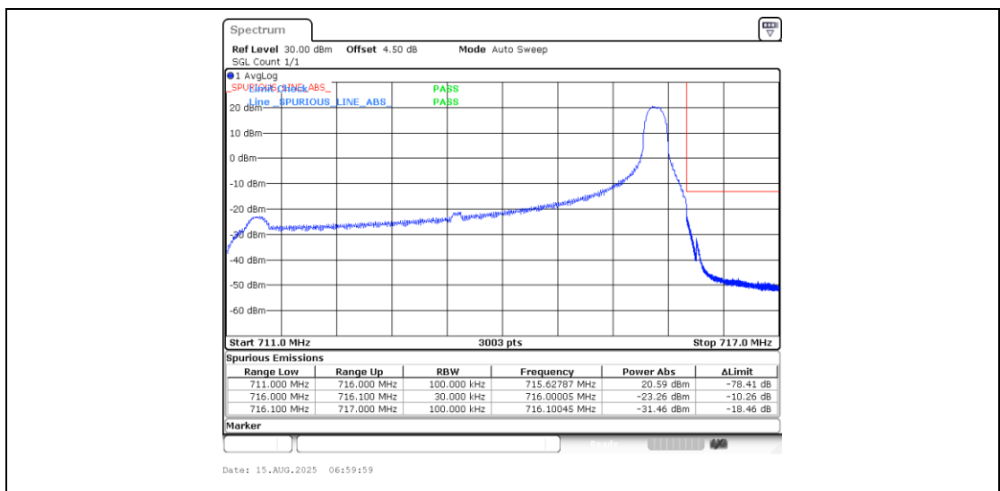
Band12_5MHz_QPSK_23155_1RB#24
