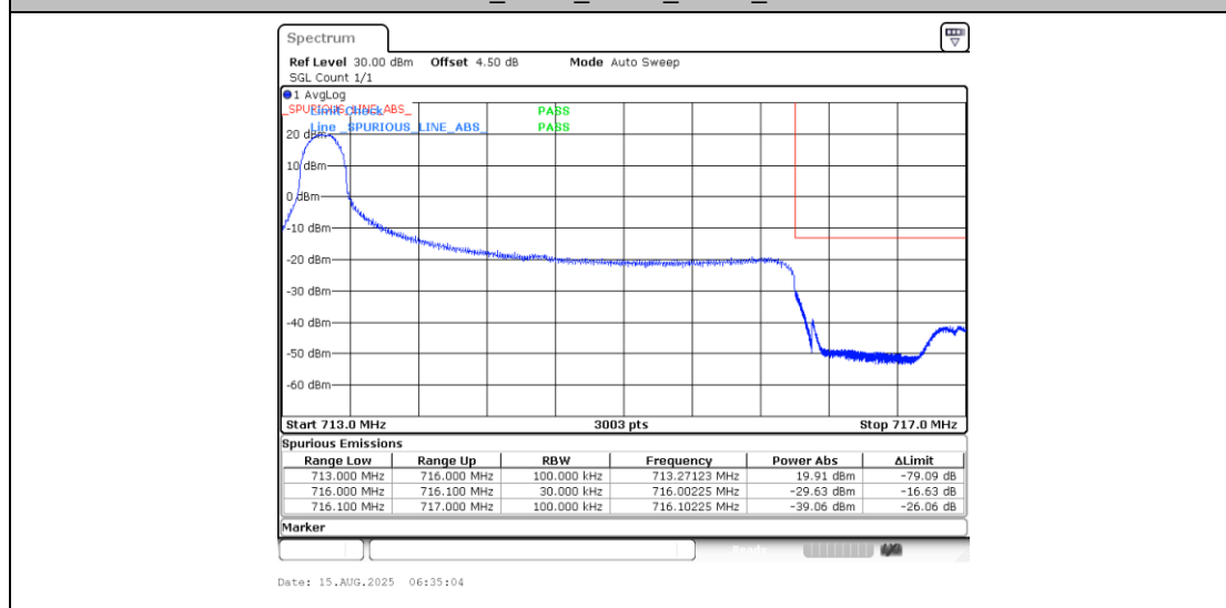
Band12_3MHz_16QAM_23165_1RB#0
