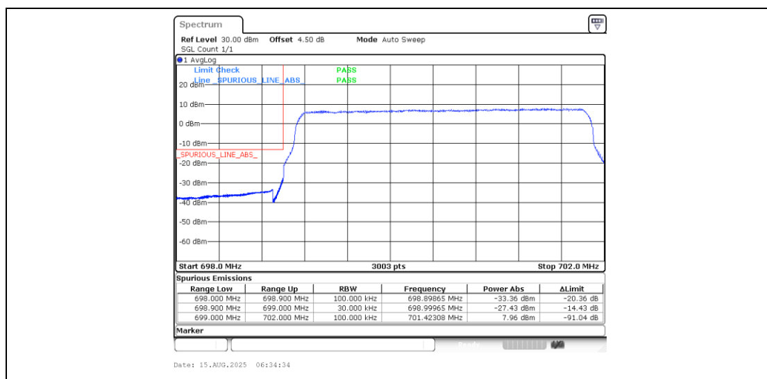
Band12_3MHz_16QAM_23025_15RB#0
