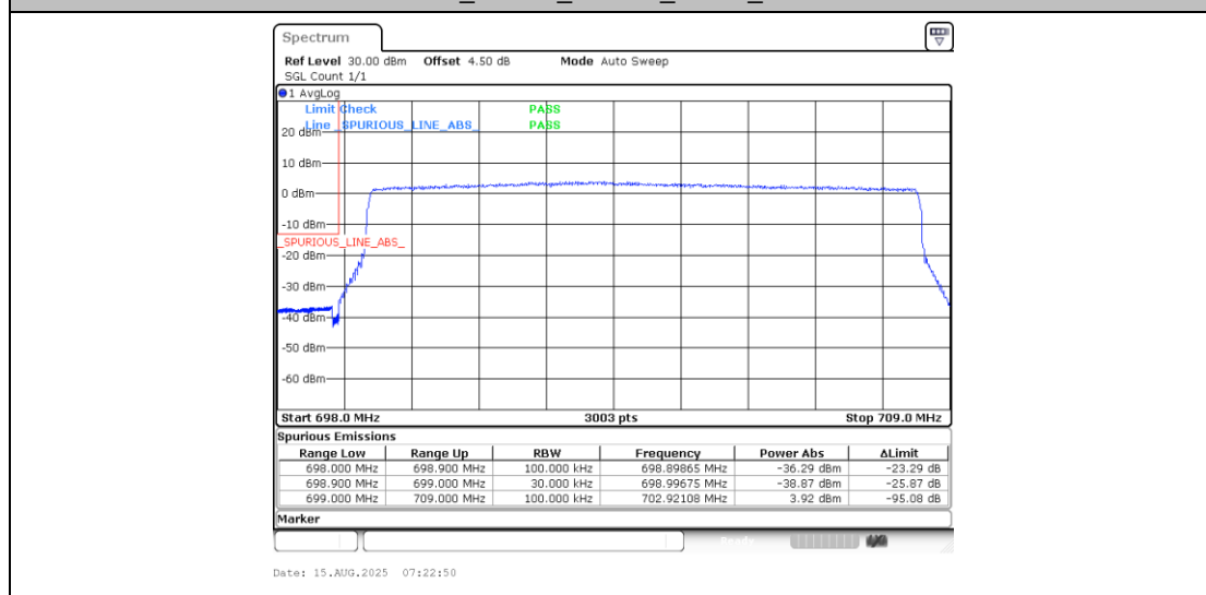
Band12_10MHz_QPSK_23060_50RB#0
