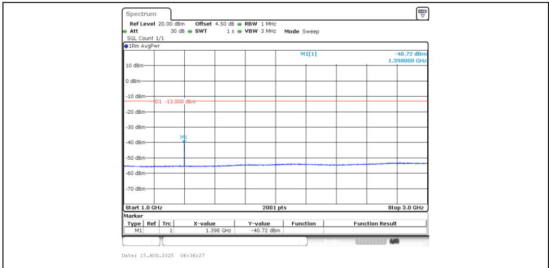
Band12_3MHz_QPSK_23025_1RB#0_1000~3000_1000~3000
