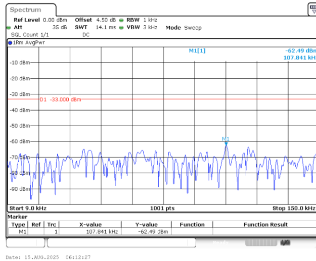
Band12_1.4MHz_QPSK_23095_1RB#0_0.009~0.15_0.009~0.15
