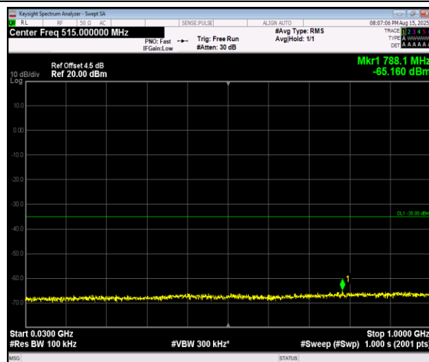
Band7_10MHz_QPSK_20800_1RB#0_30~1000_30~1000
