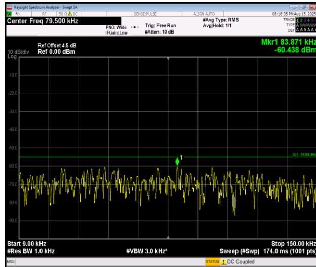
Band7_20MHz_16QAM_21100_1RB#0_0.009~0.15_0.009~0.15
