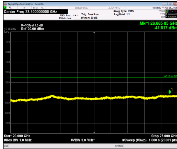
Band7_5MHz_QPSK_21425_1RB#0_20000~27000_20000~27000
