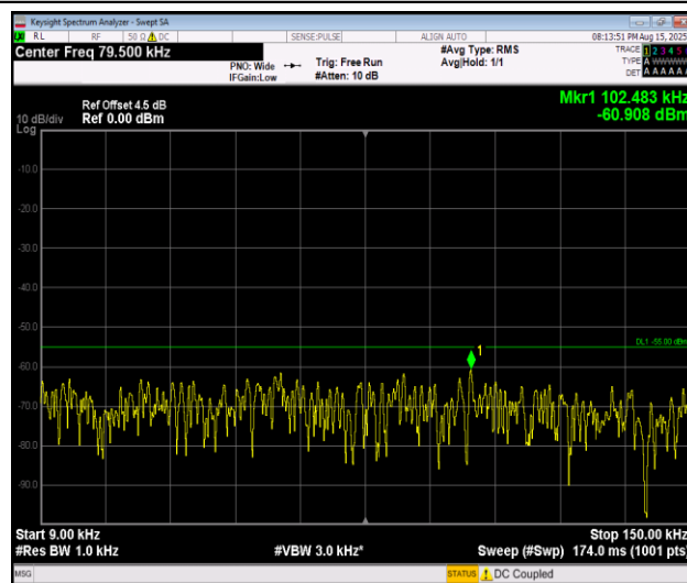
Band7_15MHz_16QAM_21100_1RB#0_0.009~0.15_0.009~0.15
