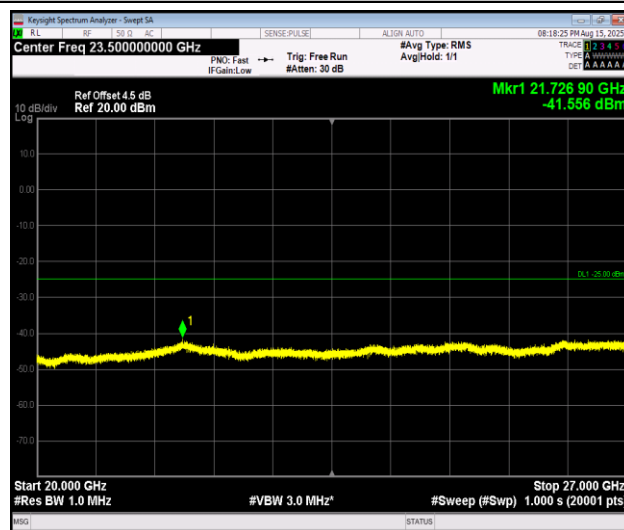
Band7_20MHz_QPSK_21100_1RB#0_20000~27000_20000~27000
