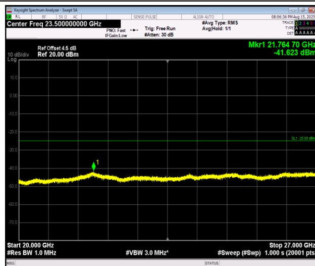
Band7_5MHz_16QAM_21425_1RB#0_20000~27000_20000~27000
