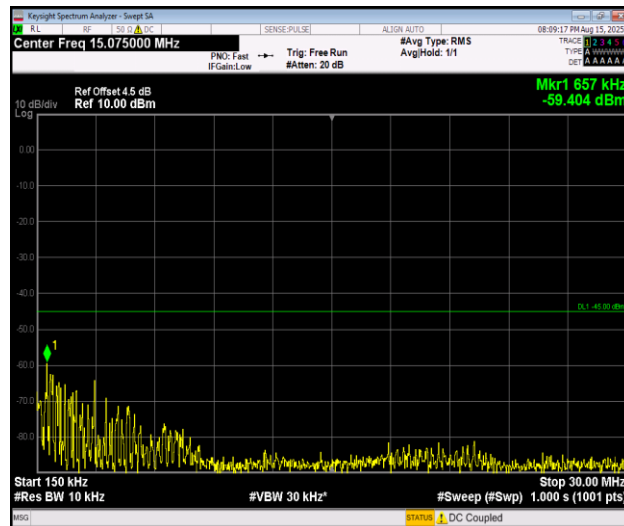
Band7_10MHz_16QAM_21100_1RB#0_0.15~30_0.15~30
