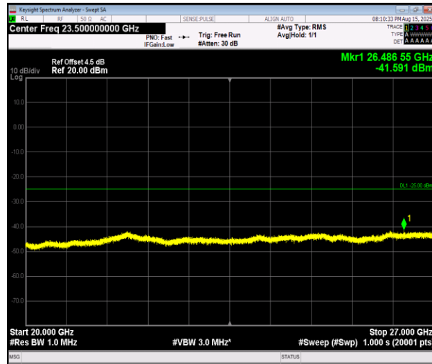
Band7_10MHz_QPSK_21400_1RB#0_20000~27000_20000~27000
