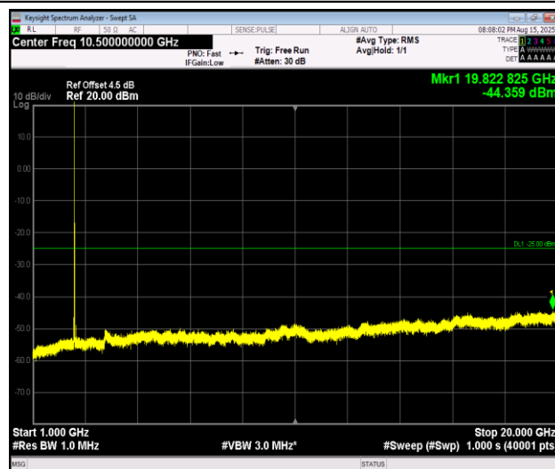
Band7_10MHz_16QAM_20800_1RB#0_1000~20000_1000~20000
