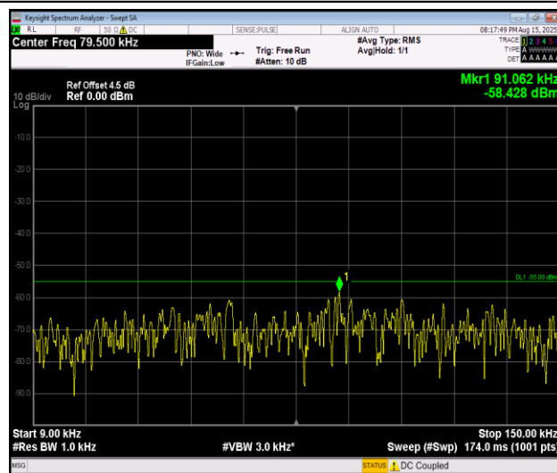
Band7_20MHz_QPSK_21100_1RB#0_0.009~0.15_0.009~0.15
