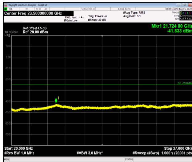
Band7_10MHz_16QAM_21100_1RB#0_20000~27000_20000~27000
