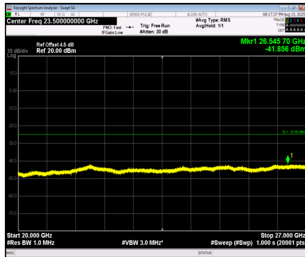
Band7_20MHz_16QAM_20850_1RB#0_20000~27000_20000~27000
