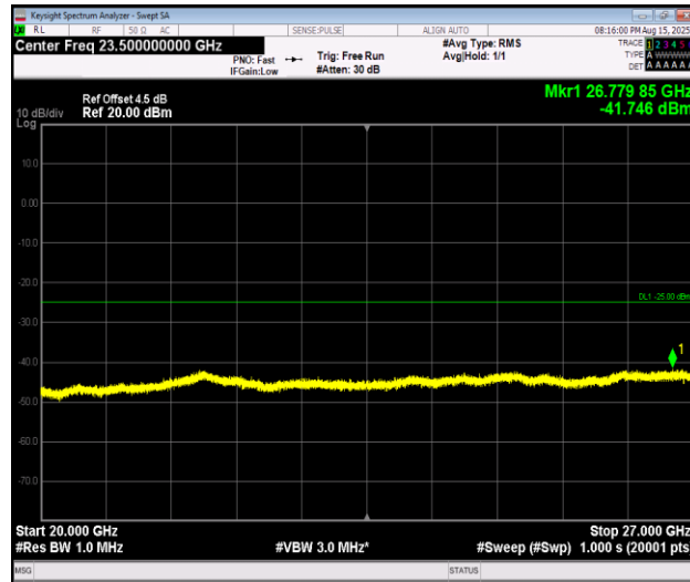
Band7_15MHz_16QAM_21375_1RB#0_20000~27000_20000~27000
