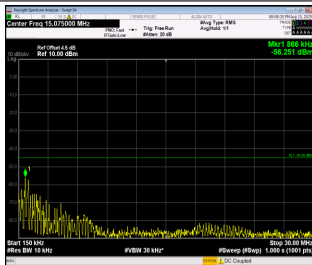
Band7_10MHz_QPSK_21100_1RB#0_0.15~30_0.15~30
