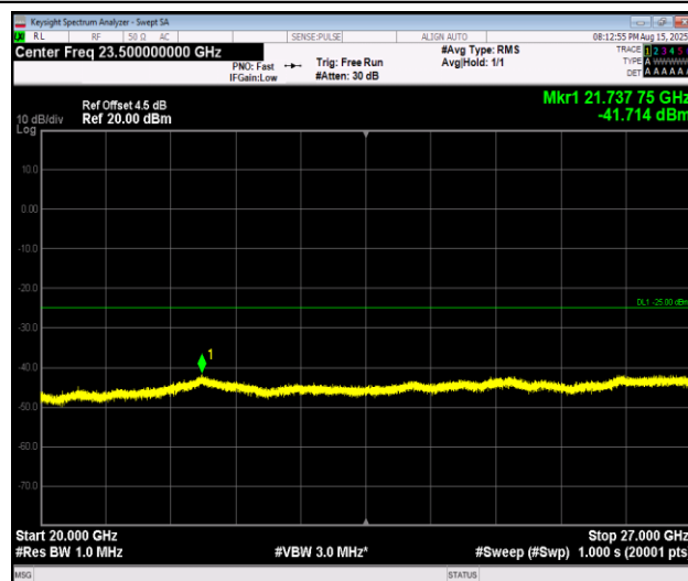
Band7_15MHz_16QAM_20825_1RB#0_20000~27000_20000~27000
