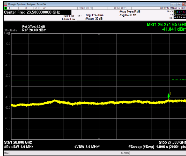
Band7_10MHz_16QAM_20800_1RB#0_20000~27000_20000~27000
