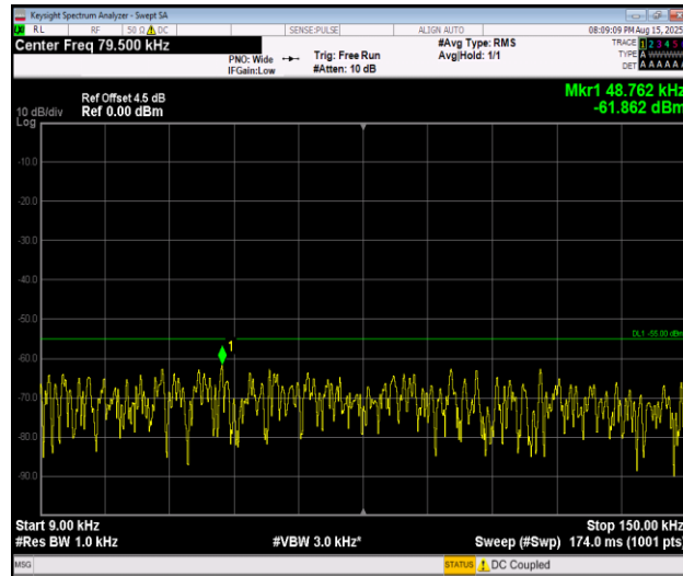
Band7_10MHz_16QAM_21100_1RB#0_0.009~0.15_0.009~0.15
