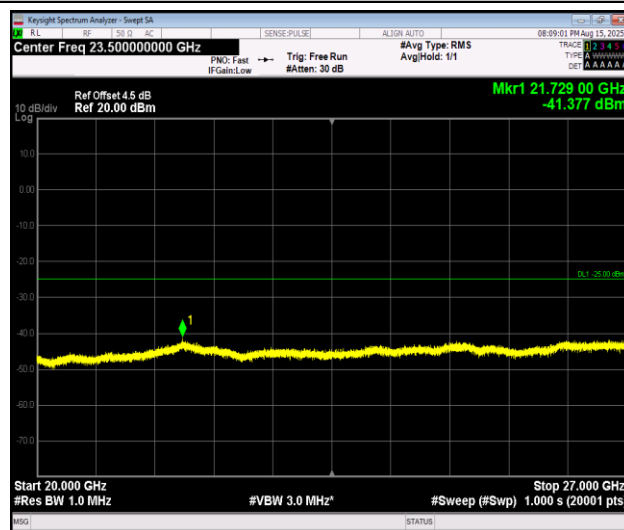
Band7_10MHz_QPSK_21100_1RB#0_20000~27000_20000~27000
