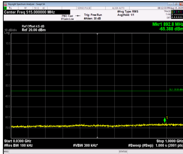
Band7_15MHz_16QAM_20825_1RB#0_30~1000_30~1000
