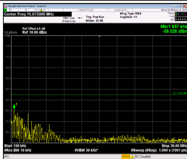
Band7_20MHz_QPSK_20850_1RB#0_0.15~30_0.15~30
