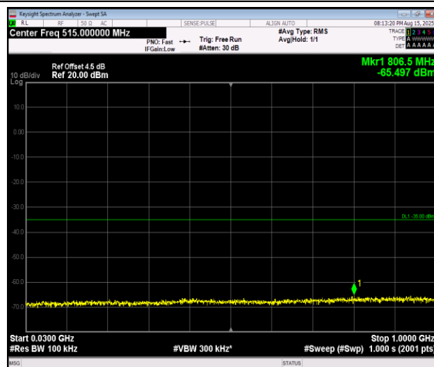
Band7_15MHz_QPSK_21100_1RB#0_30~1000_30~1000
