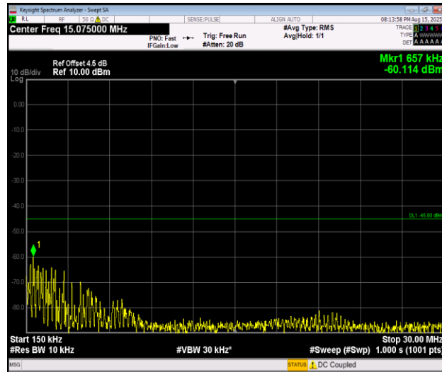
Band7_15MHz_16QAM_21100_1RB#0_0.15~30_0.15~30
