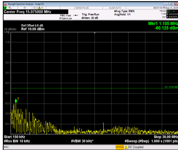
Band7_10MHz_16QAM_20800_1RB#0_0.15~30_0.15~30
