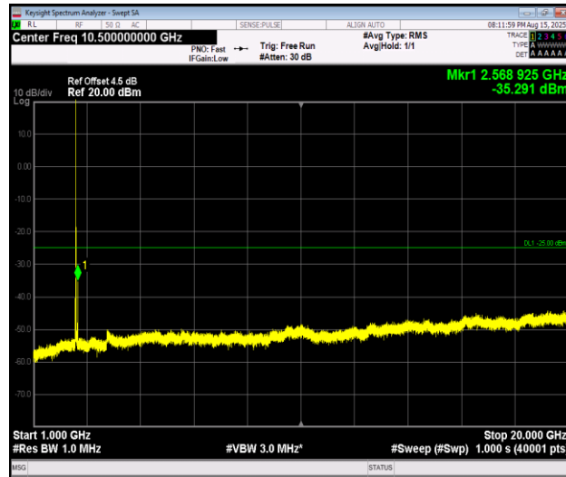
Band7_15MHz_QPSK_20825_1RB#0_1000~20000_1000~20000
