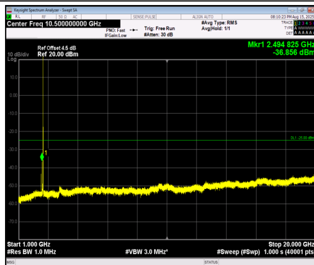
Band7_10MHz_QPSK_21400_1RB#0_1000~20000_1000~20000
