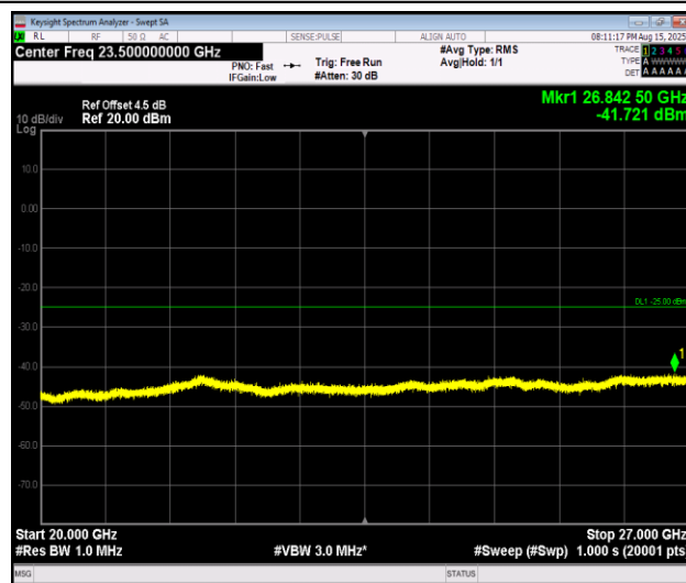
Band7_10MHz_16QAM_21400_1RB#0_20000~27000_20000~27000
