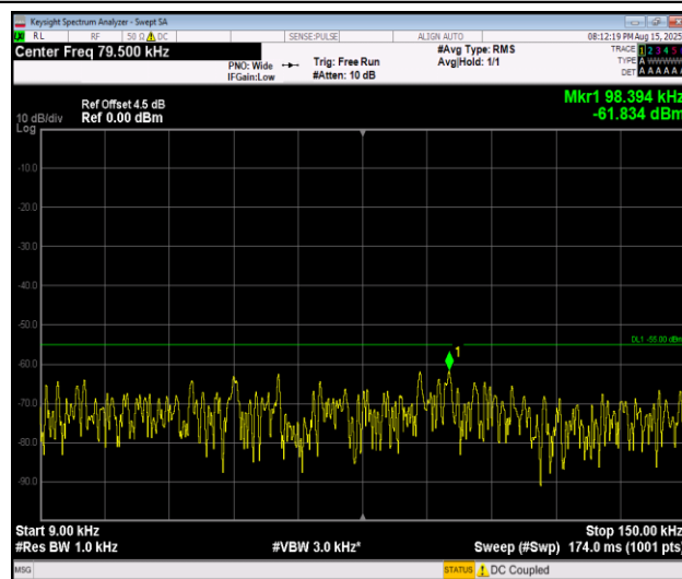
Band7_15MHz_16QAM_20825_1RB#0_0.009~0.15_0.009~0.15
