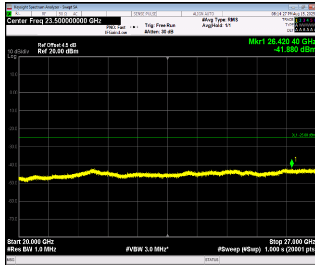
Band7_15MHz_16QAM_21100_1RB#0_20000~27000_20000~27000
