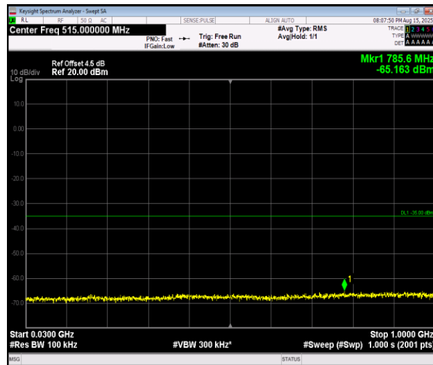
Band7_10MHz_16QAM_20800_1RB#0_30~1000_30~1000
