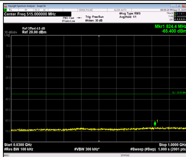
Band7_10MHz_16QAM_21100_1RB#0_30~1000_30~1000
