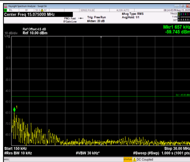
Band7_15MHz_QPSK_21375_1RB#0_0.15~30_0.15~30
