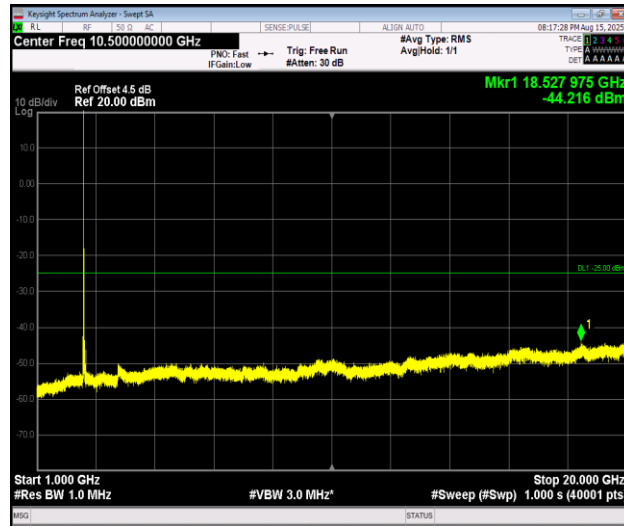
Band7_20MHz_16QAM_20850_1RB#0_1000~20000_1000~20000
