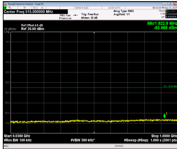
Band7_20MHz_QPSK_20850_1RB#0_30~1000_30~1000
