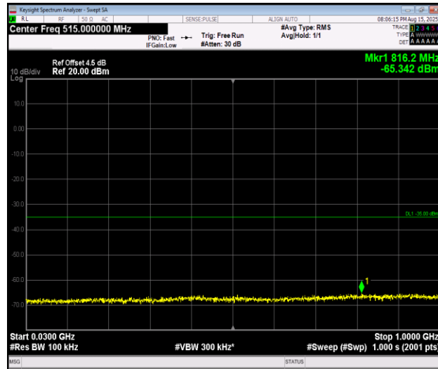
Band7_5MHz_16QAM_21425_1RB#0_30~1000_30~1000
