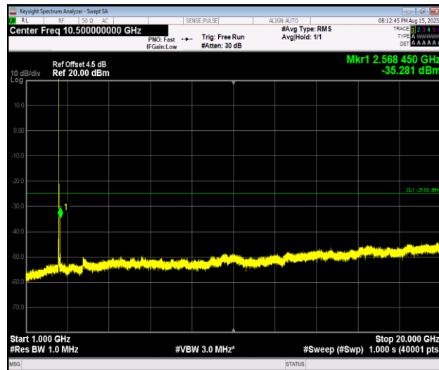
Band7_15MHz_16QAM_20825_1RB#0_1000~20000_1000~20000
