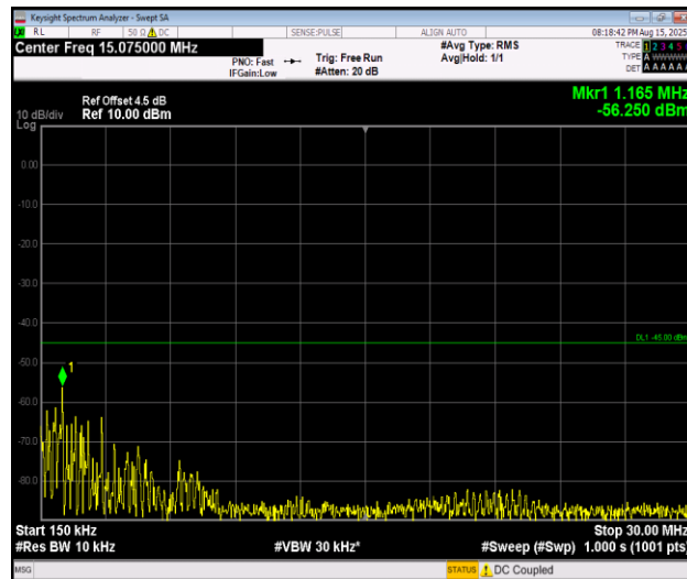
Band7_20MHz_16QAM_21100_1RB#0_0.15~30_0.15~30
