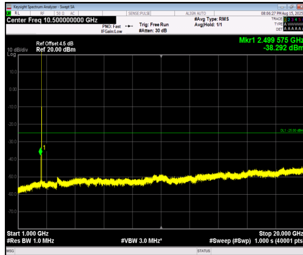
Band7_5MHz_16QAM_21425_1RB#0_1000~20000_1000~20000
