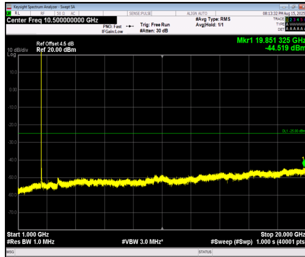
Band7_15MHz_QPSK_21100_1RB#0_1000~20000_1000~20000
