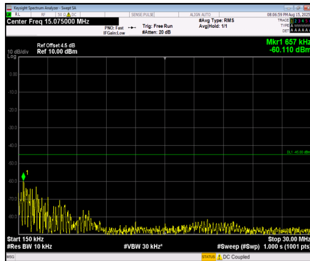
Band7_10MHz_QPSK_20800_1RB#0_0.15~30_0.15~30
