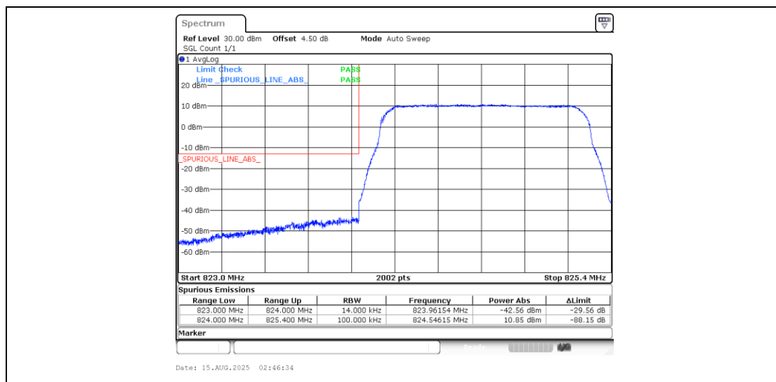
Band5_1.4MHz_16QAM_20407_6RB#0
