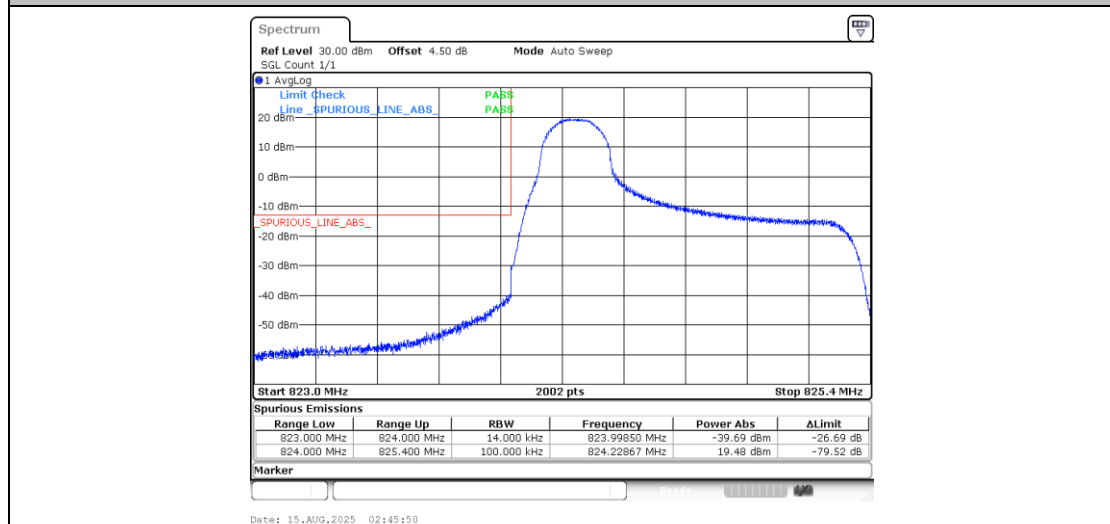
Band5_1.4MHz_16QAM_20407_1RB#0
