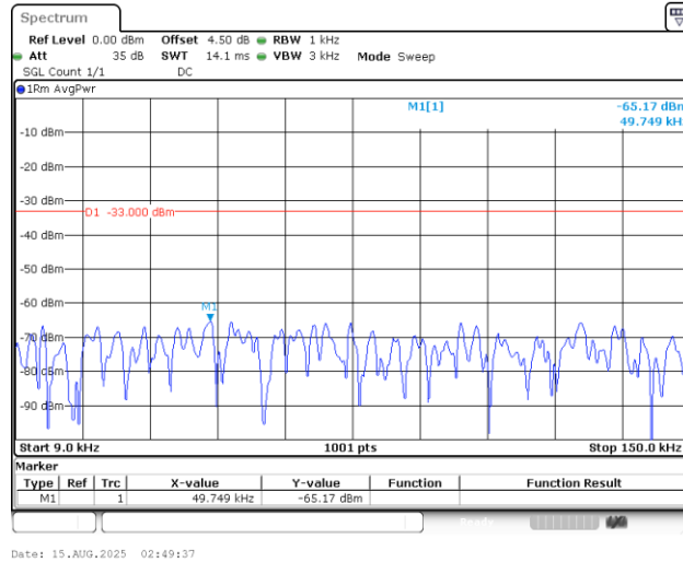
Band5_1.4MHz_QPSK_20525_1RB#0_0.009~0.15_0.009~0.15
