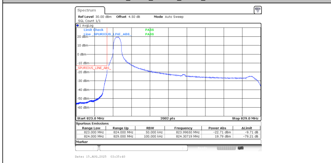
Band5_5MHz_QPSK_20425_1RB#0
