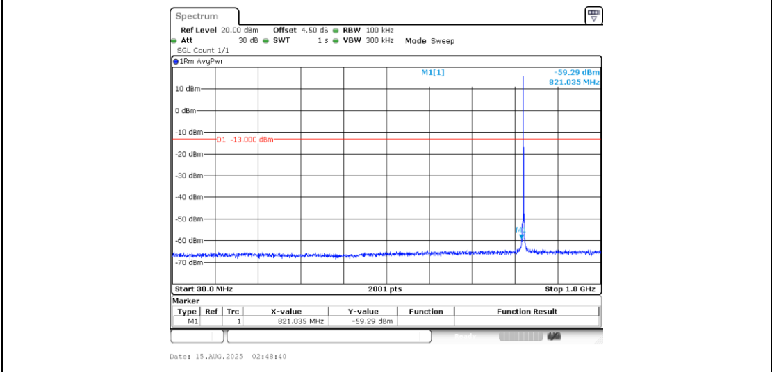
Band5_1.4MHz_QPSK_20407_1RB#0_30~1000_30~1000
