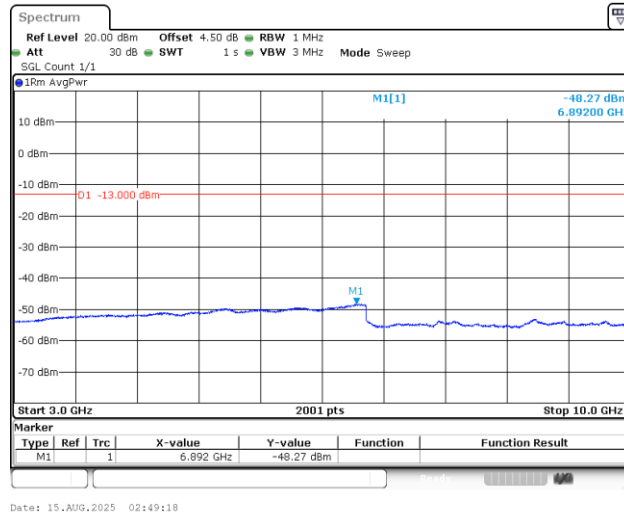
Band5_1.4MHz_16QAM_20407_1RB#0_3000~10000_3000~10000
