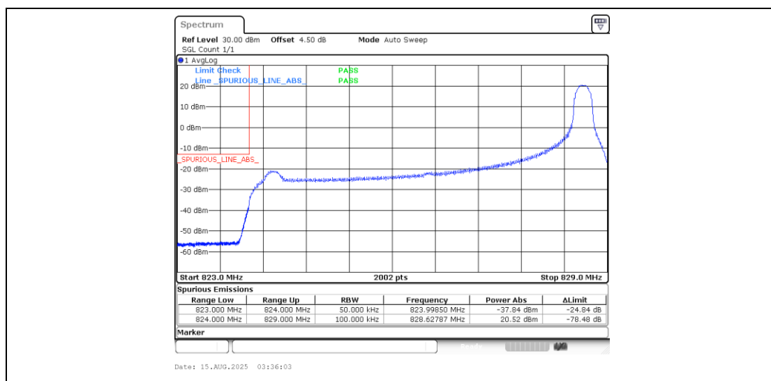
Band5_5MHz_QPSK_20425_1RB#24
