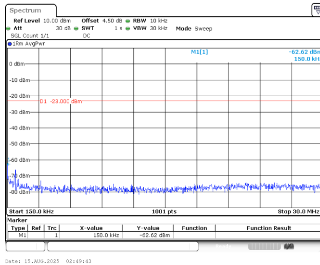
Band5_1.4MHz_QPSK_20525_1RB#0_0.15~30_0.15~30
