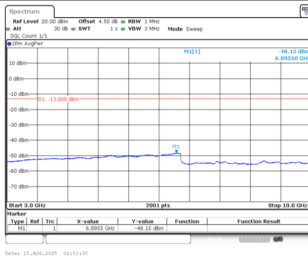
Band5_1.4MHz_16QAM_20643_1RB#0_3000~10000_3000~10000
