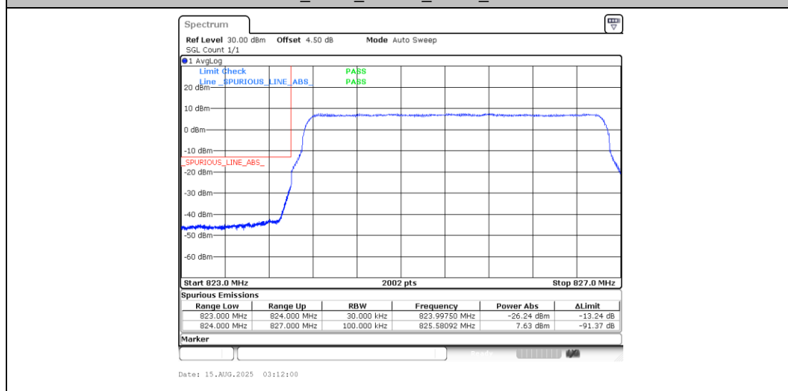
Band5_3MHz_QPSK_20415_15RB#0
