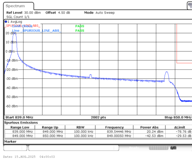
Band5_10MHz_QPSK_20600_1RB#0
