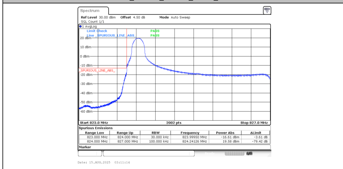
Band5_3MHz_QPSK_20415_1RB#0
