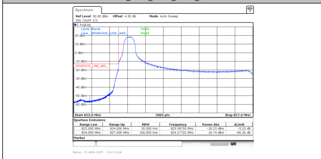
Band5_3MHz_16QAM_20415_1RB#0
