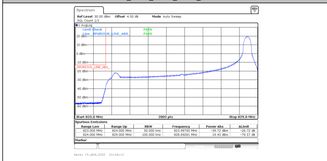
Band5_5MHz_16QAM_20425_1RB#24
