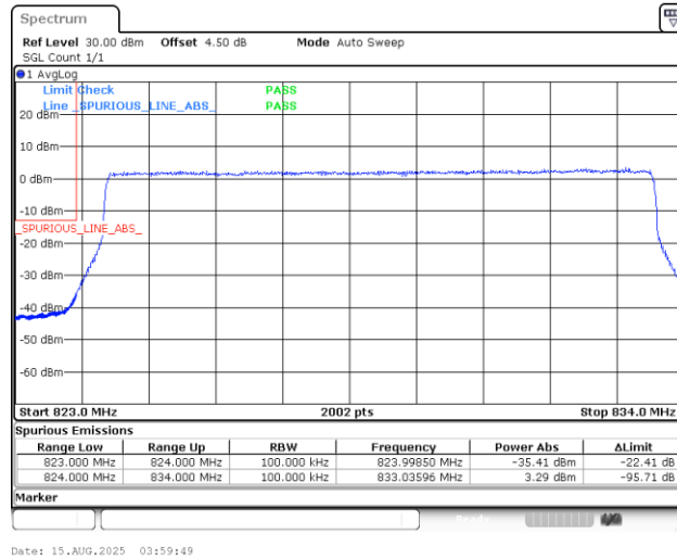
Band5_10MHz_16QAM_20450_50RB#0
