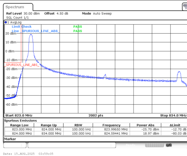
Band5_10MHz_16QAM_20450_1RB#0
