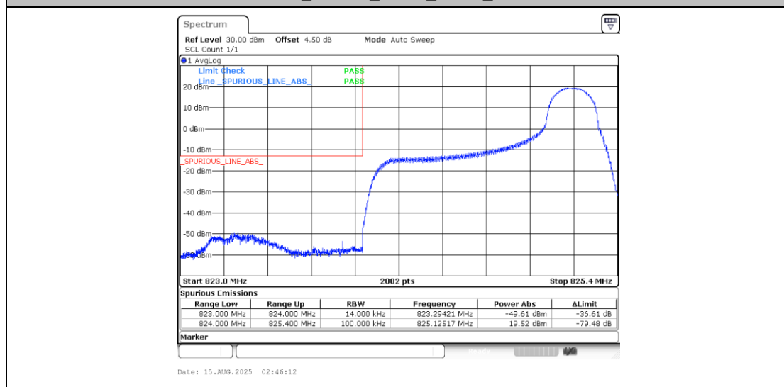
Band5_1.4MHz_16QAM_20407_1RB#5
