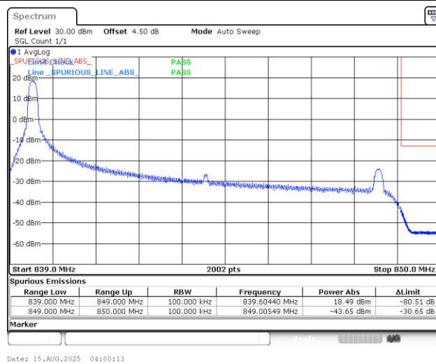
Band5_10MHz_16QAM_20600_1RB#0
