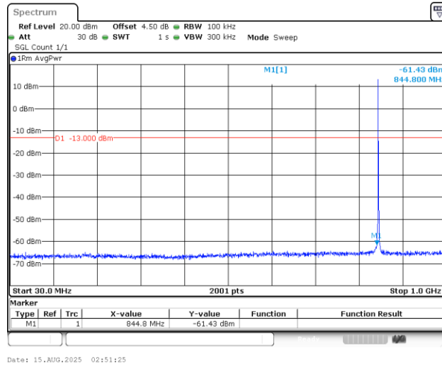
Band5_1.4MHz_16QAM_20643_1RB#0_30~1000_30~1000
