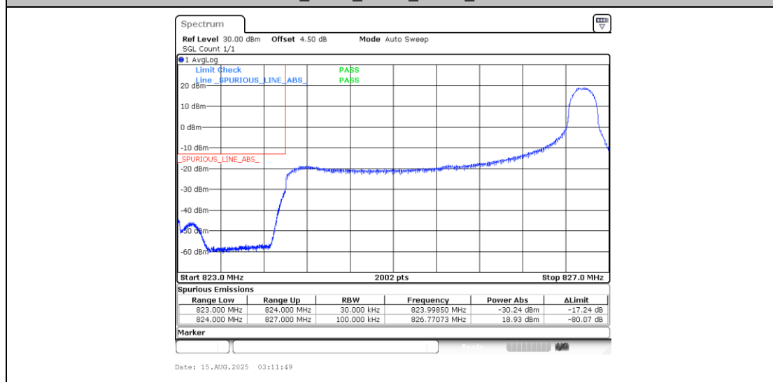
Band5_3MHz_16QAM_20415_1RB#14
