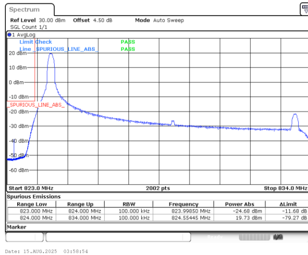
Band5_10MHz_QPSK_20450_1RB#0
