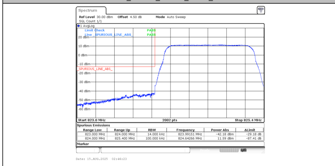
Band5_1.4MHz_QPSK_20407_6RB#0
