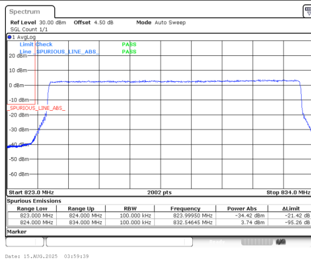
Band5_10MHz_QPSK_20450_50RB#0
