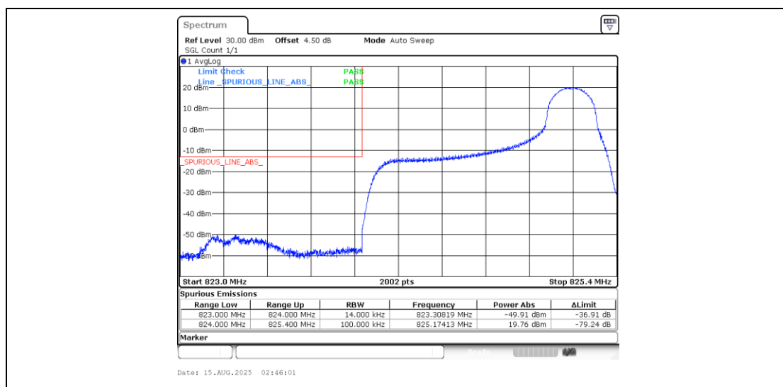
Band5_1.4MHz_QPSK_20407_1RB#5
