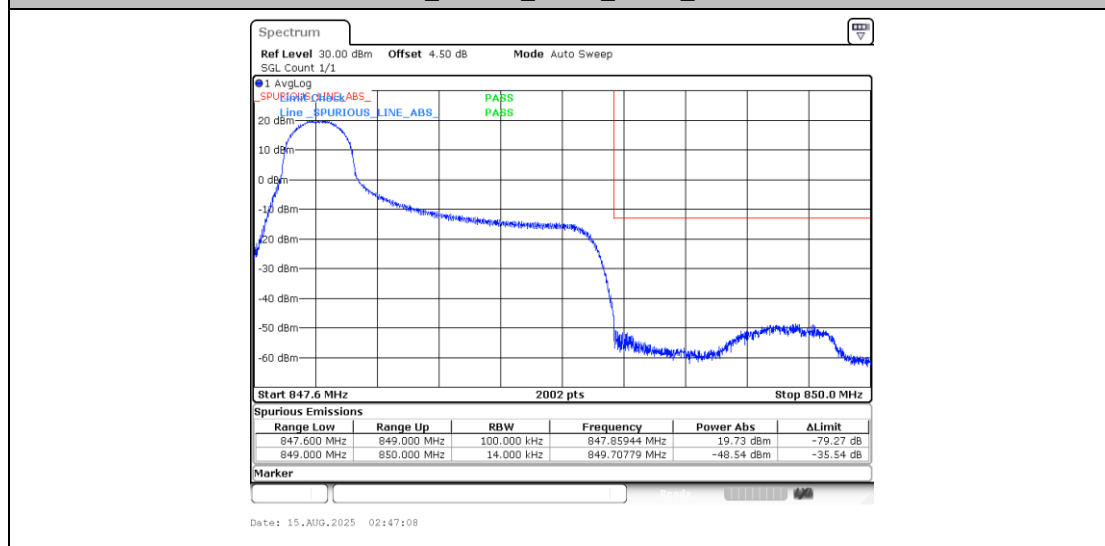
Band5_1.4MHz_16QAM_20643_1RB#0
