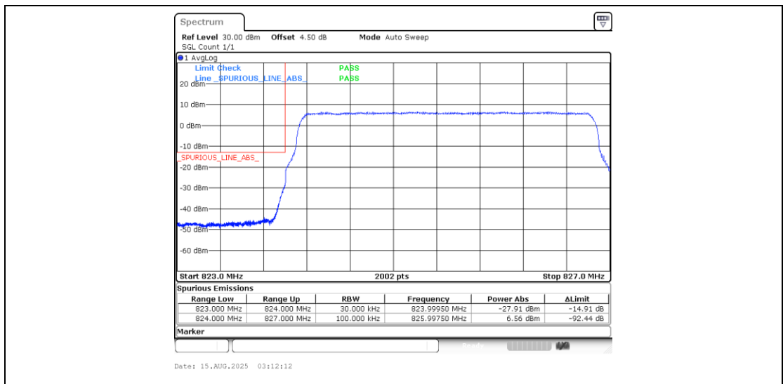
Band5_3MHz_16QAM_20415_15RB#0
