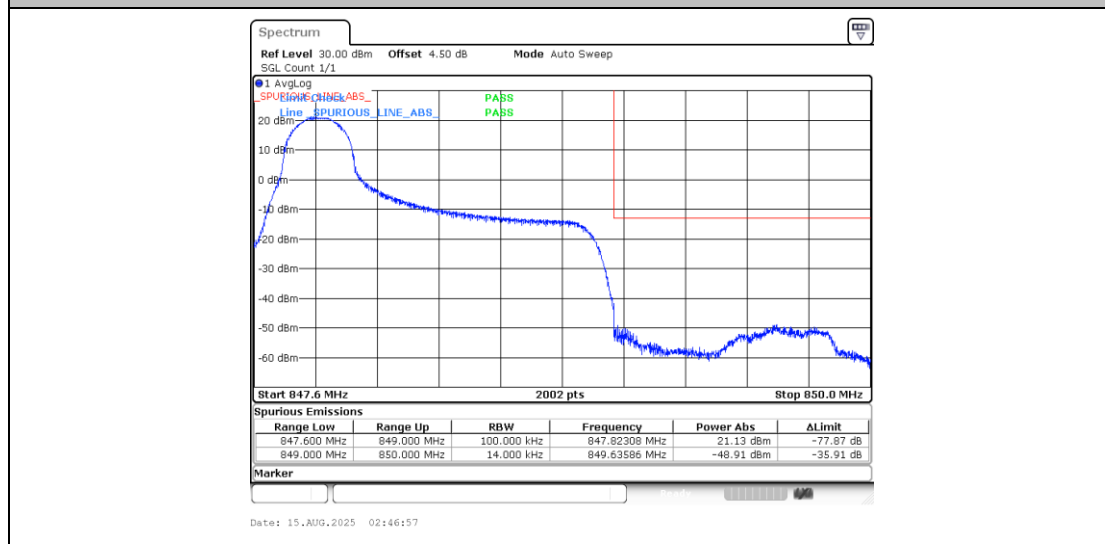
Band5_1.4MHz_QPSK_20643_1RB#0
