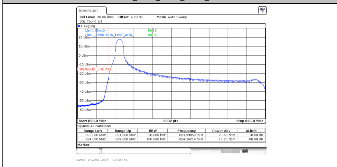
Band5_5MHz_16QAM_20425_1RB#0
