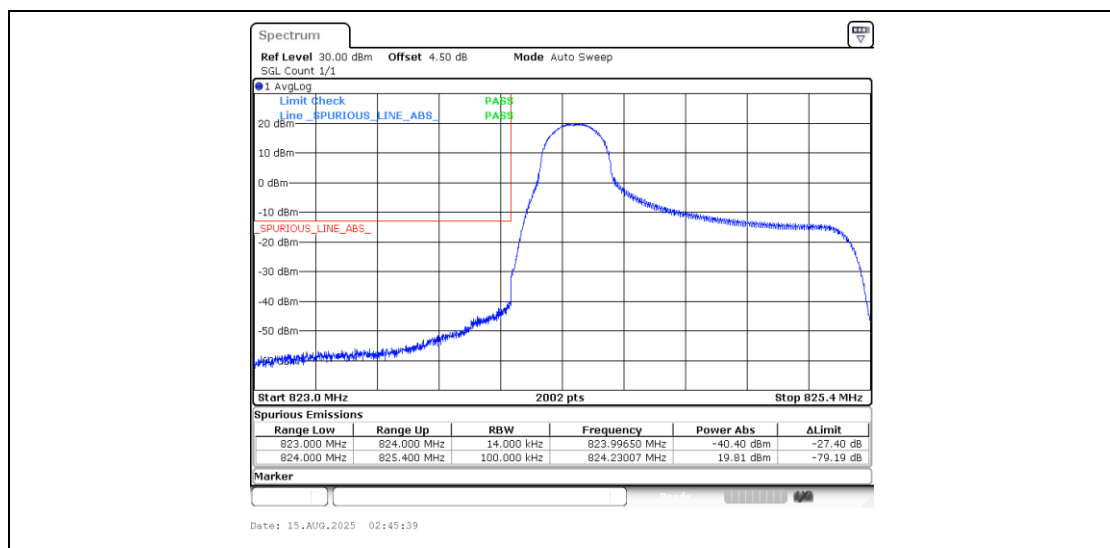
Band5_1.4MHz_QPSK_20407_1RB#0
