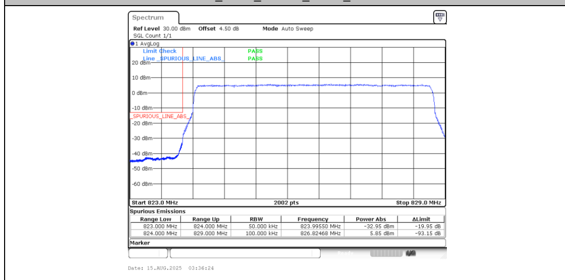
Band5_5MHz_QPSK_20425_25RB#0
