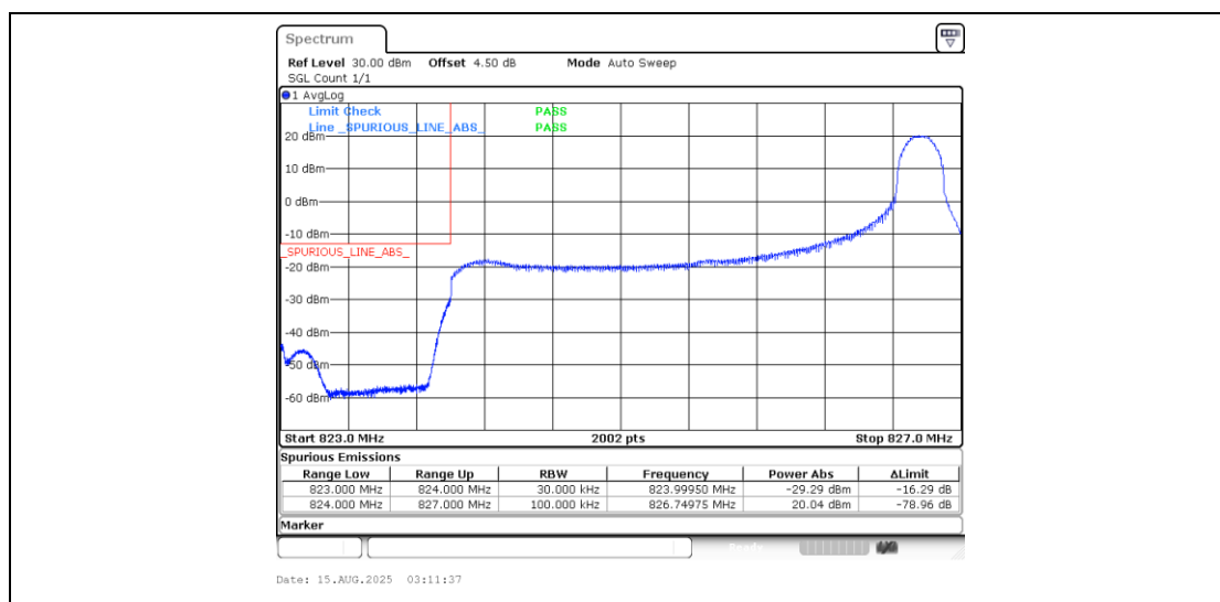
Band5_3MHz_QPSK_20415_1RB#14
