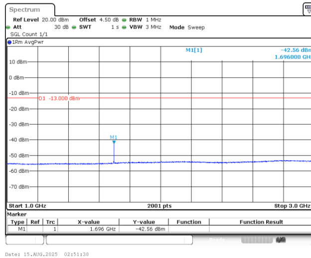
Band5_1.4MHz_16QAM_20643_1RB#0_1000~3000_1000~3000
