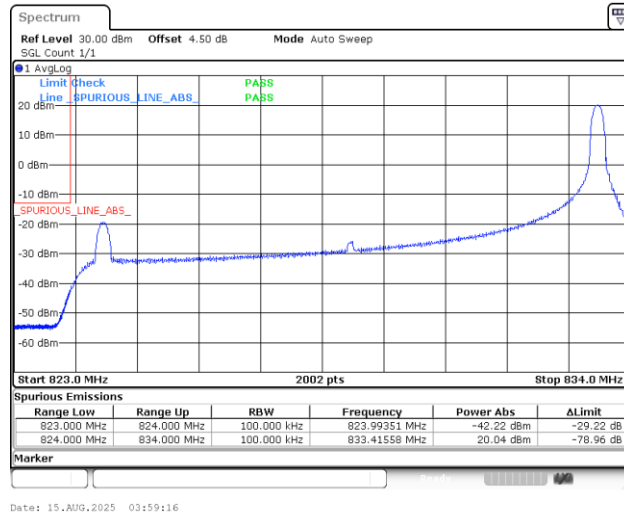
Band5_10MHz_QPSK_20450_1RB#49
