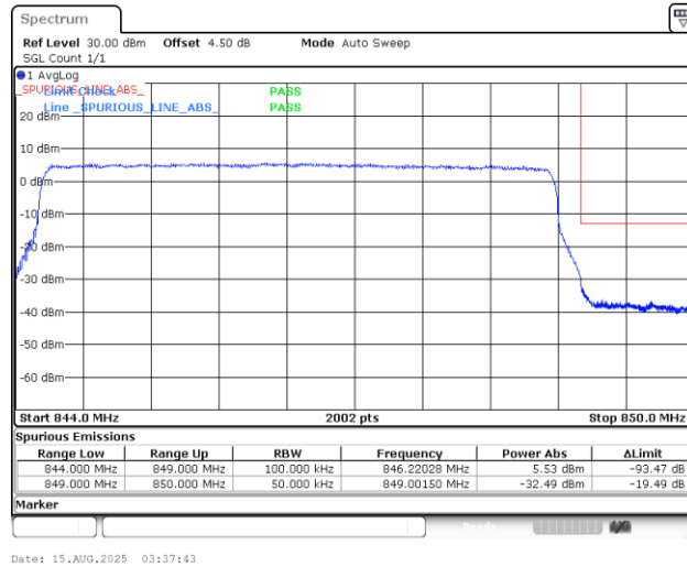
Band5_5MHz_16QAM_20625_25RB#0
