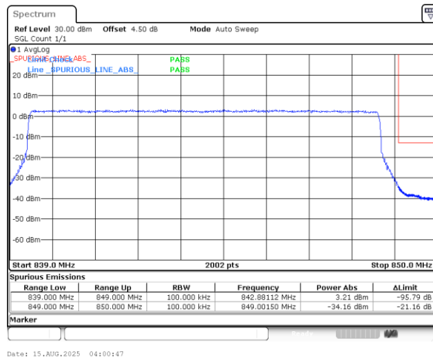
Band5_10MHz_QPSK_20600_50RB#0
