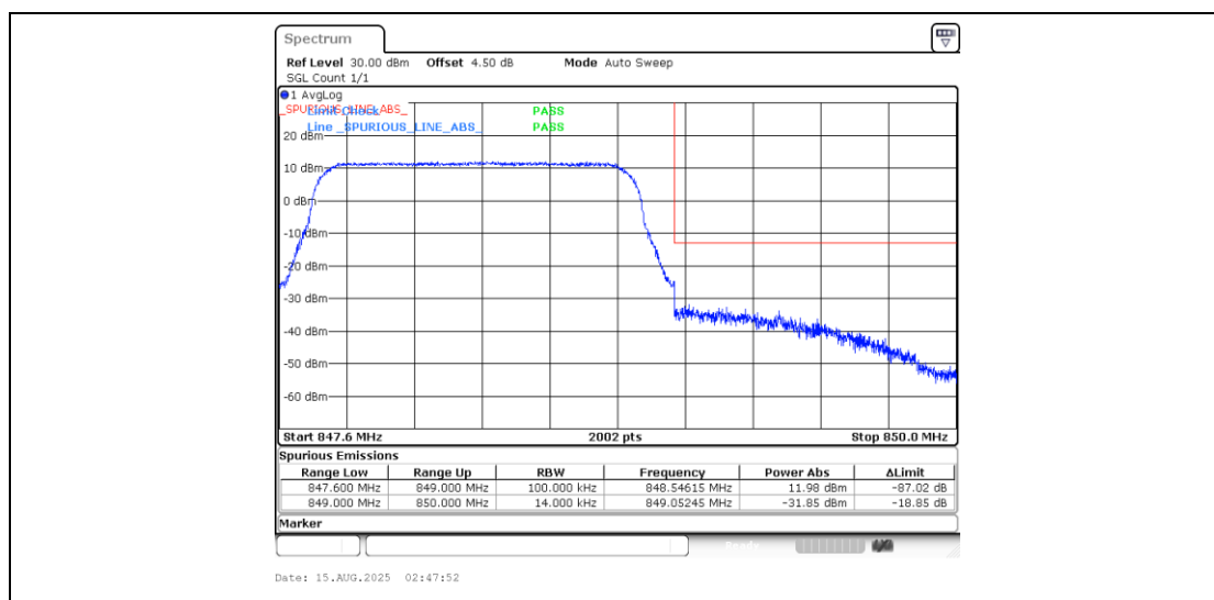
Band5_1.4MHz_16QAM_20643_6RB#0
