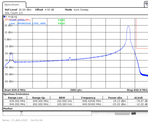
Band5_10MHz_16QAM_20600_1RB#49
