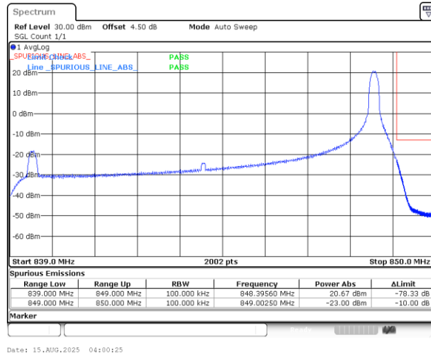
Band5_10MHz_QPSK_20600_1RB#49
