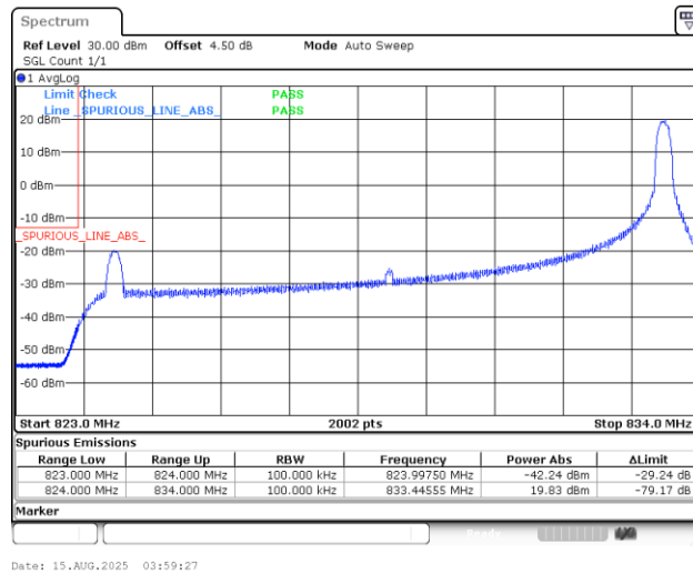
Band5_10MHz_16QAM_20450_1RB#49
