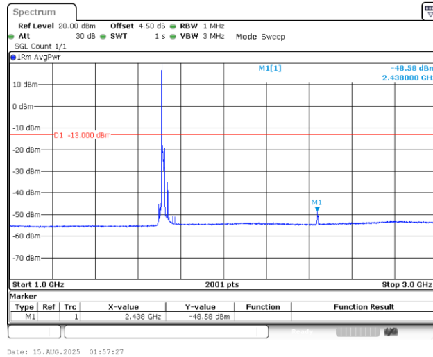
Band4_15MHz_16QAM_20025_1RB#0_1000~3000_1000~3000
