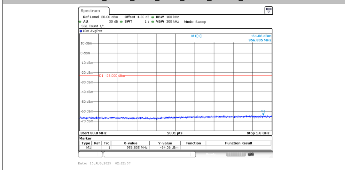
Band4_20MHz_QPSK_20175_1RB#0_30~1000_30~1000
