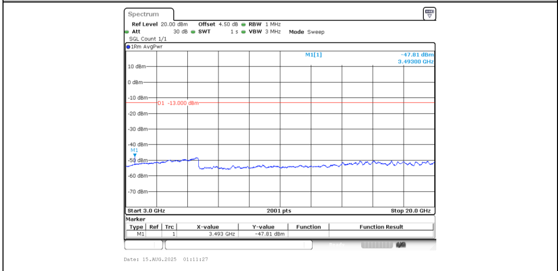
Band4_5MHz_QPSK_20375_1RB#0_3000~20000_3000~20000
