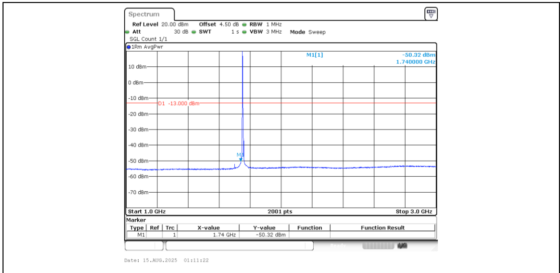
Band4_5MHz_QPSK_20375_1RB#0_1000~3000_1000~3000
