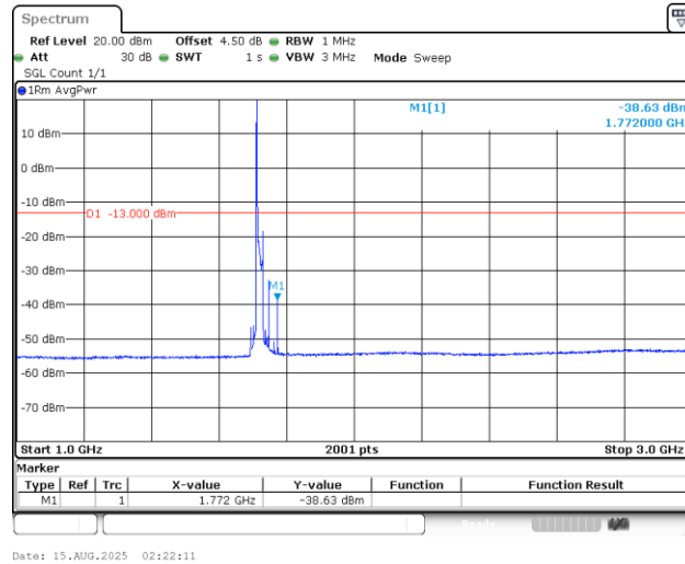
Band4_20MHz_16QAM_20050_1RB#0_1000~3000_1000~3000
