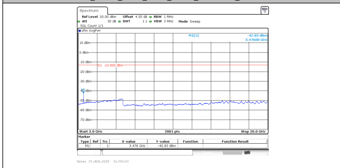
Band4_15MHz_QPSK_20325_1RB#0_3000~20000_3000~20000
