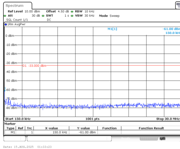
Band4_10MHz_QPSK_20175_1RB#0_0.15~30_0.15~30
