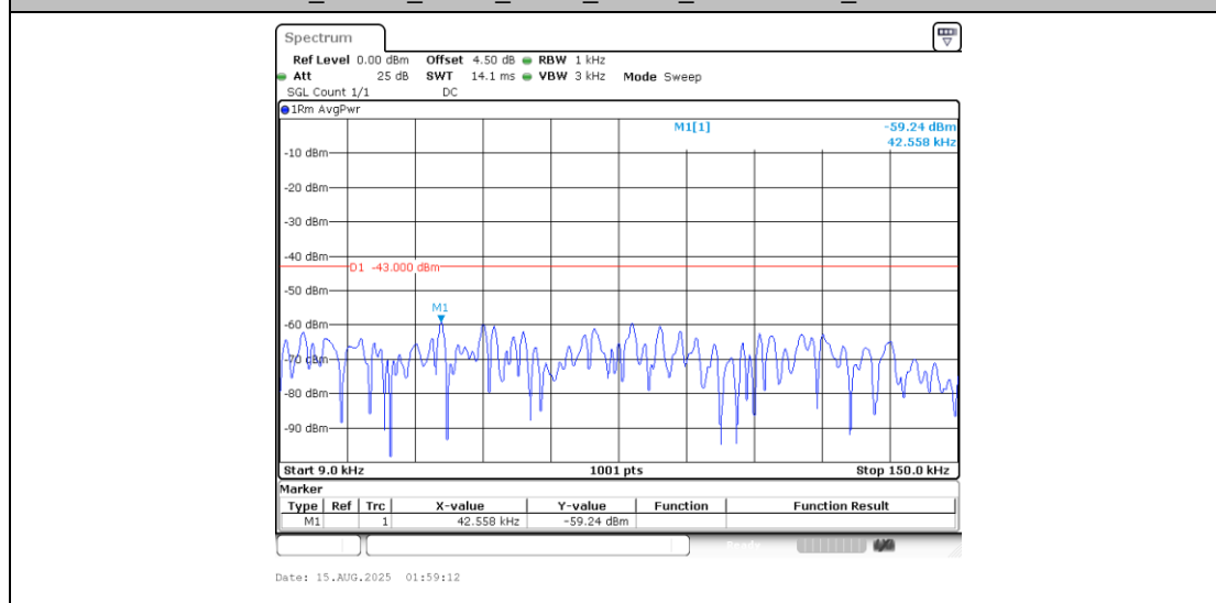
Band4_15MHz_16QAM_20325_1RB#0_0.009~0.15_0.009~0.15
