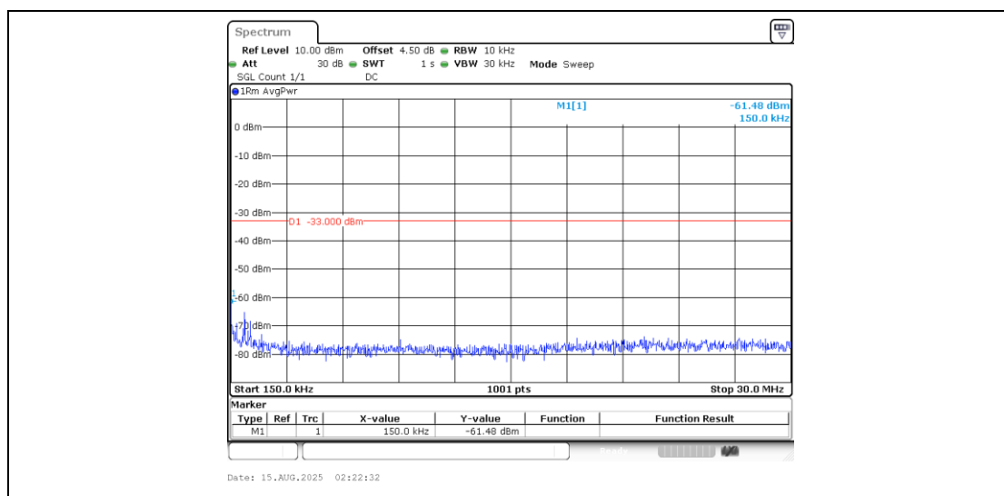
Band4_20MHz_QPSK_20175_1RB#0_0.15~30_0.15~30
