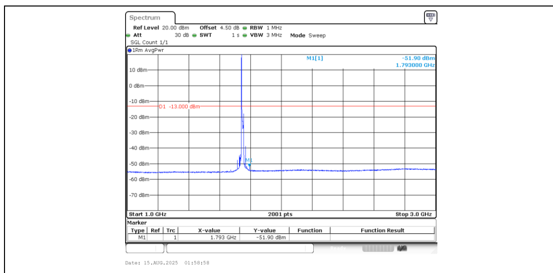
Band4_15MHz_QPSK_20325_1RB#0_1000~3000_1000~3000
