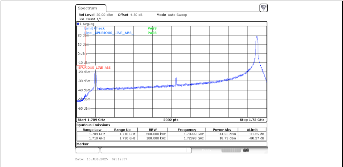
Band4_20MHz_16QAM_20050_1RB#99
