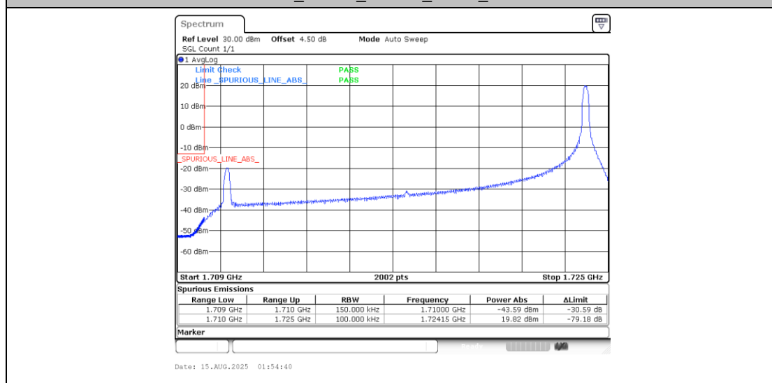
Band4_15MHz_QPSK_20025_1RB#74
