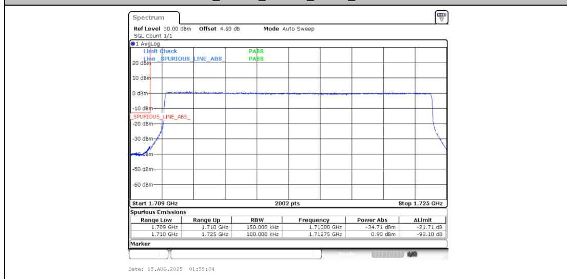
Band4_15MHz_QPSK_20025_75RB#0
