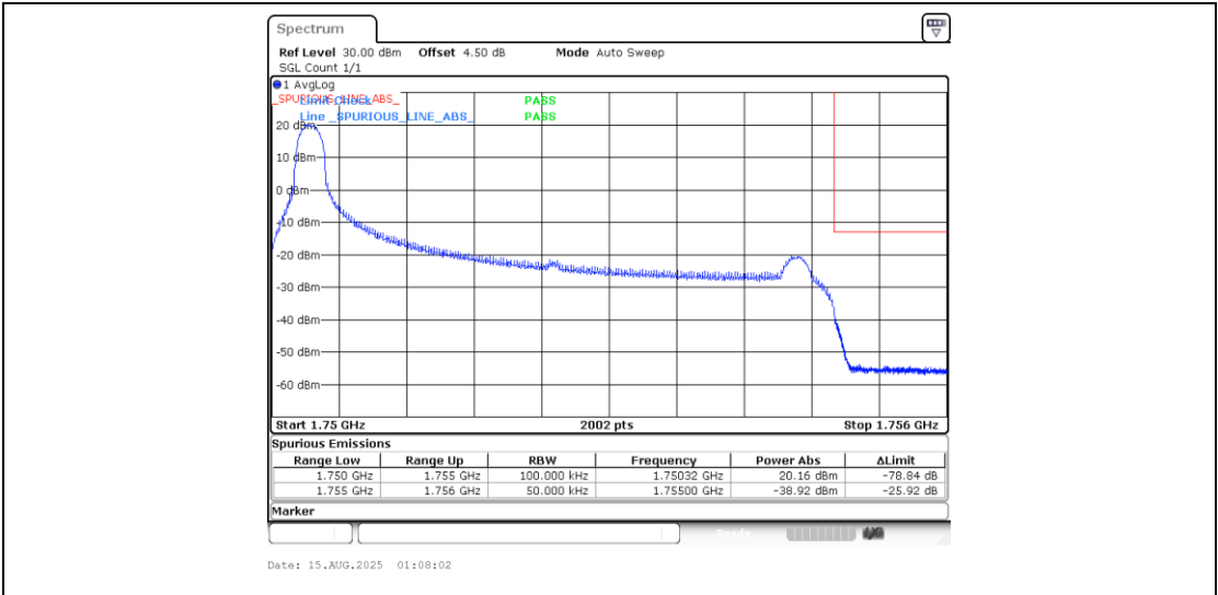
Band4_5MHz_QPSK_20375_1RB#0
