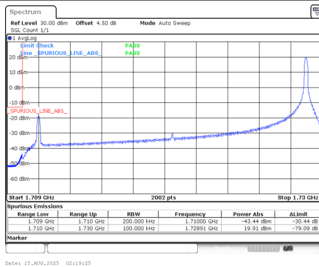
Band4_20MHz_QPSK_20050_1RB#99
