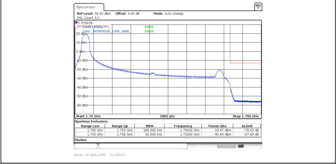
Band4_5MHz_16QAM_20375_1RB#0
