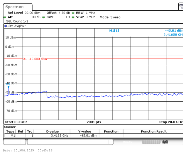
Band4_3MHz_QPSK_19965_1RB#0_3000~20000_3000~20000
