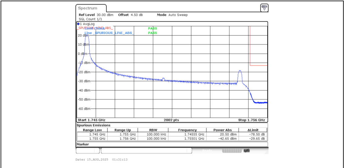
Band4_10MHz_QPSK_20350_1RB#0
