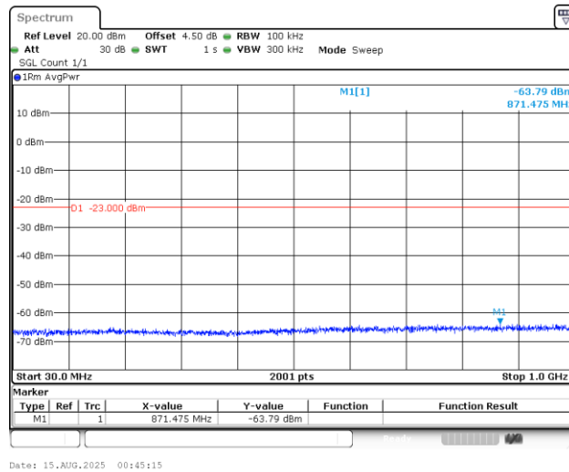
Band4_3MHz_QPSK_19965_1RB#0_30~1000_30~1000
