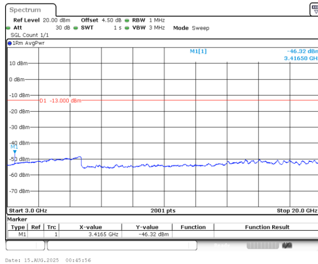
Band4_3MHz_16QAM_19965_1RB#0_3000~20000_3000~20000
