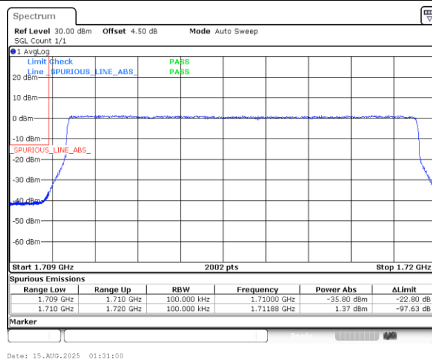
Band4_10MHz_16QAM_20000_50RB#0
