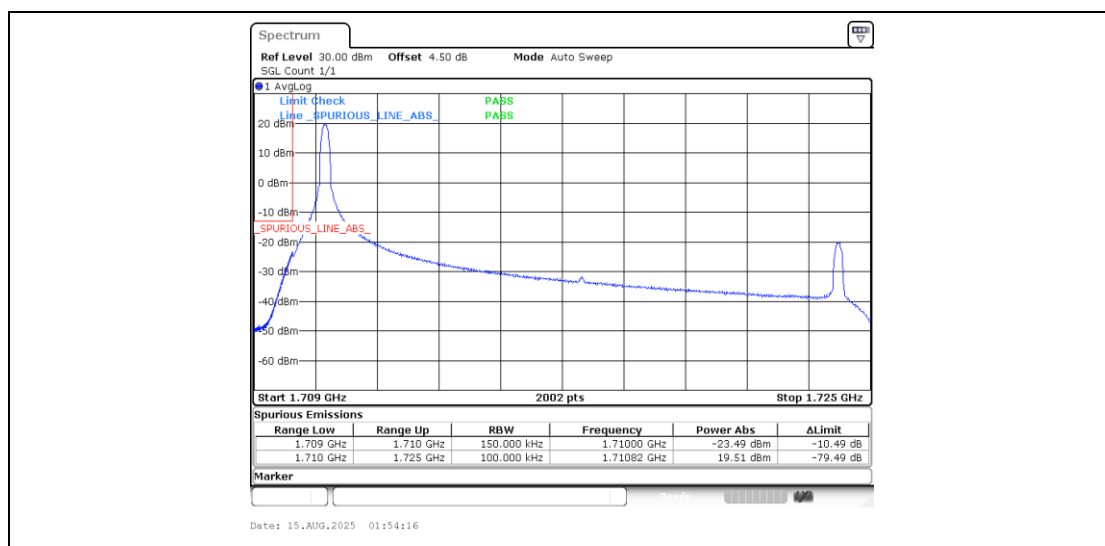
Band4_15MHz_QPSK_20025_1RB#0
