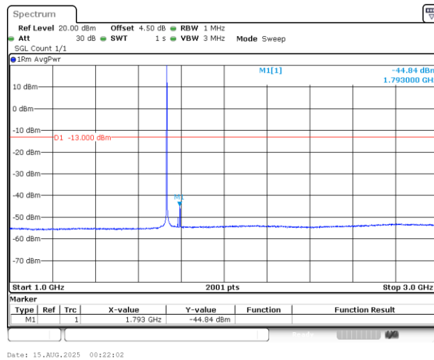
Band4_1.4MHz_QPSK_20175_1RB#0_1000~3000_1000~3000
