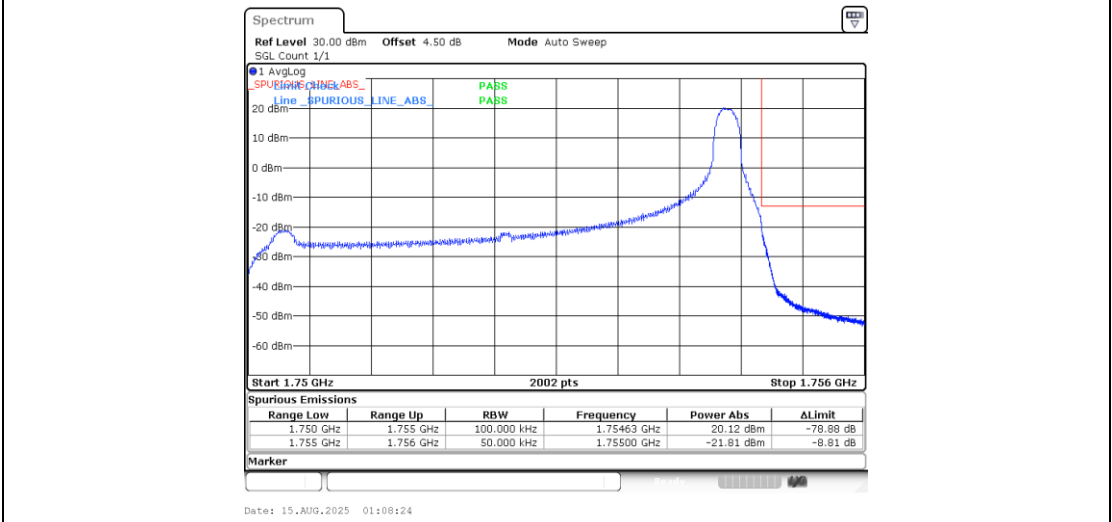
Band4_5MHz_QPSK_20375_1RB#24
