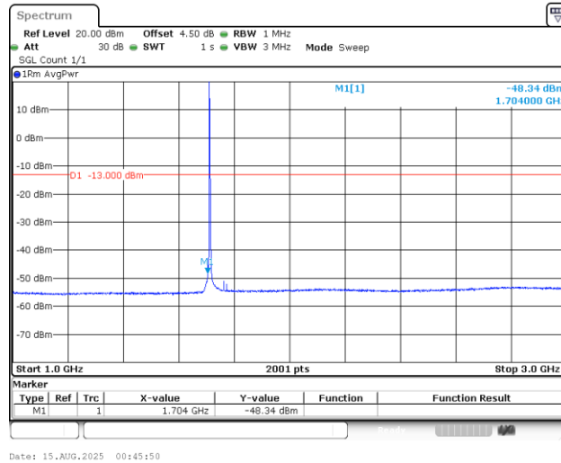
Band4_3MHz_16QAM_19965_1RB#0_1000~3000_1000~3000
