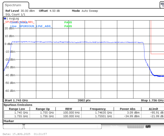
Band4_10MHz_QPSK_20350_50RB#0
