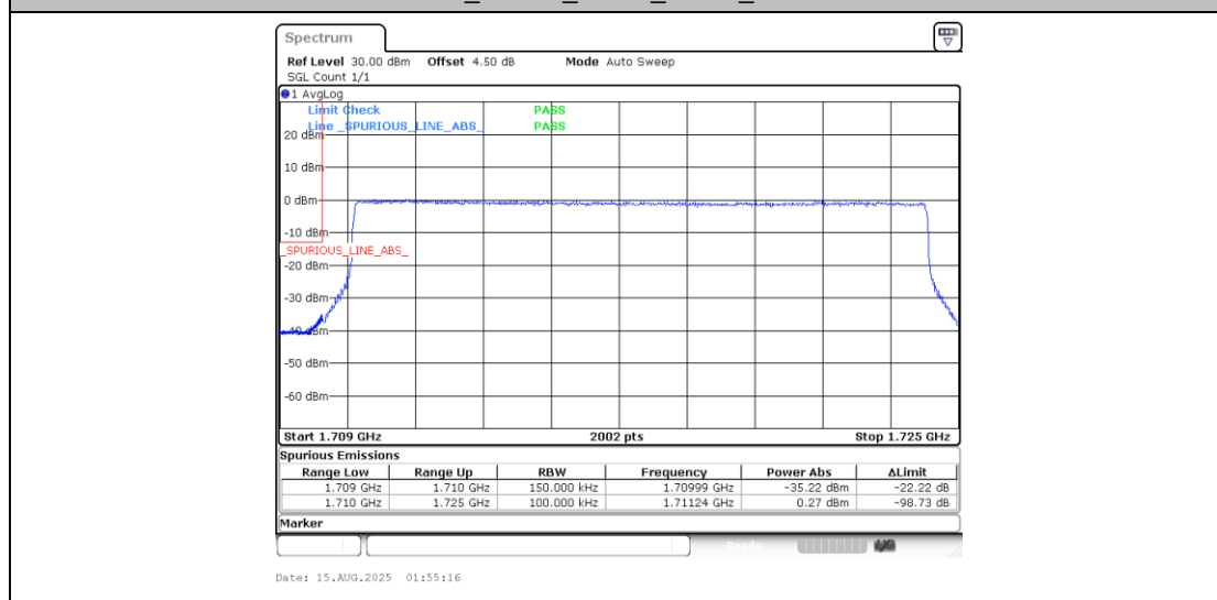
Band4_15MHz_16QAM_20025_75RB#0
