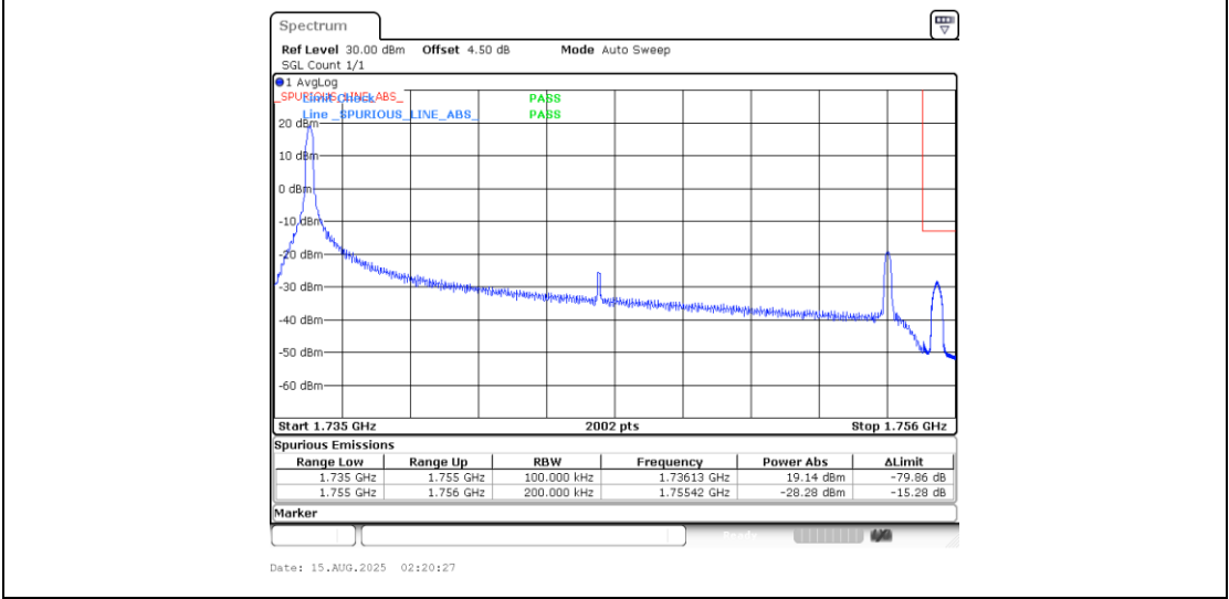
Band4_20MHz_16QAM_20300_1RB#0
