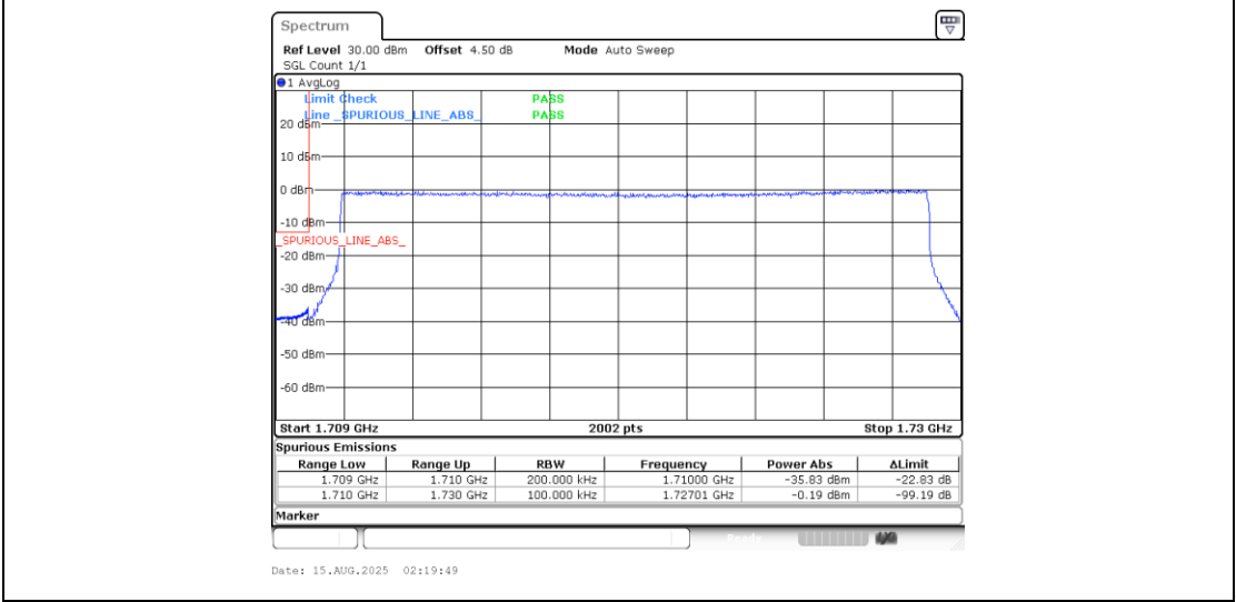
Band4_20MHz_QPSK_20050_100RB#0
