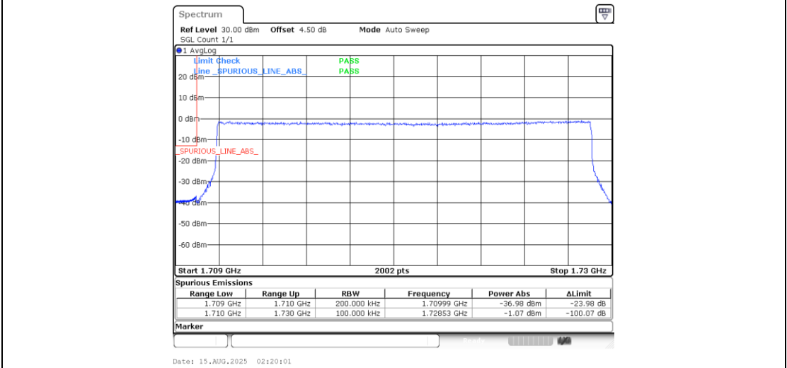
Band4_20MHz_16QAM_20050_100RB#0
