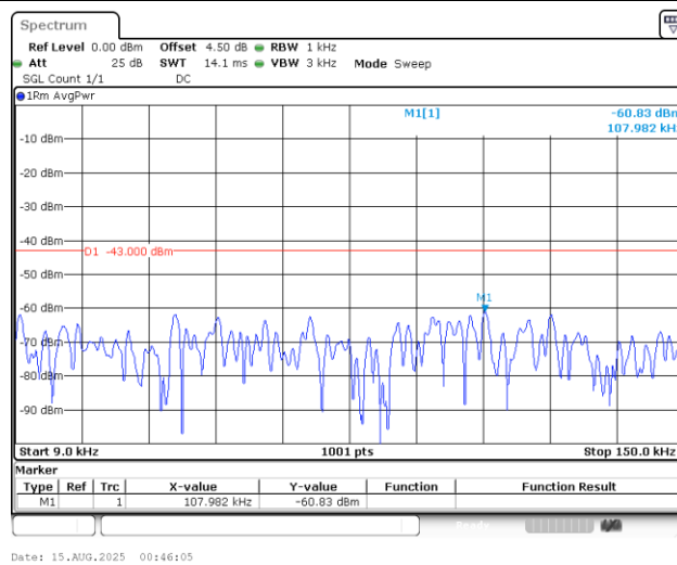
Band4_3MHz_QPSK_20175_1RB#0_0.009~0.15_0.009~0.15
