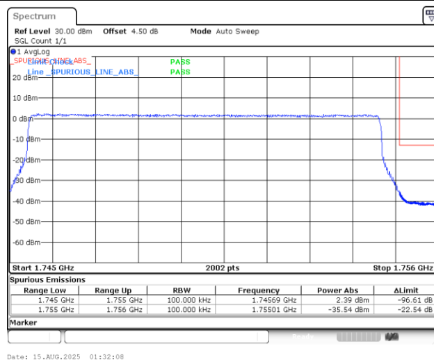
Band4_10MHz_16QAM_20350_50RB#0
