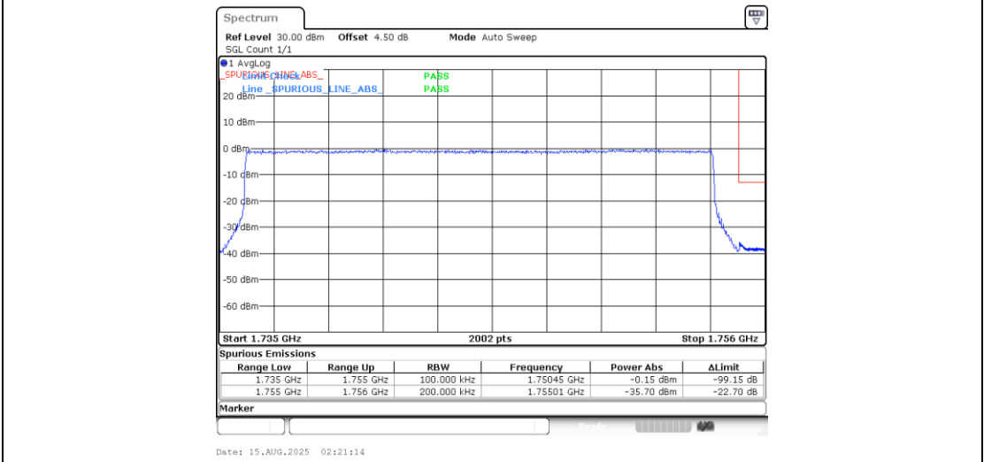
Band4_20MHz_16QAM_20300_100RB#0
