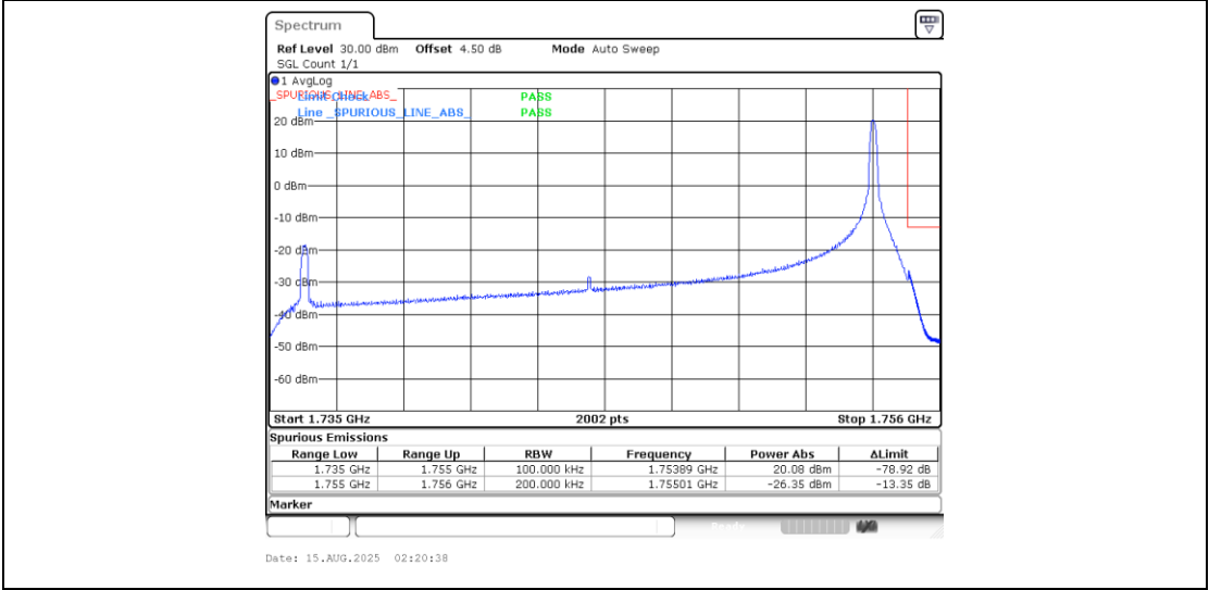
Band4_20MHz_QPSK_20300_1RB#99
