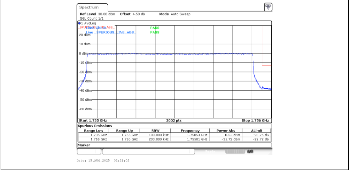
Band4_20MHz_QPSK_20300_100RB#0
