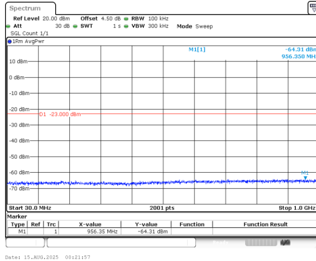
Band4_1.4MHz_QPSK_20175_1RB#0_30~1000_30~1000
