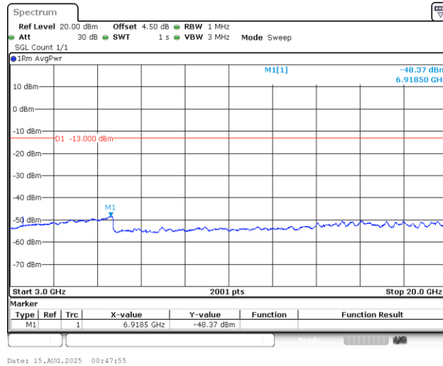
Band4_3MHz_16QAM_20385_1RB#0_3000~20000_3000~20000
