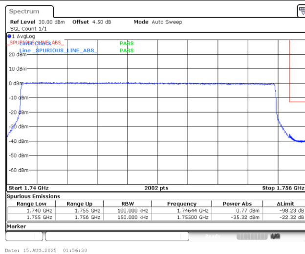
Band4_15MHz_16QAM_20325_75RB#0
