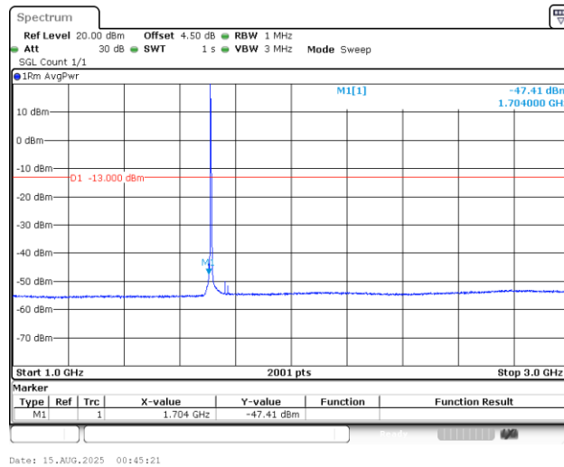
Band4_3MHz_QPSK_19965_1RB#0_1000~3000_1000~3000
