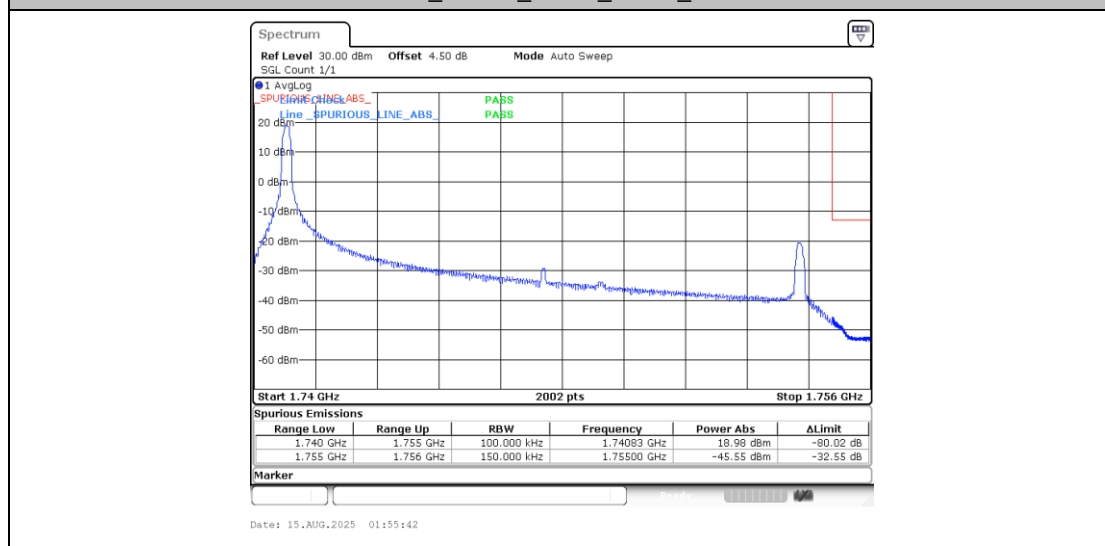
Band4_15MHz_16QAM_20325_1RB#0
