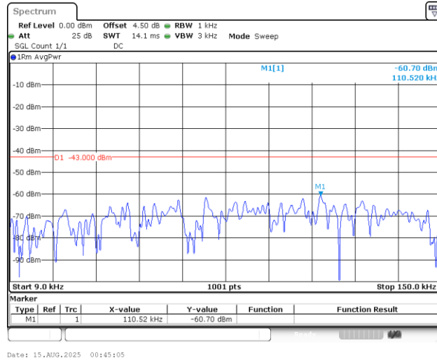
Band4_3MHz_QPSK_19965_1RB#0_0.009~0.15_0.009~0.15
