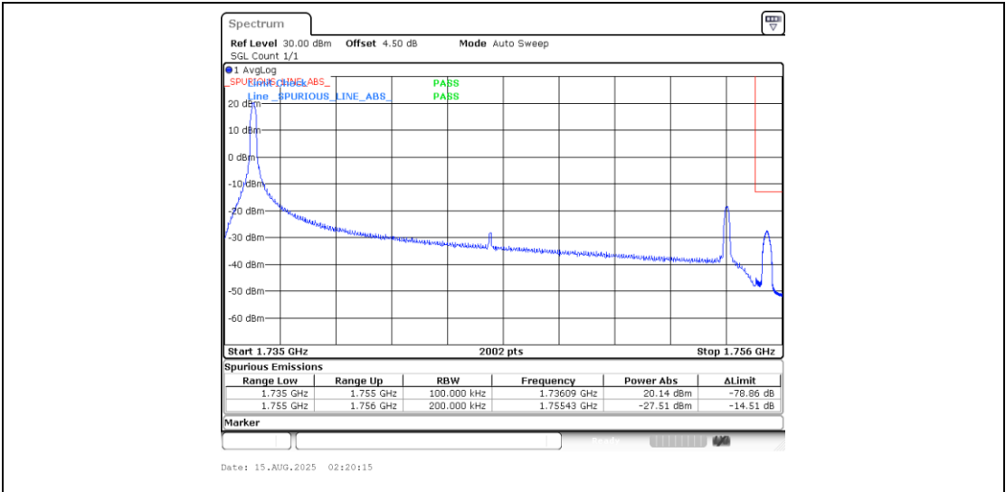
Band4_20MHz_QPSK_20300_1RB#0
