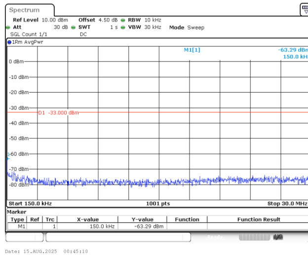
Band4_3MHz_QPSK_19965_1RB#0_0.15~30_0.15~30
