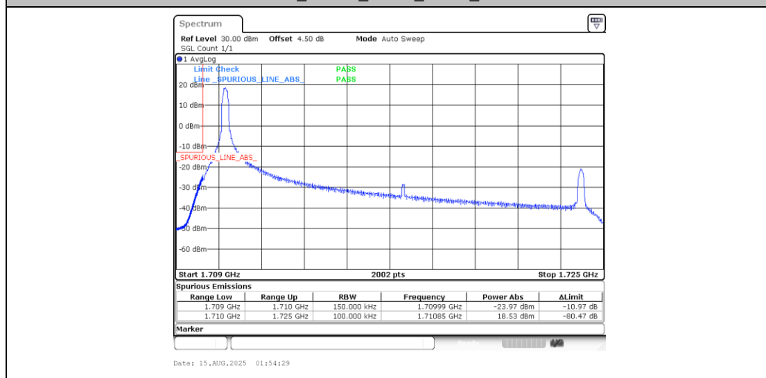
Band4_15MHz_16QAM_20025_1RB#0
