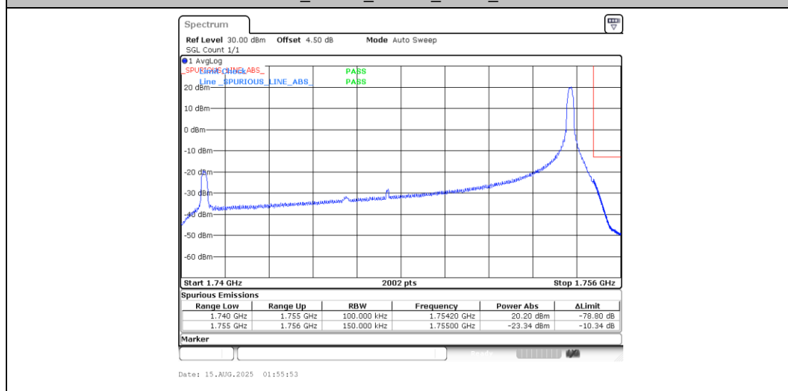
Band4_15MHz_QPSK_20325_1RB#74
