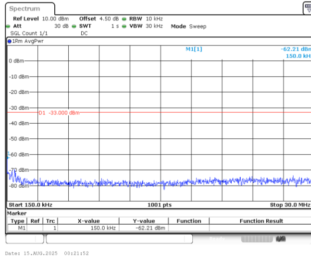
Band4_1.4MHz_QPSK_20175_1RB#0_0.15~30_0.15~30
