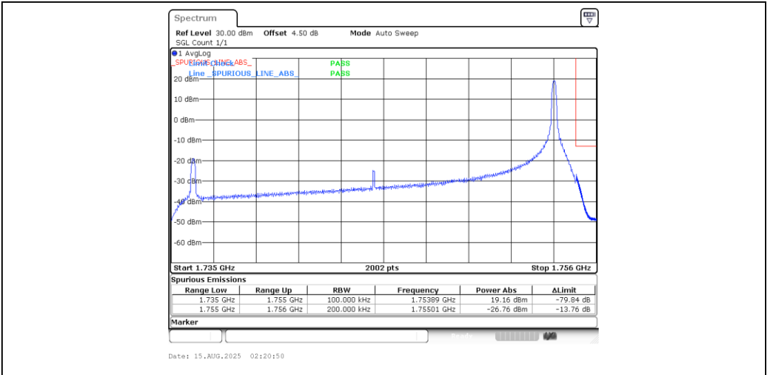
Band4_20MHz_16QAM_20300_1RB#99
