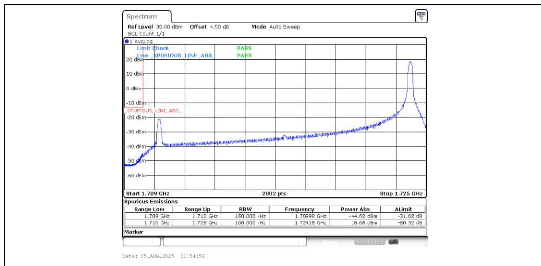
Band4_15MHz_16QAM_20025_1RB#74
