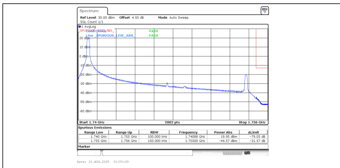
Band4_15MHz_QPSK_20325_1RB#0
