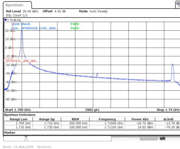
Band4_20MHz_QPSK_20050_1RB#0
