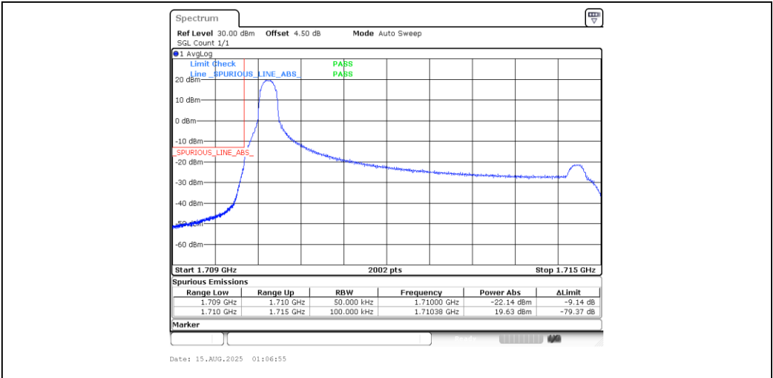
Band4_5MHz_QPSK_19975_1RB#0
