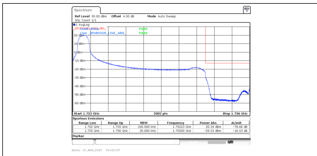
Band4_3MHz_QPSK_20385_1RB#0
