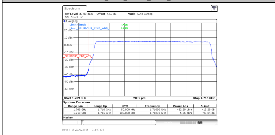
Band4_5MHz_QPSK_19975_25RB#0
