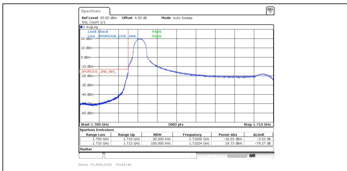
Band4_3MHz_QPSK_19965_1RB#0
