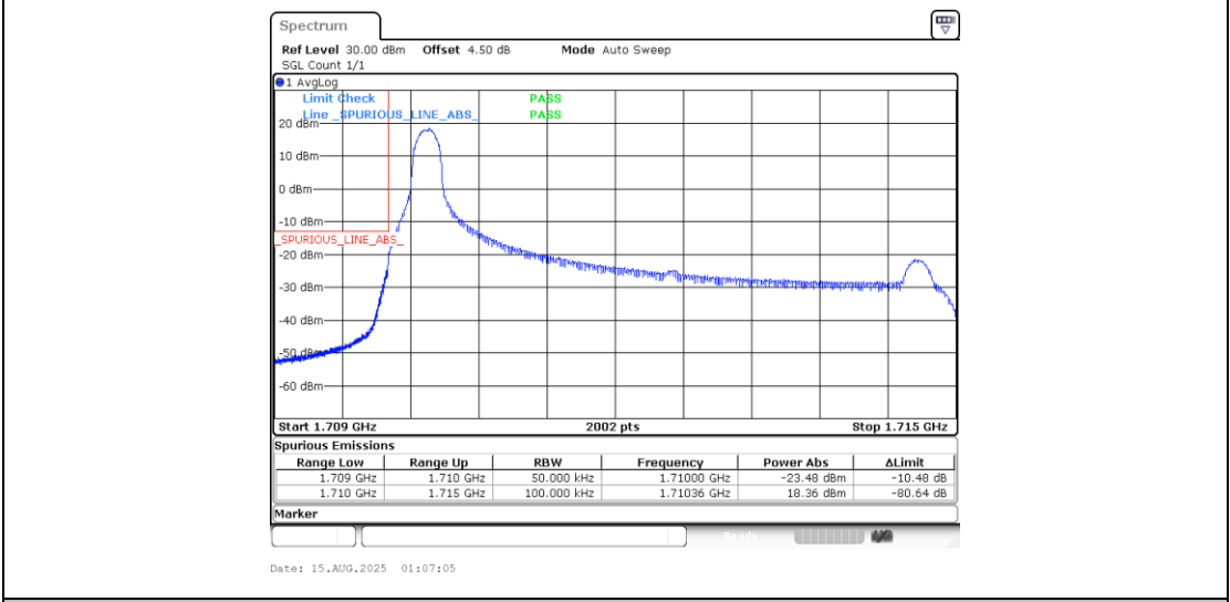
Band4_5MHz_16QAM_19975_1RB#0
