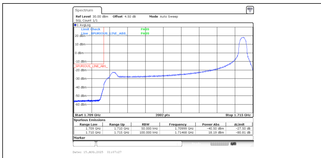
Band4_5MHz_16QAM_19975_1RB#24
