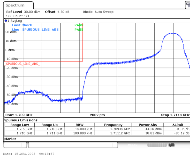
Band4_1.4MHz_16QAM_19957_1RB#5
