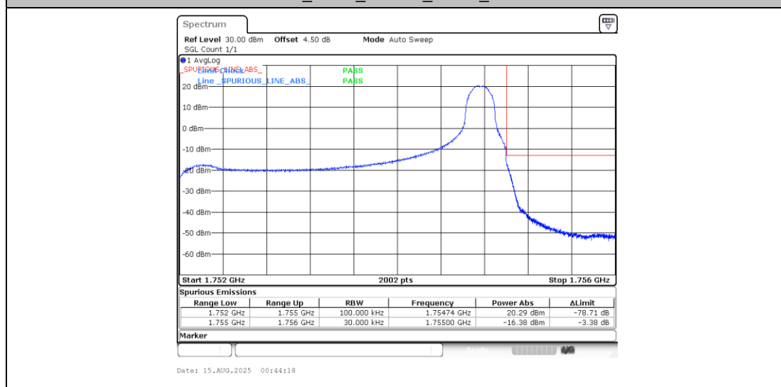
Band4_3MHz_QPSK_20385_1RB#14
