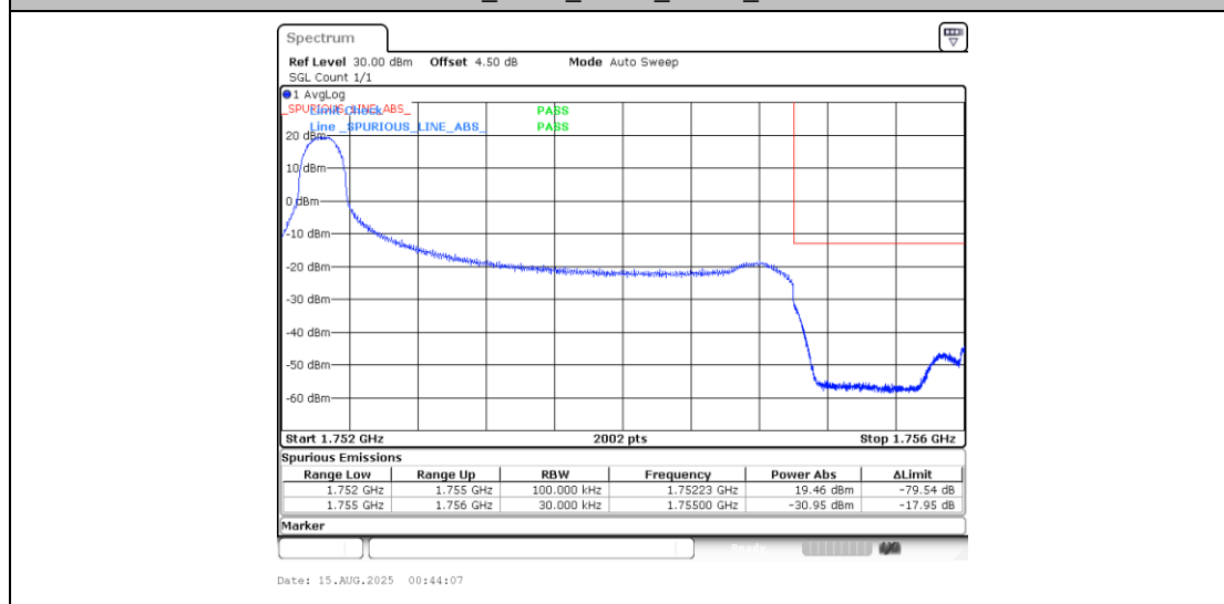
Band4_3MHz_16QAM_20385_1RB#0
