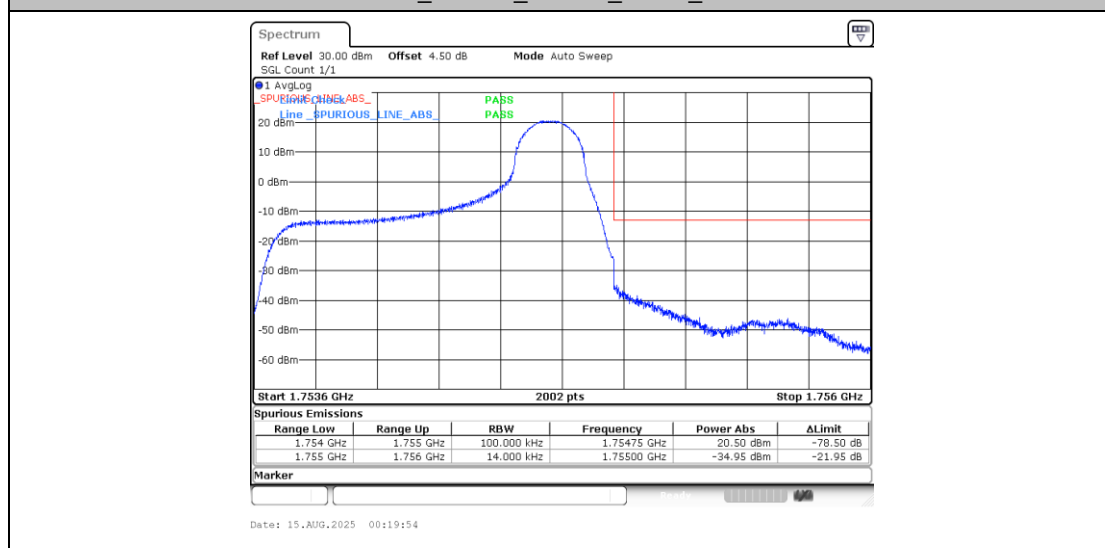
Band4_1.4MHz_QPSK_20393_1RB#5
