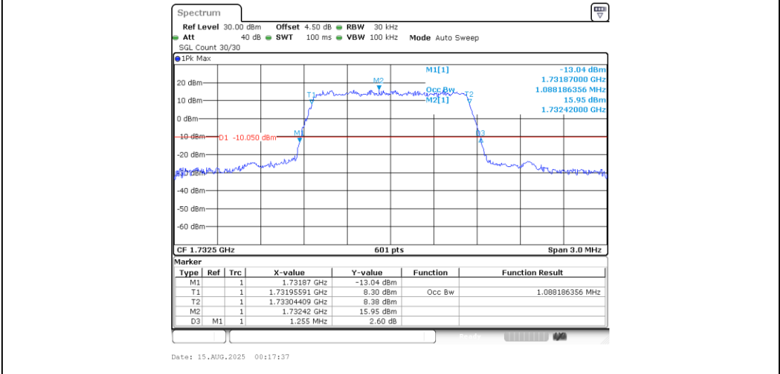
Band4-1.4MHz-QPSK-20175-6RB#0-PASS
