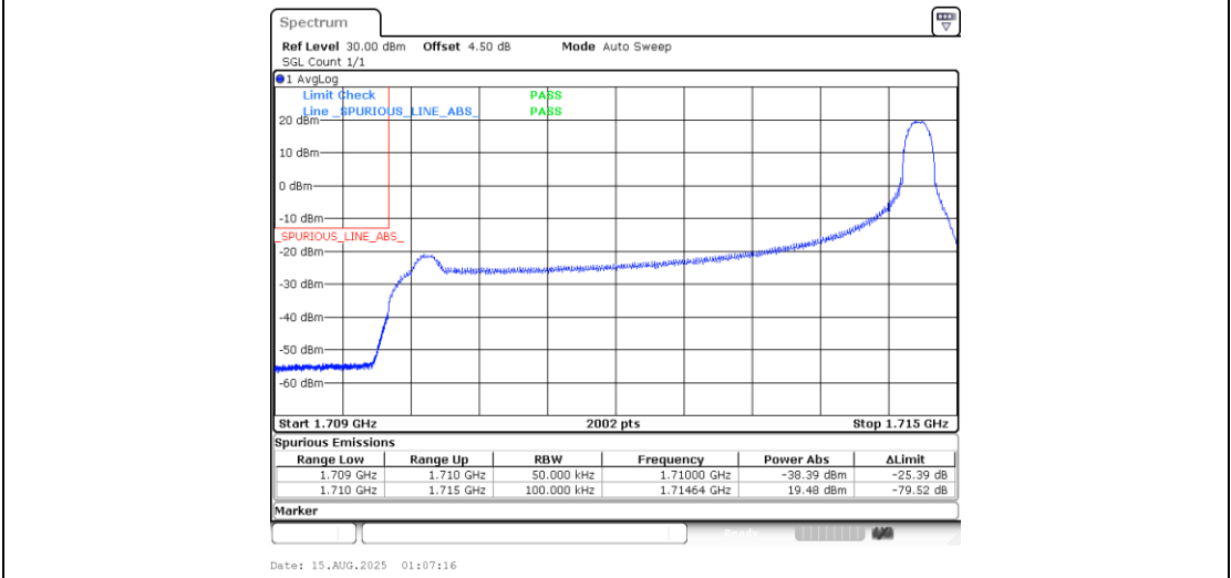
Band4_5MHz_QPSK_19975_1RB#24
