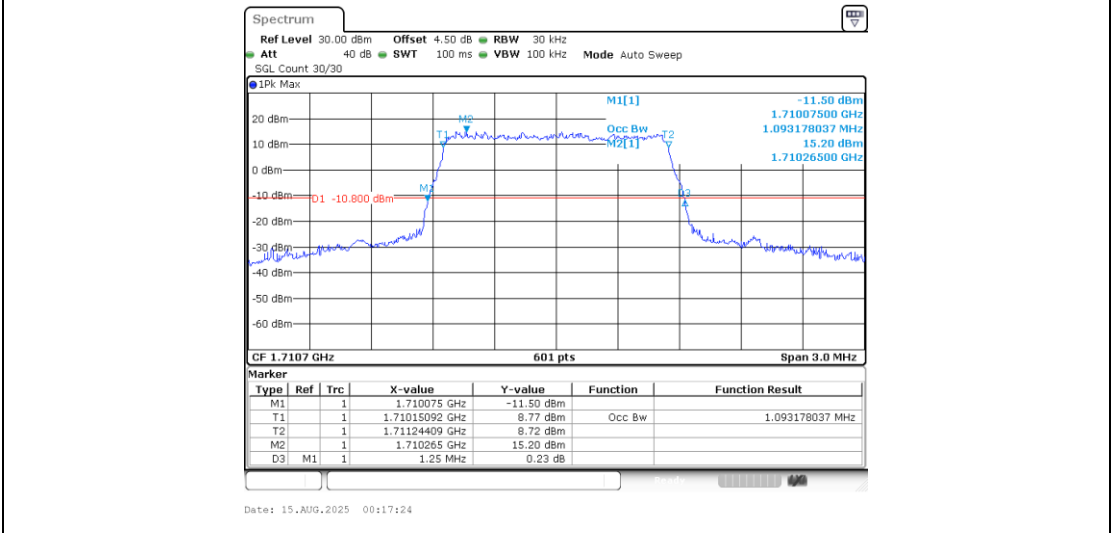
Band4-1.4MHz-16QAM-19957-6RB#0-PASS
