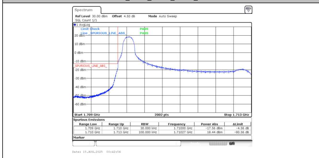
Band4_3MHz_16QAM_19965_1RB#0
