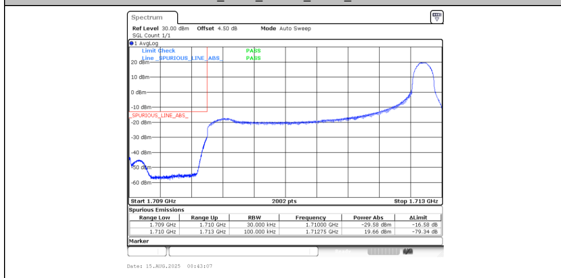
Band4_3MHz_QPSK_19965_1RB#14
