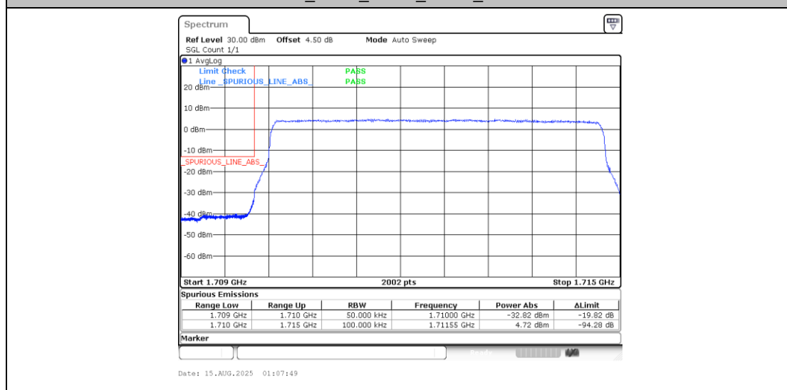
Band4_5MHz_16QAM_19975_25RB#0
