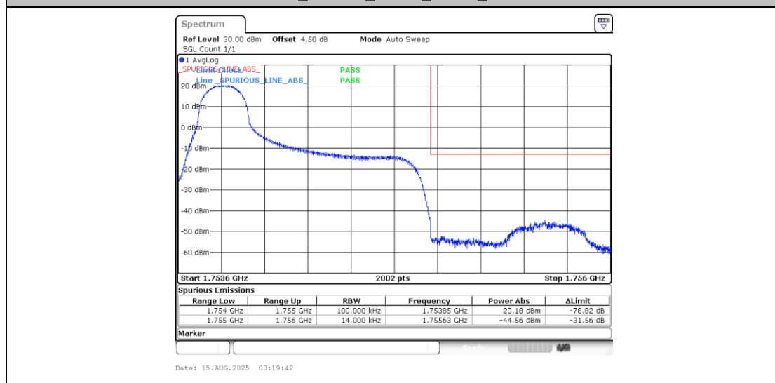
Band4_1.4MHz_16QAM_20393_1RB#0
