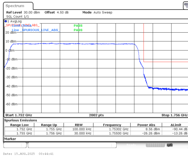
Band4_3MHz_QPSK_20385_15RB#0
