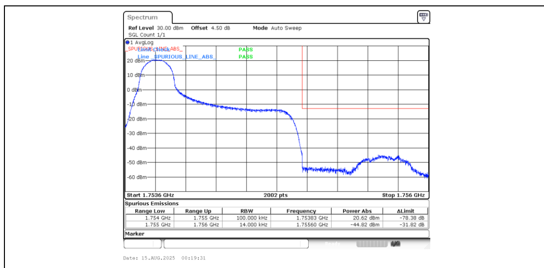
Band4_1.4MHz_QPSK_20393_1RB#0
