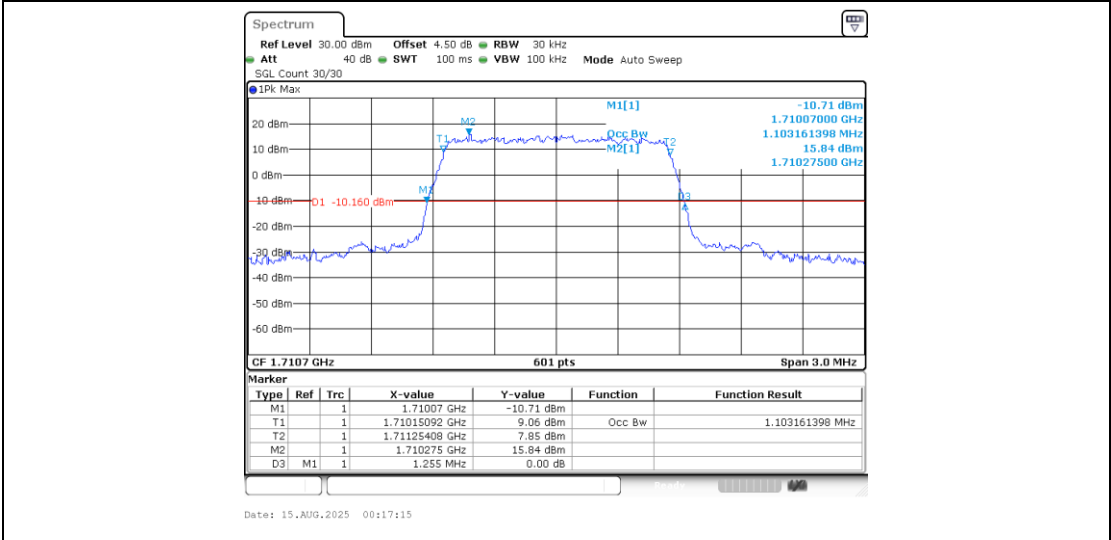
Band4-1.4MHz-QPSK-19957-6RB#0-PASS
