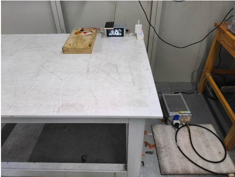
Description: 7.11. AC Conducted Emissions Test Setup for 30MHz ~ 1GHz
