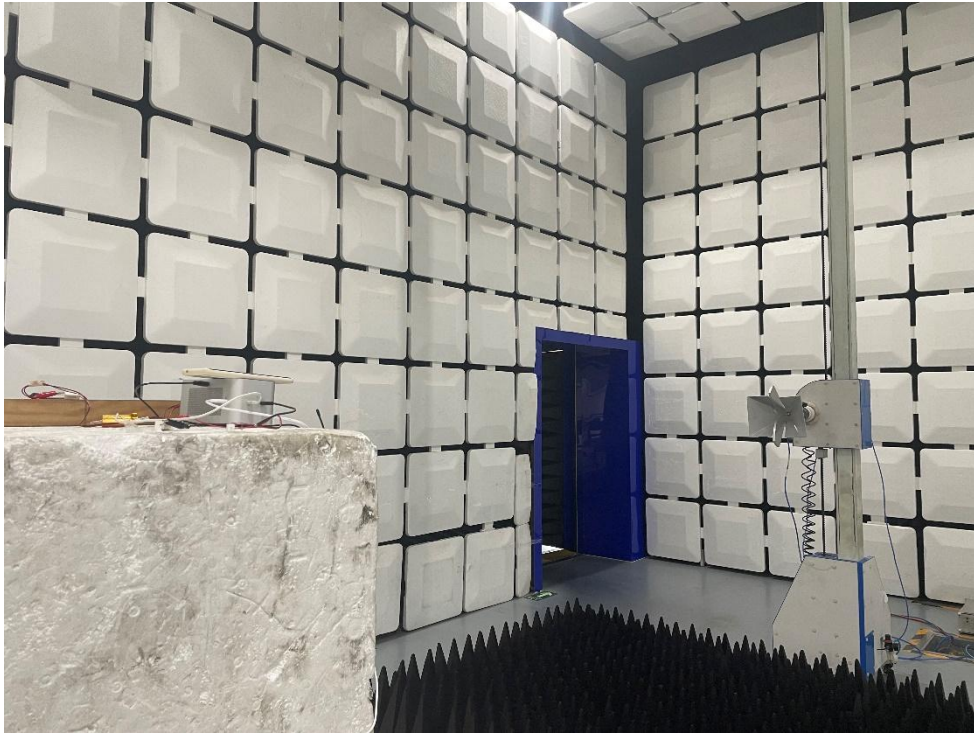
Description: Radiated Emission Test Setup for 1GHz ~ 25GHz
