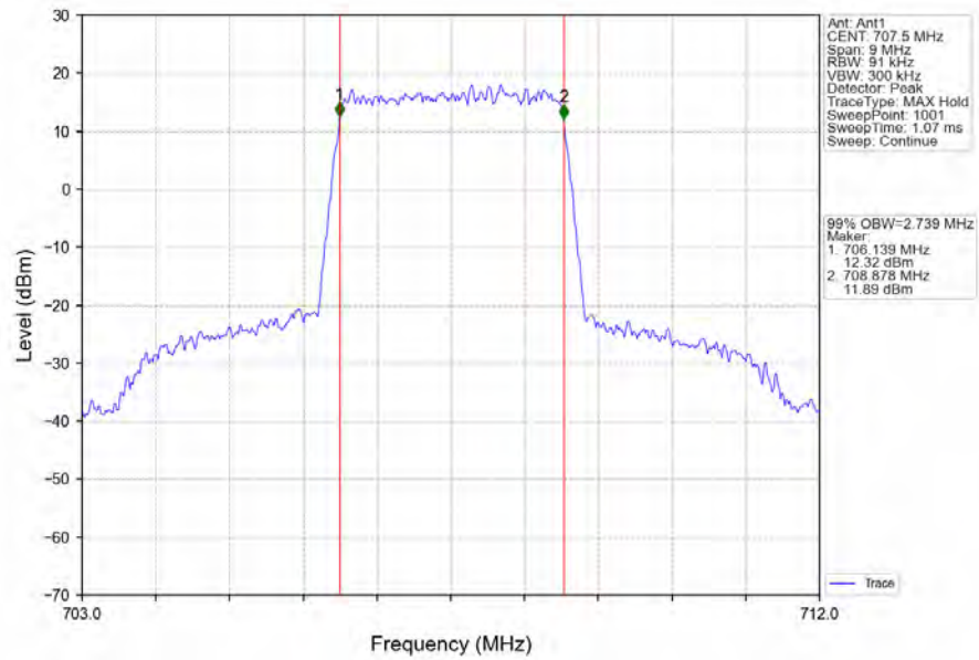
Band12_3MHz_QPSK_MCH_707.5MHz_RB_15_0_NTNV
