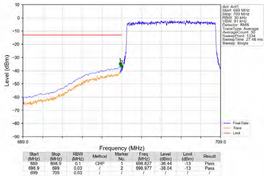
Band12 10MHz 16QAM LCH 704MHz RB 50 0 NTNV
