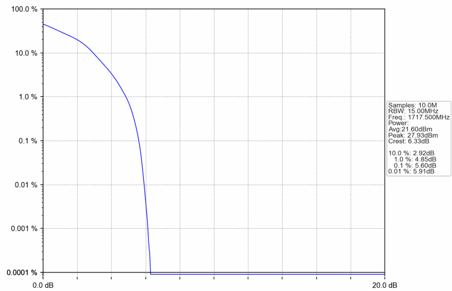
Band66_15MHz_16QAM_LCH_1717.5MHz_RB_75_0_NTNV
