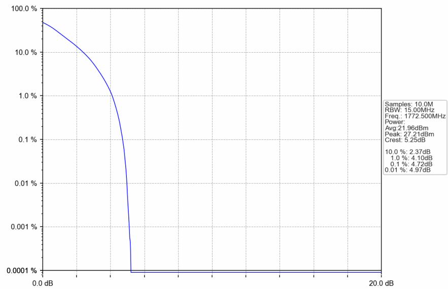
Band66_15MHz_QPSK_HCH_1772.5MHz_RB_75_0_NTNV
