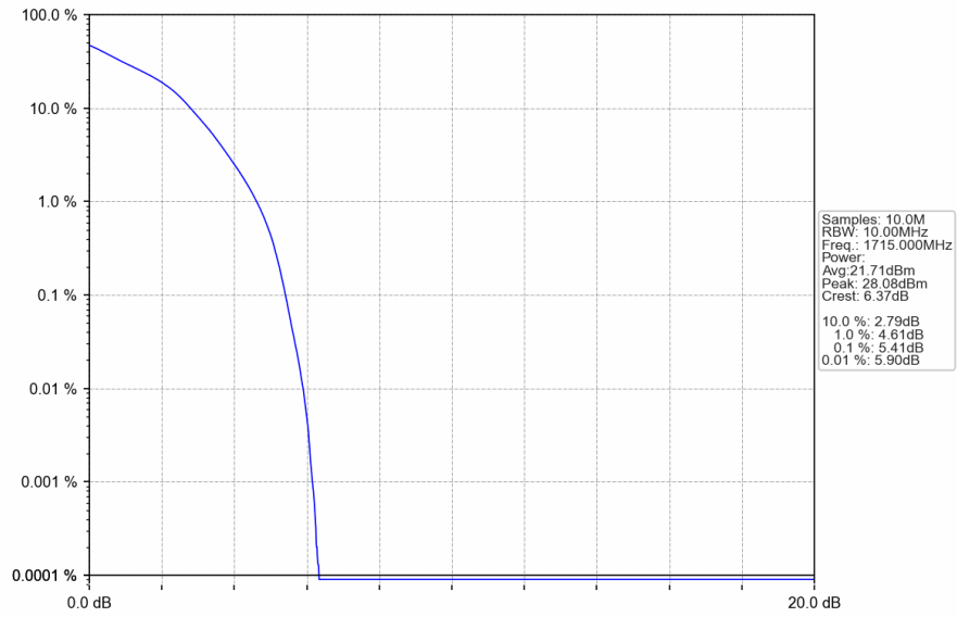
Band66_10MHz_16QAM_LCH_1715MHz_RB_50_0_NTNV
