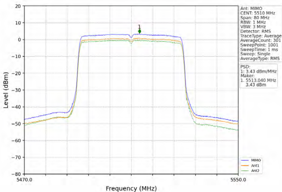
802.11ax(HEW40)_LCH_5510MHz_RU484_Left_MIMO_NTNV
