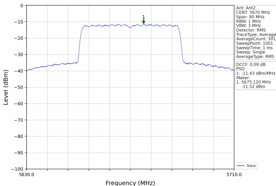
802.11ax(HEW40)_HCH_5670MHz_RU484_Left_MIMO_NTNV
