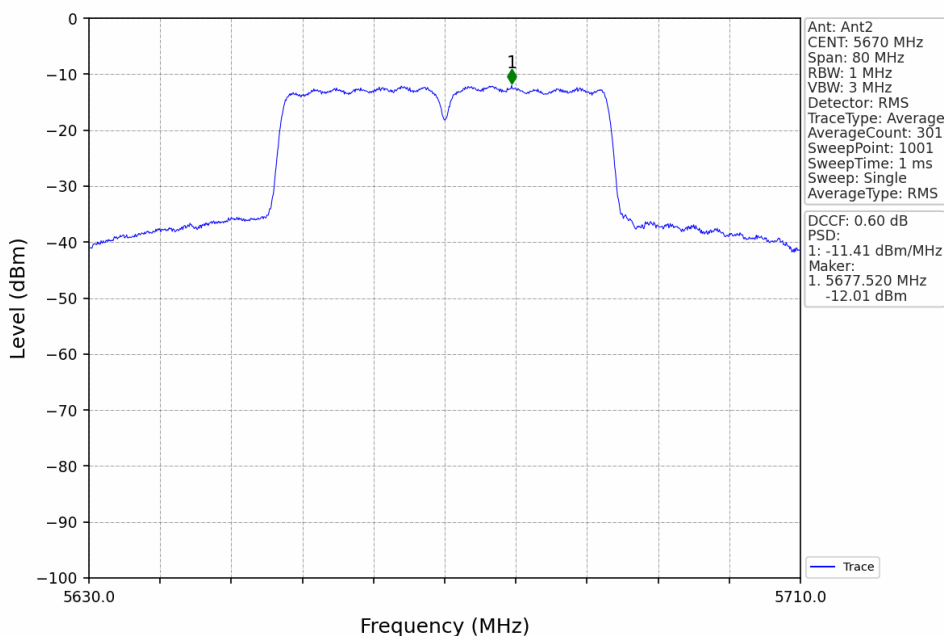
802.11n(HT40)_HCH_5670MHz_MIMO_NTNV
