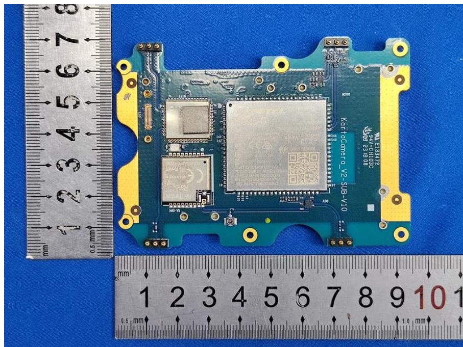
PCB view
