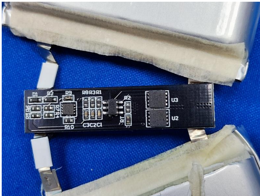
Battery PCB view
