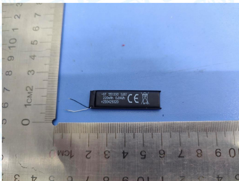
Photo 9 Battery Appearance
