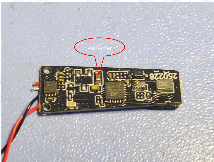
Photo 12 Appearance of PCB ----Left
