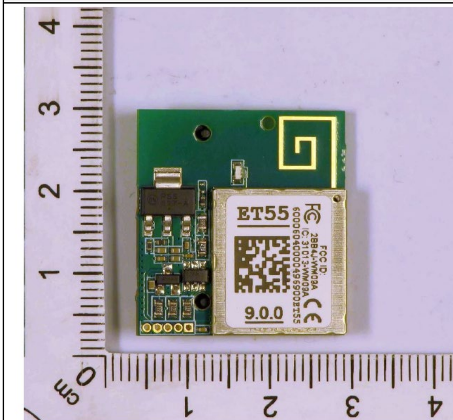
EUT 1 TOP VIEW
