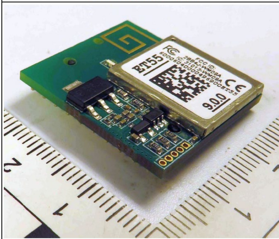
EUT 1 PERSPECTIVE VIEW 1
