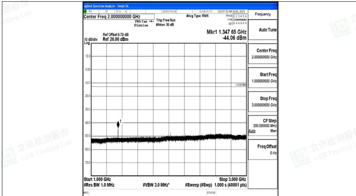
Band71_15MHz_16QAM_133297_1RB#0_1000~3000_1000~3000
