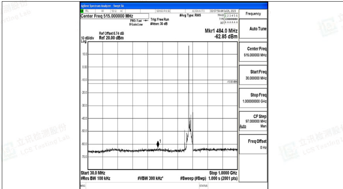
Band71_15MHz_QPSK_133397_1RB#0_30~1000_30~1000
