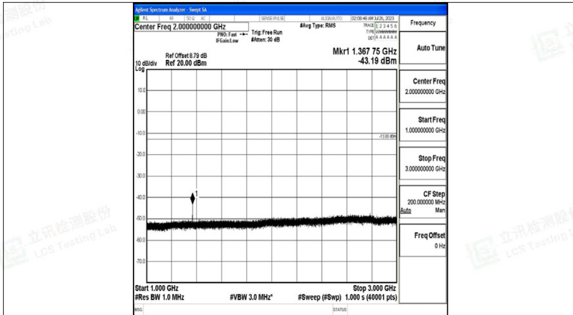
Band71_15MHz_16QAM_133397_1RB#0_1000~3000_1000~3000
