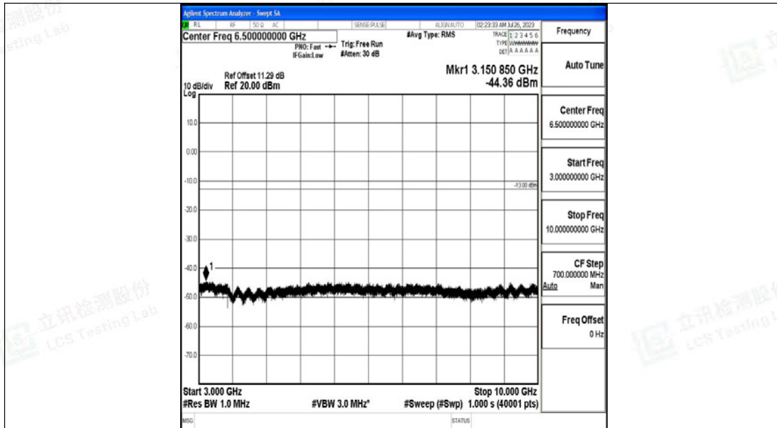
Band71_20MHz_QPSK_133222_1RB#0_3000~10000_3000~10000
