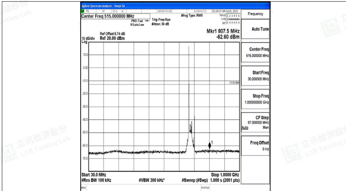
Band71_20MHz_QPSK_133322_1RB#0_30~1000_30~1000
