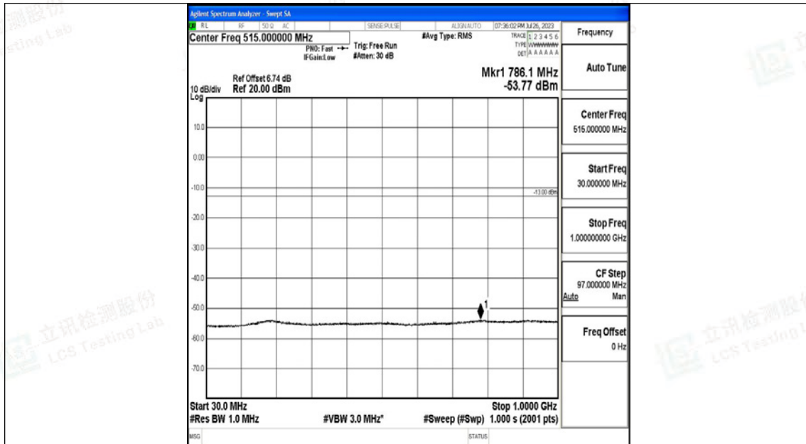
Band66_3MHz_QPSK_132657_1RB#0_30~1000_30~1000
