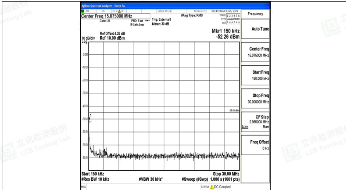
Band41_10MHz_16QAM_40620_1RB#0_0.15~30_0.15~30
