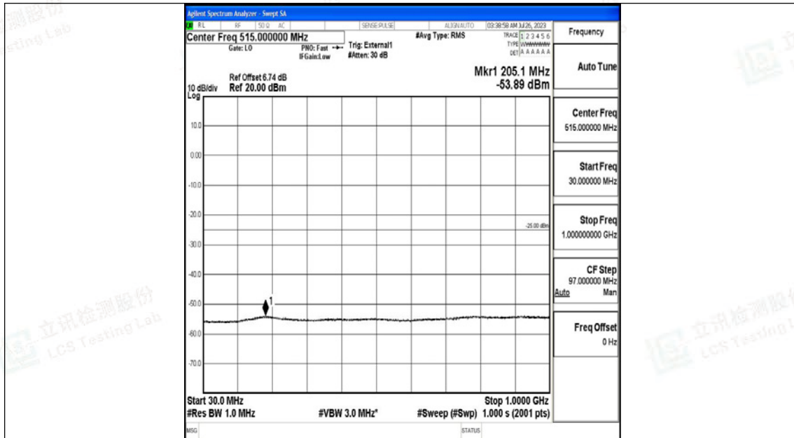
Band41_10MHz_QPSK_40620_1RB#0_30~1000_30~1000
