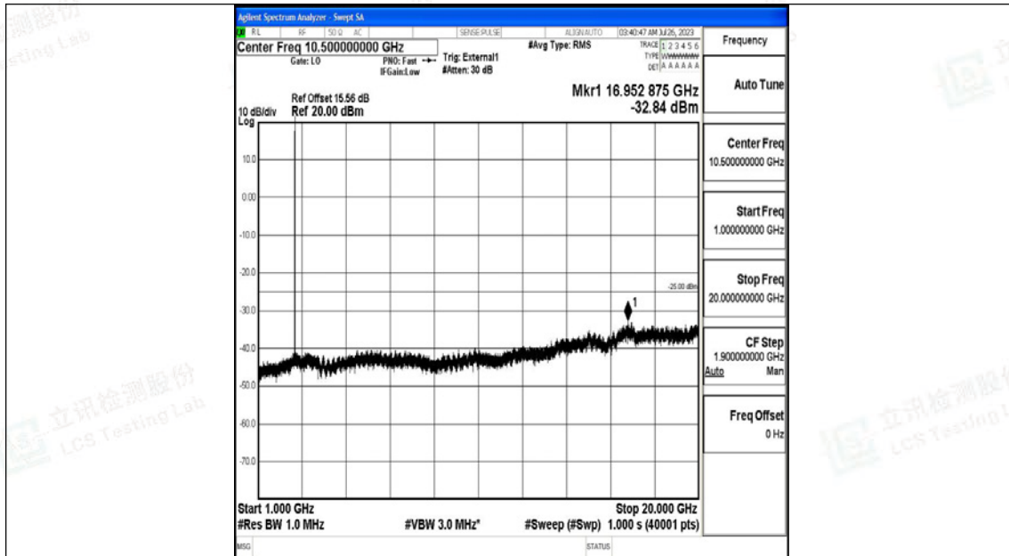
Band41_10MHz_16QAM_40620_1RB#0_1000~20000_1000~20000
