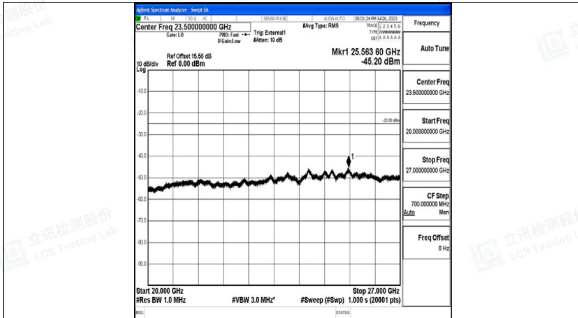
Band41_15MHz_QPSK_39725_1RB#0_20000~27000_20000~27000
