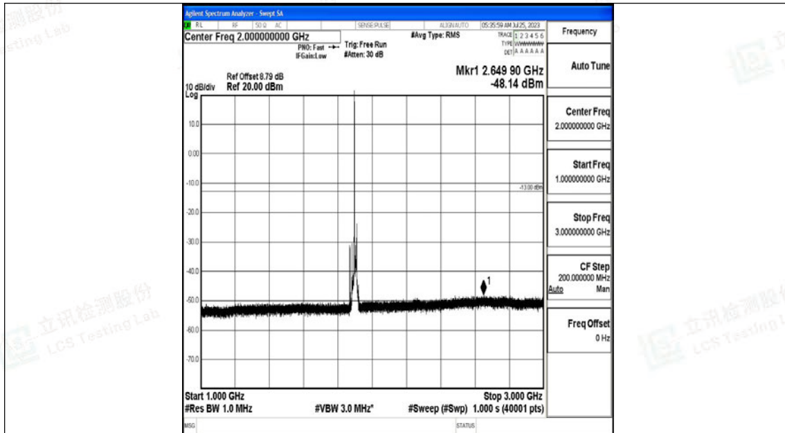
Band2_15MHz_16QAM_19125_1RB#0_1000~3000_1000~3000
