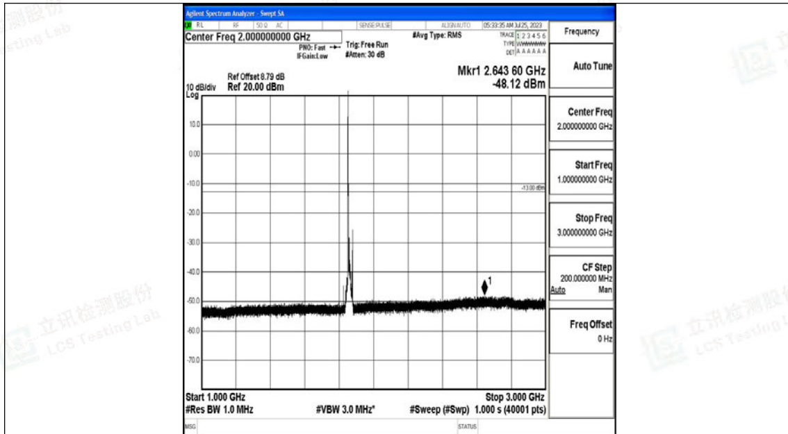
Band2_15MHz_16QAM_18675_1RB#0_1000~3000_1000~3000
