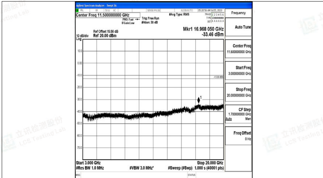
Band2_10MHz_QPSK_19150_1RB#0_3000~20000_3000~20000
