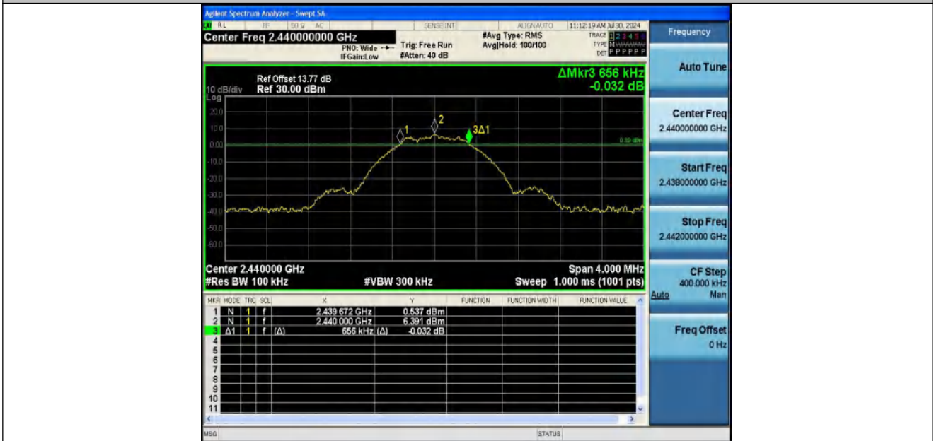
BLE_1M-Ant1-2440-PASS
