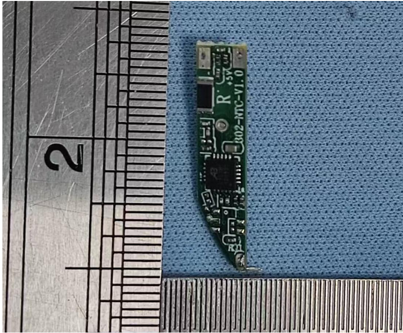
Internal Photos(Left Earphone)
