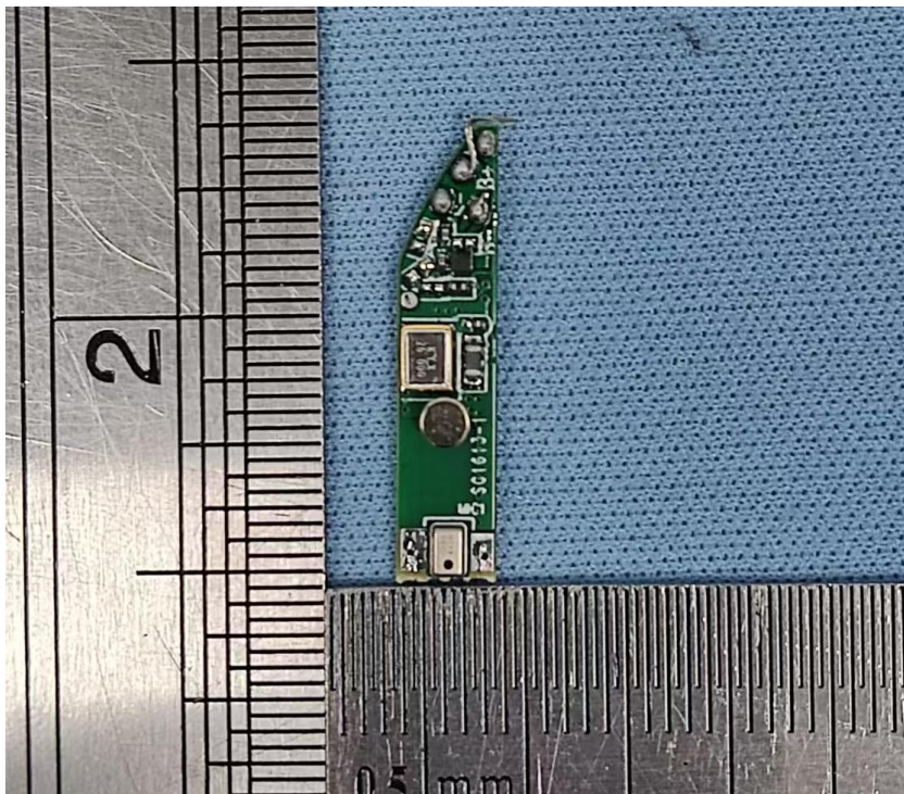
Internal Photos(Left Earphone)
