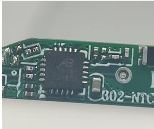
Internal Photos(Left Earphone)
