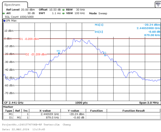
GFSK_Middle 0.879MHz
