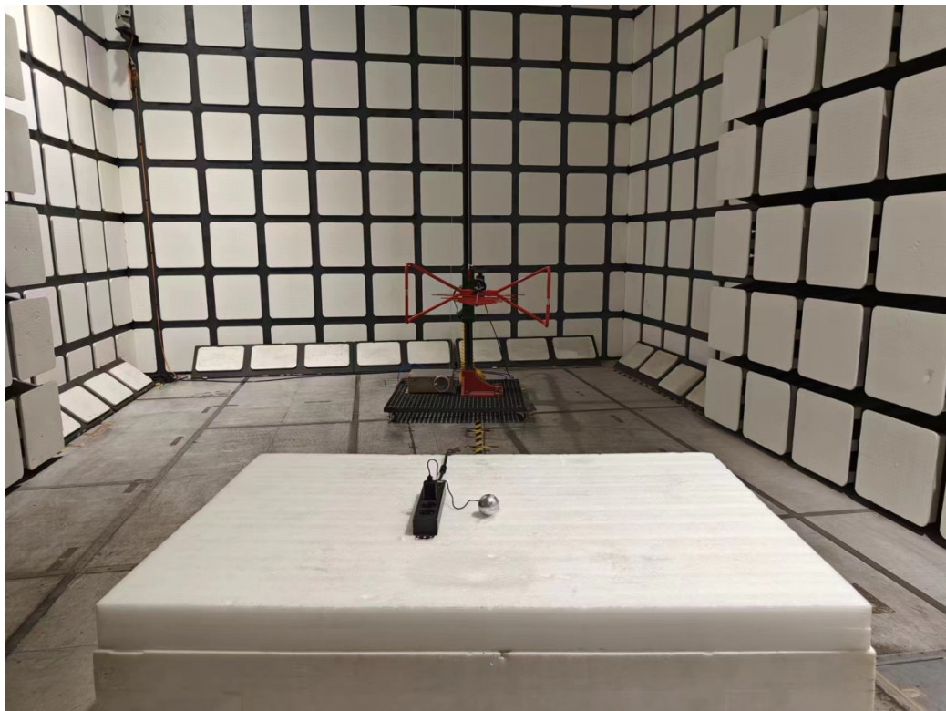
Radiated Emissions View (30-1000 MHz)
