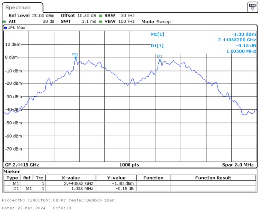
GFSK_Middle 1.005MHz
