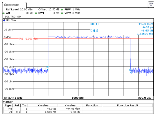
\pi/4 -DQPSK_Hopping_2DH3 1.656ms
