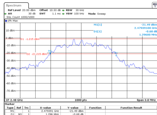
\pi/4 -DQPSK_High 1.296MHz
