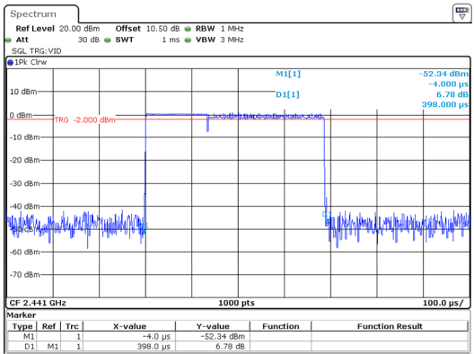
\pi/4 -DQPSK_Hopping_2DH1 0.398ms
