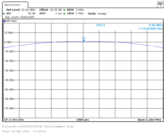
GFSK_Middle 0.83dBm
