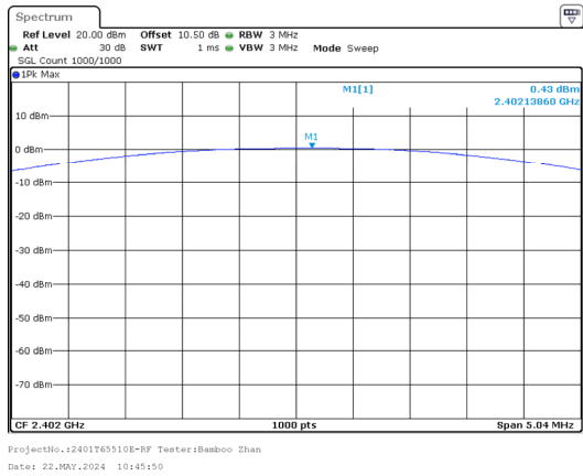
GFSK_Low 0.43dBm
