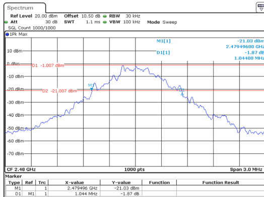
GFSK_High 1.044MHz
