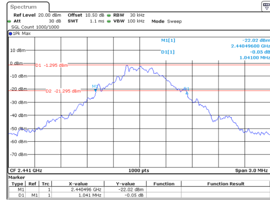
GFSK_Middle 1.041MHz
