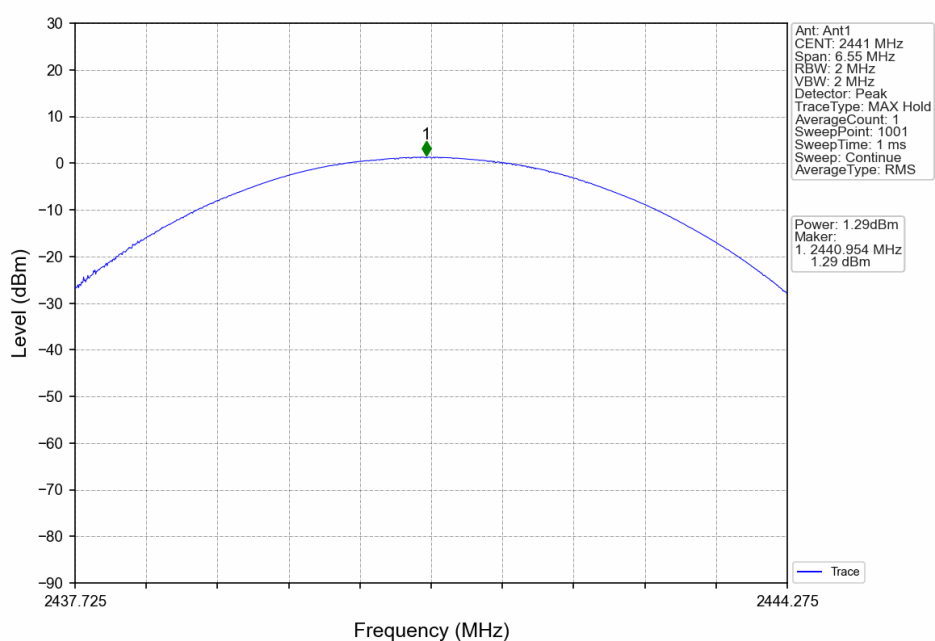
8-DPSK 3DH5 MCH 2441MHz Ant1 NTN
