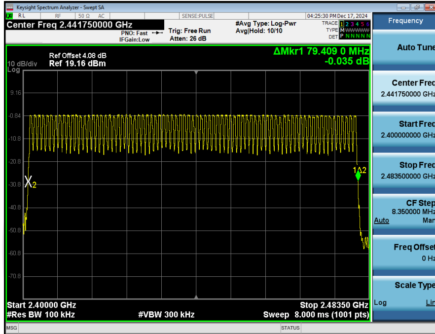
Number_of_Hopping_Channel_(Hopping)_NVNT_ANT1_1-DH1_Hopping
