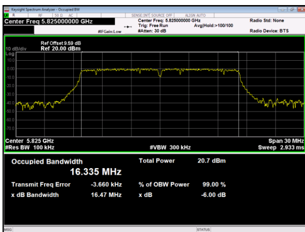
(802.11a)99%&6DB Bandwidth plot on channel 165
