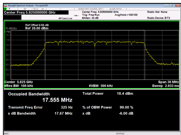
(802.11n20)99%&6DB Bandwidth plot on channel 165
