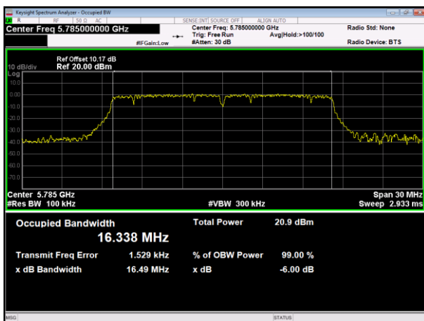
(802.11a)99%&6DB Bandwidth plot on channel 157
