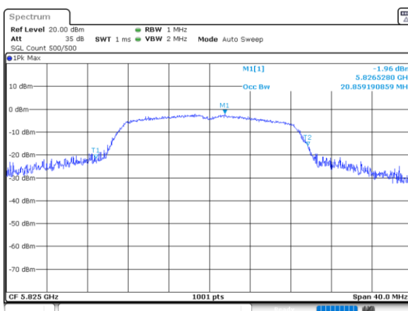
(802.11 n20) 99%Bandwidth plot on channel 165
