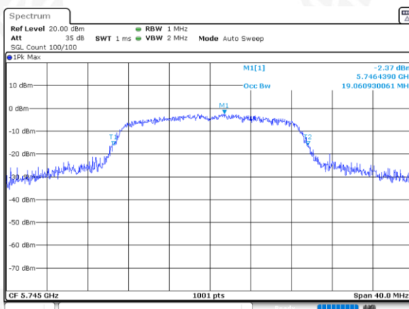
(802.11 n20) 99%Bandwidth plot on channel 149
