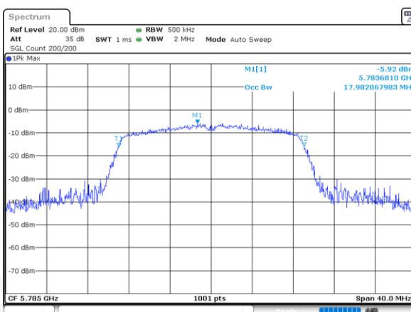
(802.11 n20) 99%Bandwidth plot on channel 157
