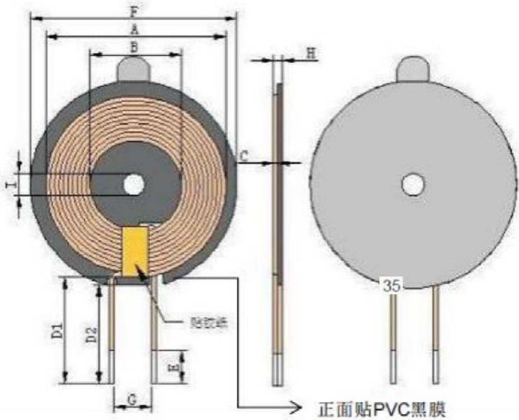
Outside Diagra:
