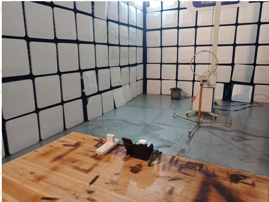
Photo of Radiation Emission Test (below 30MHz)
