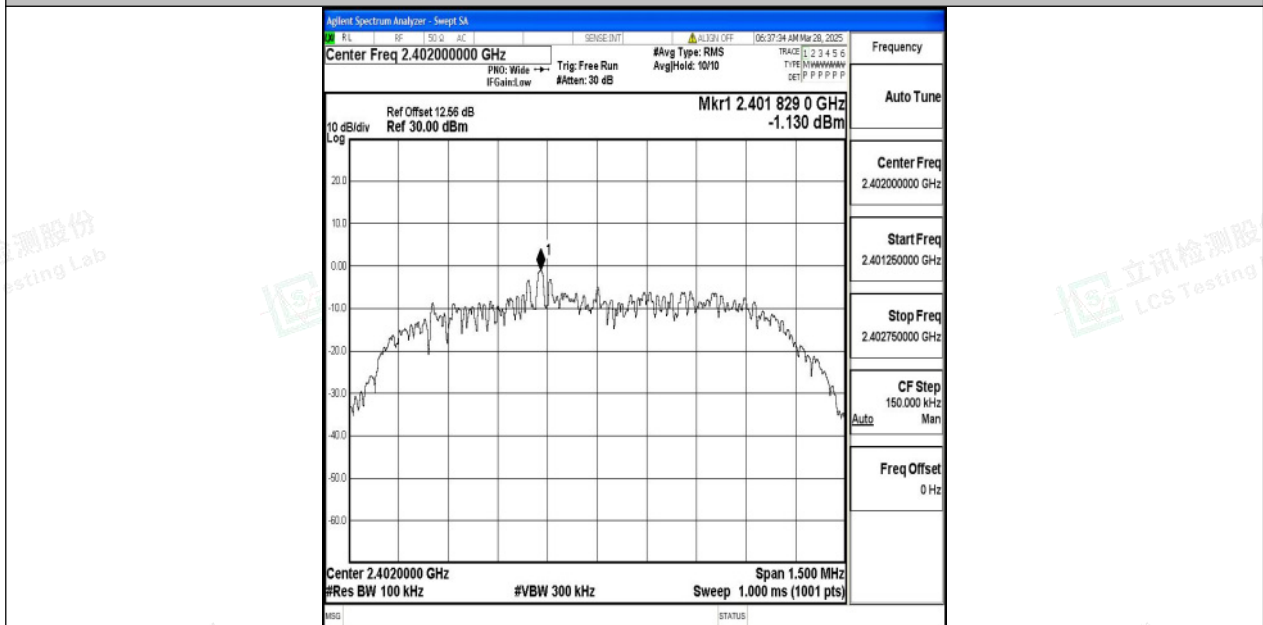
2DH5-Ant1-2402-0~Reference-PASS
