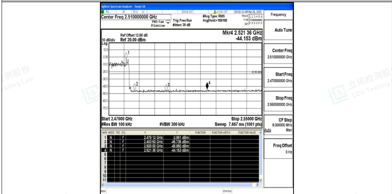
2DH5-Ant1-Hop_2480-PASS
