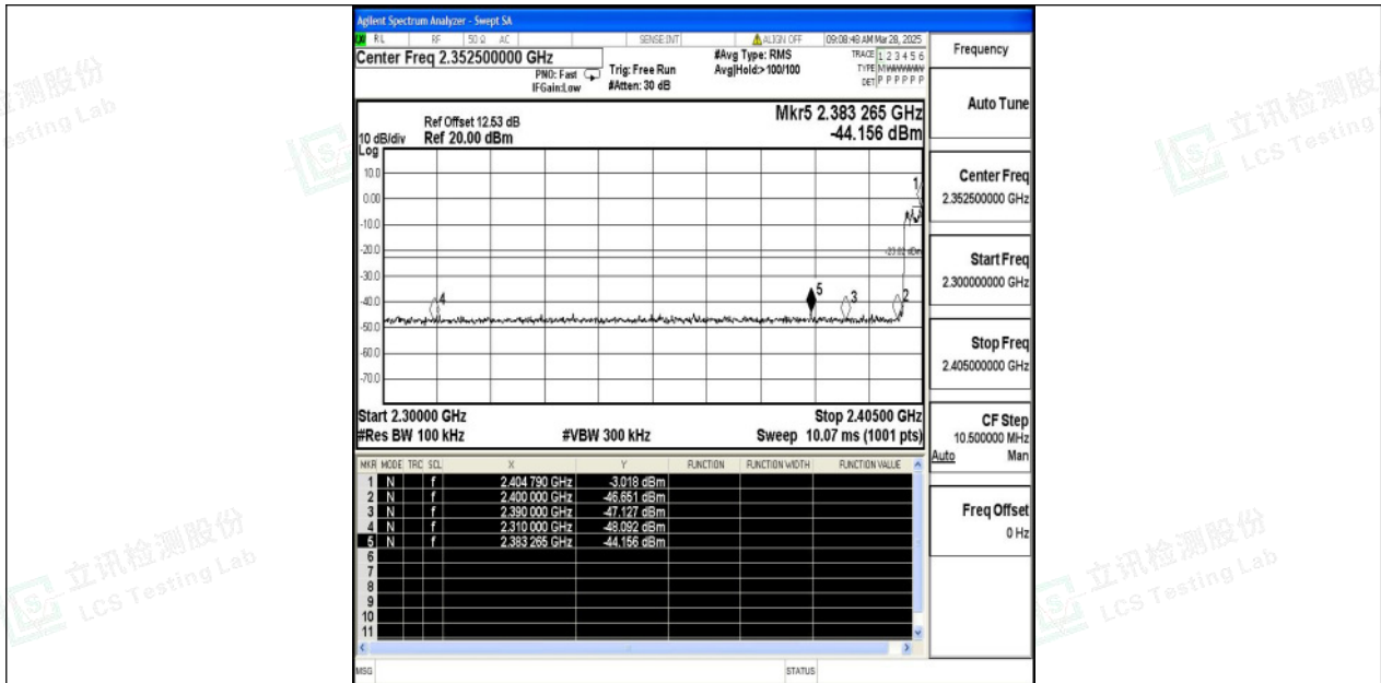
3DH5-Ant1-Hop_2402-PASS
