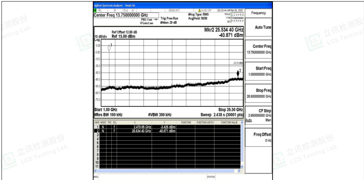
DH5-Ant1-2480-1000~26500-PASS
