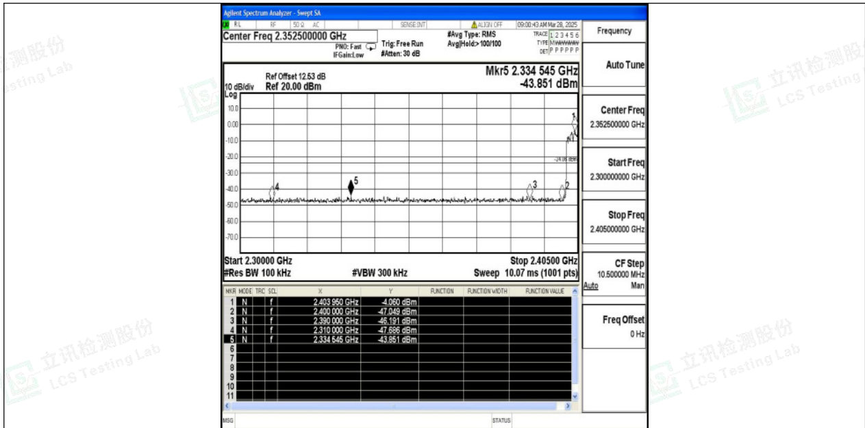
2DH5-Ant1-Hop_2402-PASS
