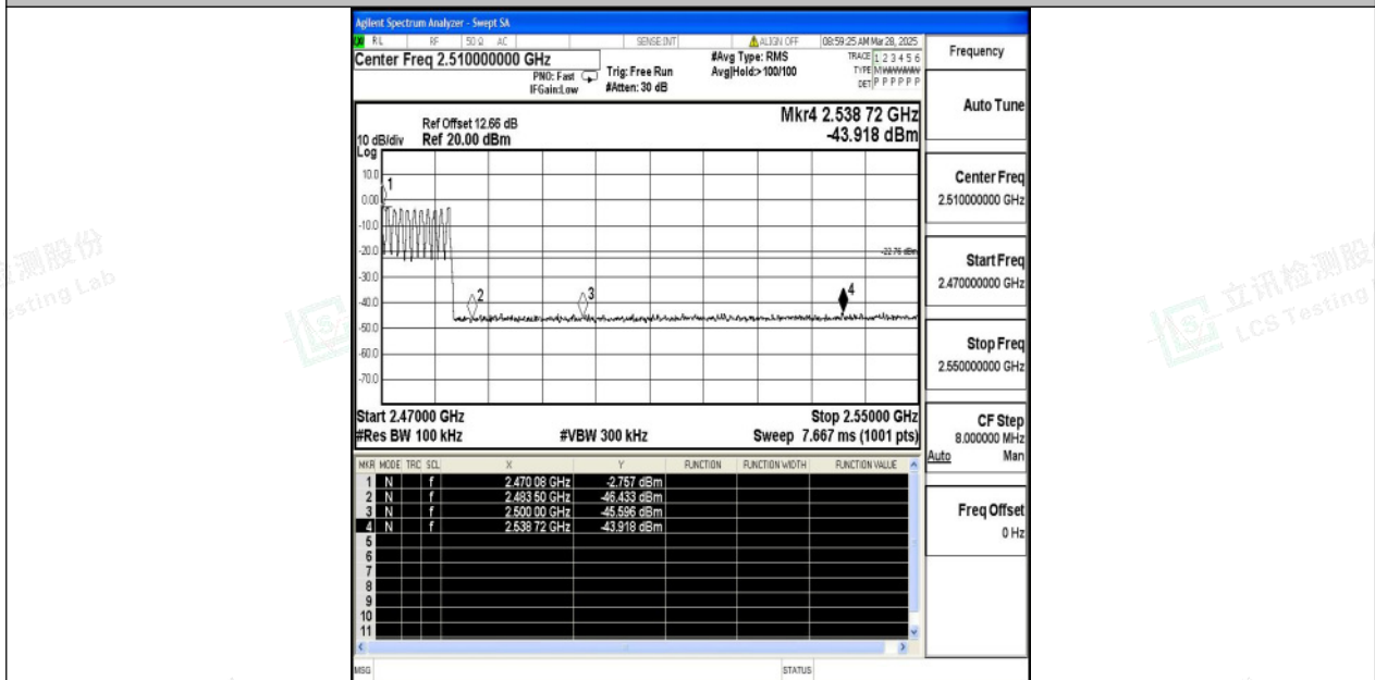
DH5-Ant1-Hop_2480-PASS
