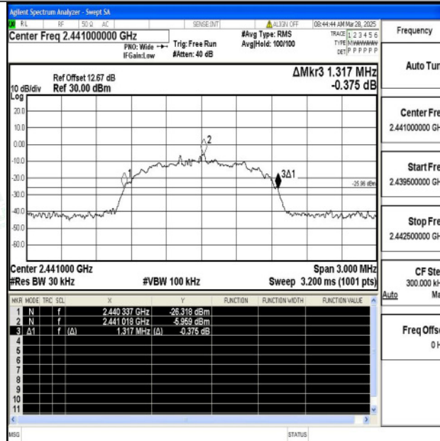
3DH5-Ant1-2441
