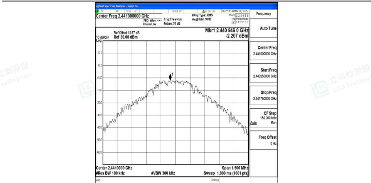
DH5-Ant1-2441-0~Reference-PASS
