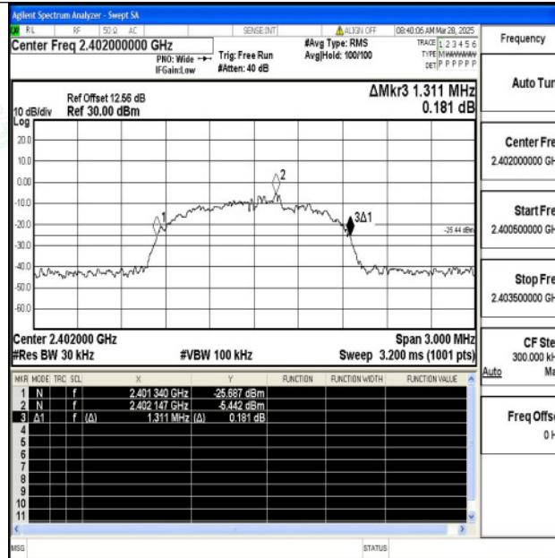
3DH5-Ant1-2402
