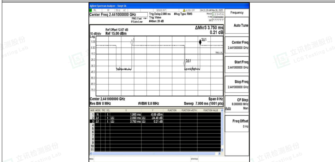
NTNV-DH5-Ant1-2441
