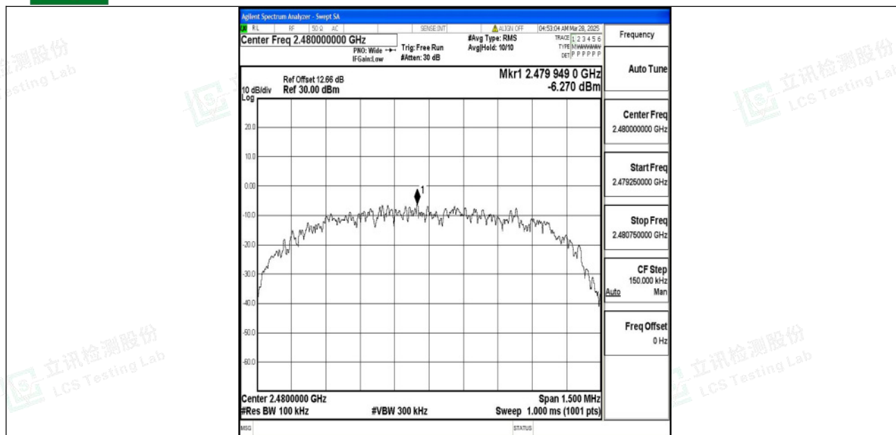
3DH5-Ant1-2480-0~Reference-PASS
