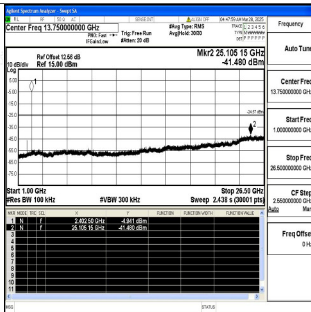
3DH5-Ant1-2402-1000~26500-PASS
