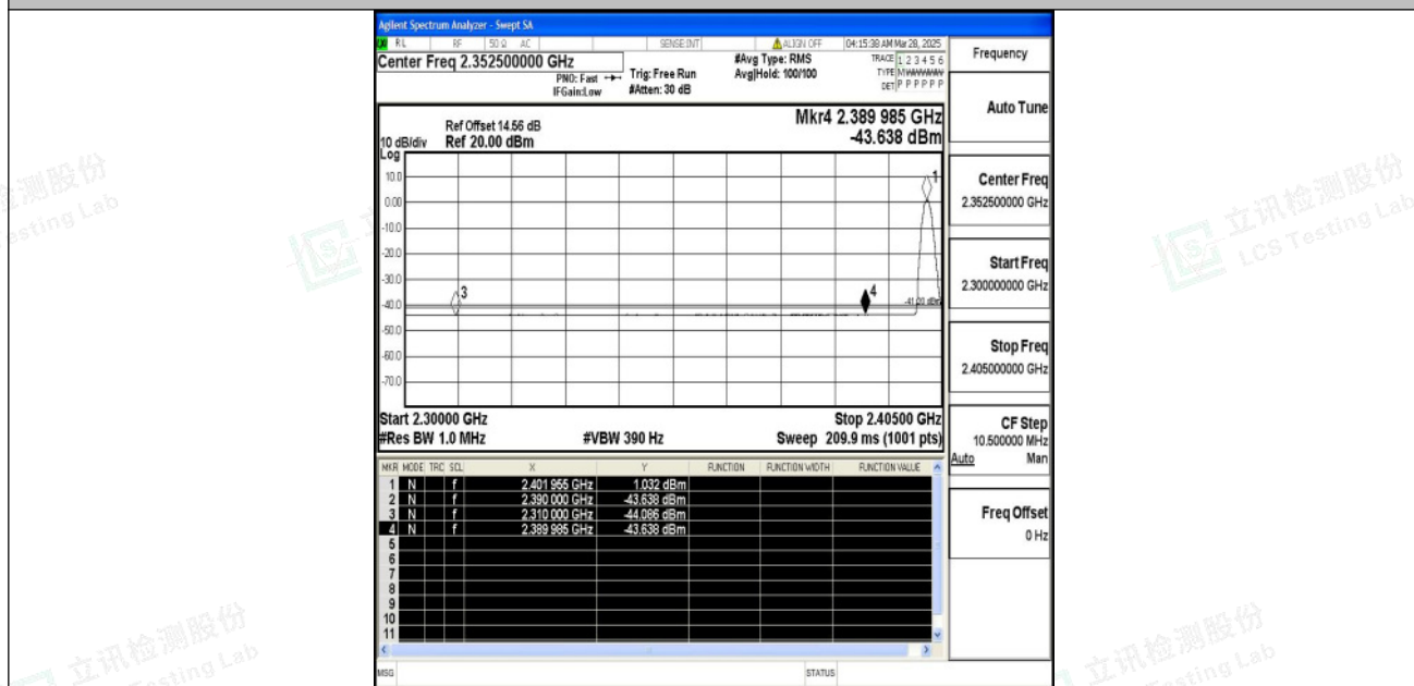
DH5-Ant1-2402-PASS
