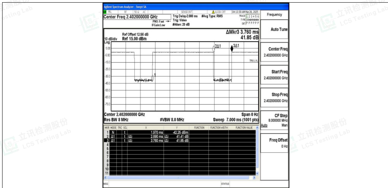
NTNV-DH5-Ant1-2402
