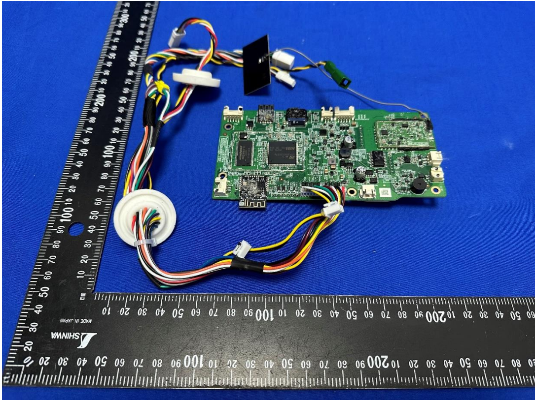
(24) EUT Photo (2.4G WIFI#1 Transceiver)
