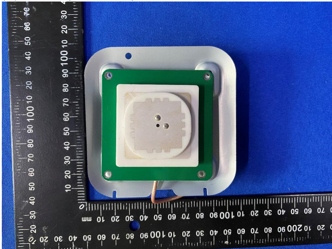
(36) EUT Photo (GNSS Antenna)
