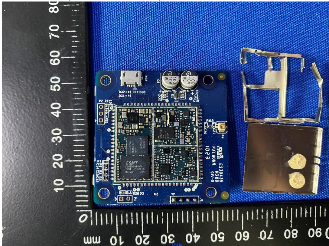
(34) EUT Photo (WCDMA / LTE Module)
