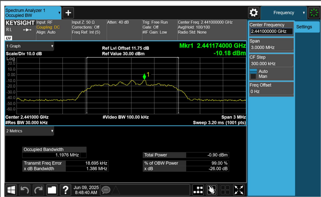
2DH5_Ant1_2441
