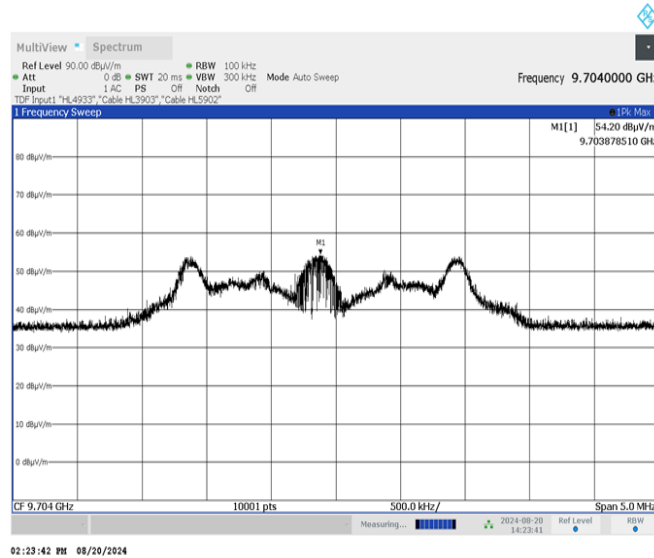
Plot 7.3.17 Radiated emission measurements at the fourth harmonic of high carrier frequency
