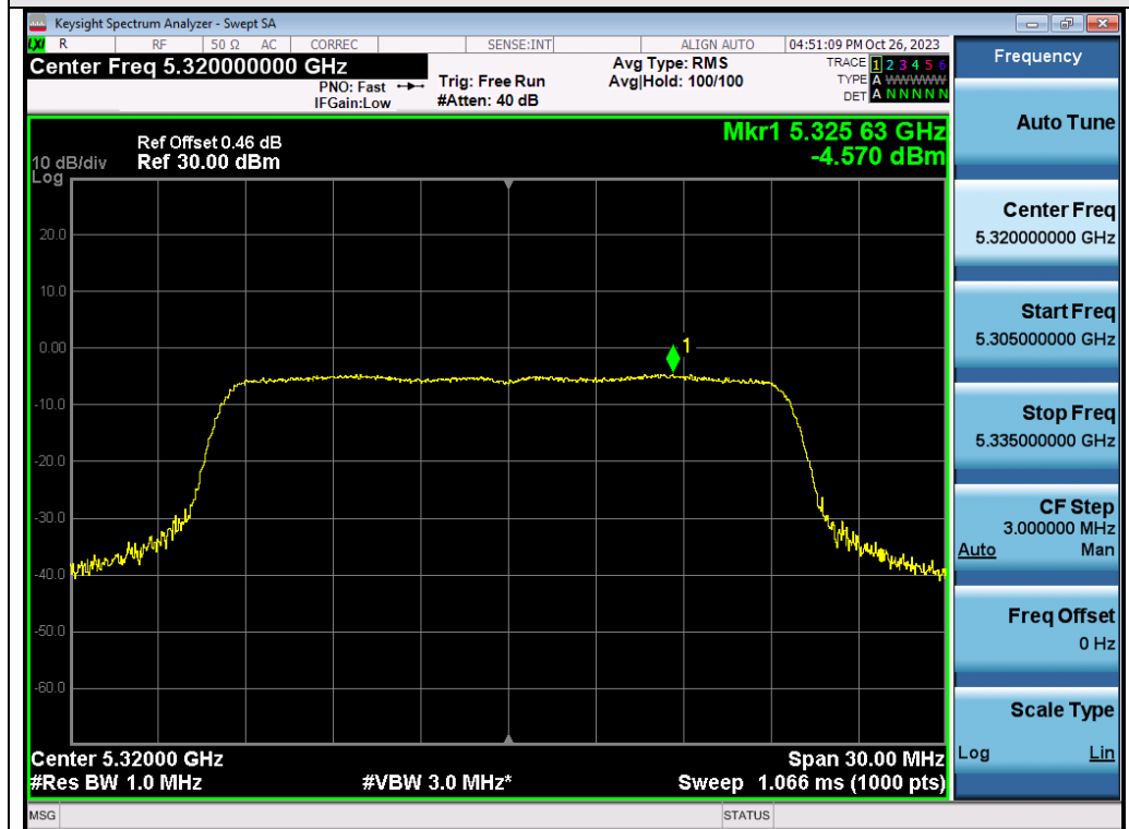
Test_Graph_802.11ax20_ANT1_5320_MCS0_PSD
