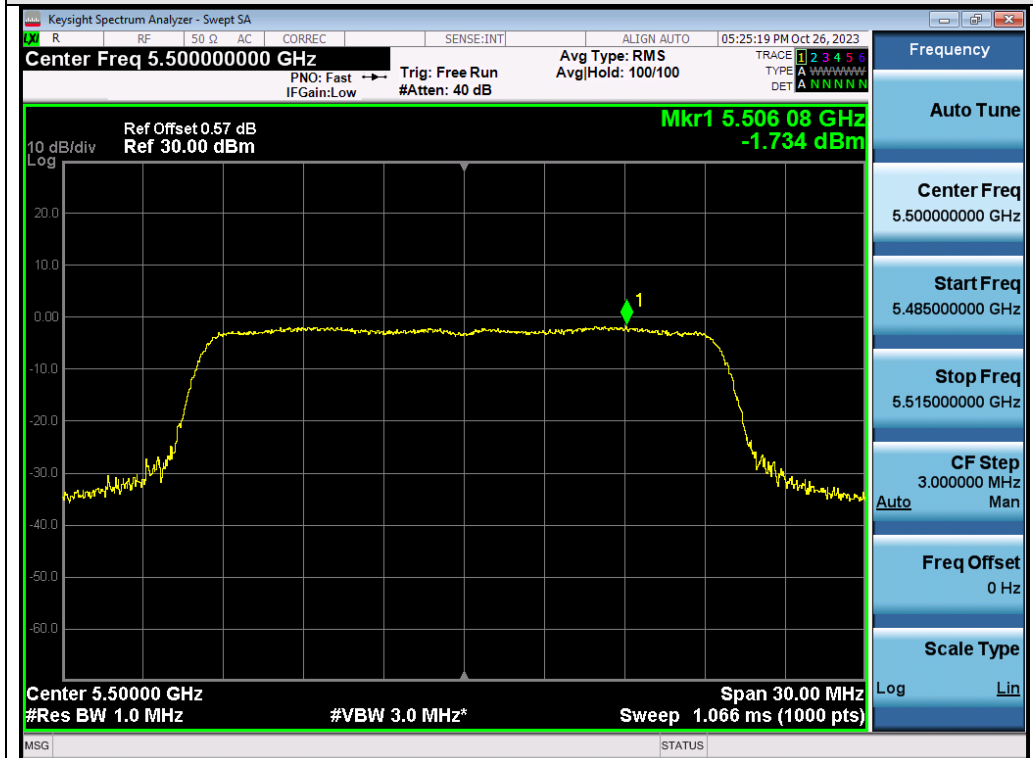
Test_Graph_802.11ax20_ANT1_5500_MCS0_OBW
