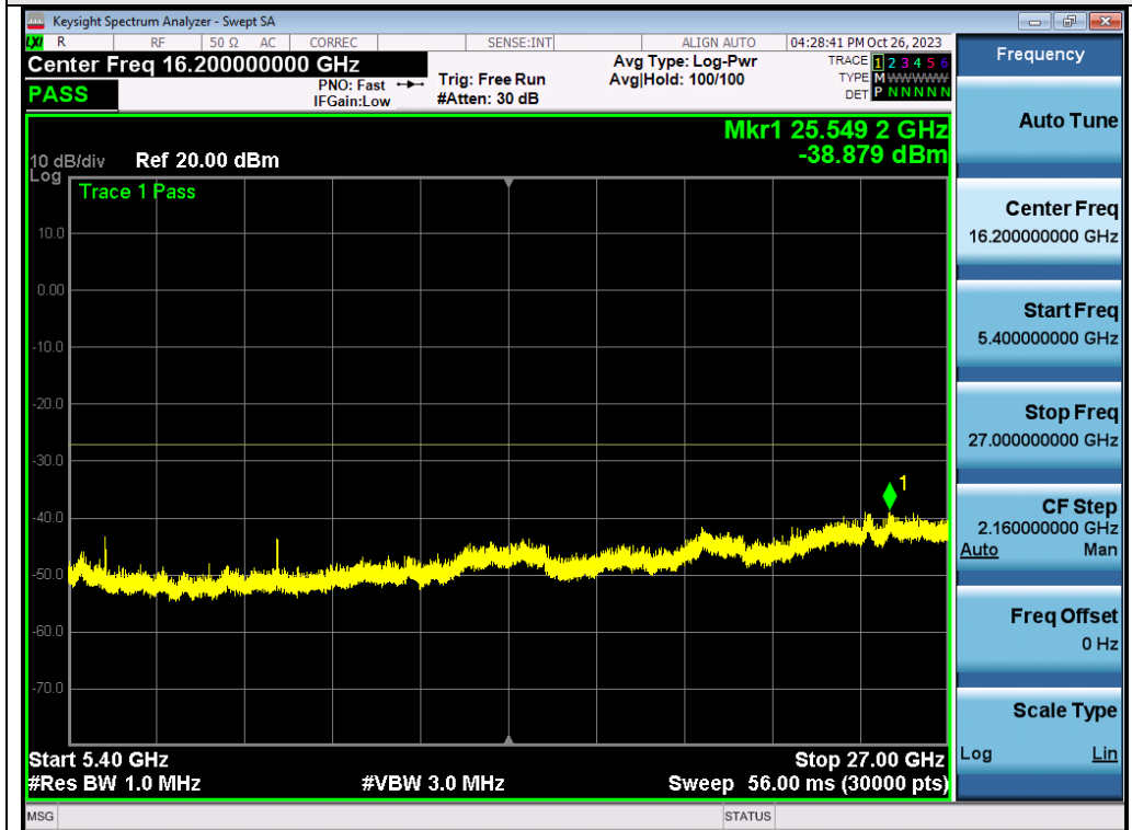
Test_Graph_802.11a_ANT1_5260_6Mbps_Frequency Band 4
