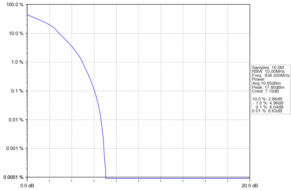
Band5_10MHz_16QAM_MCH_836.5MHz_RB_27_0_NTNV
