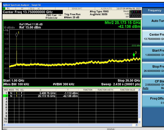
11G-Ant1-2437-0~Reference--3.21
