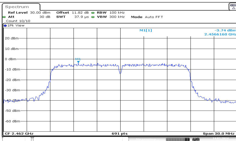
11N20SISO-Ant1-2462-0~Reference--3.74
