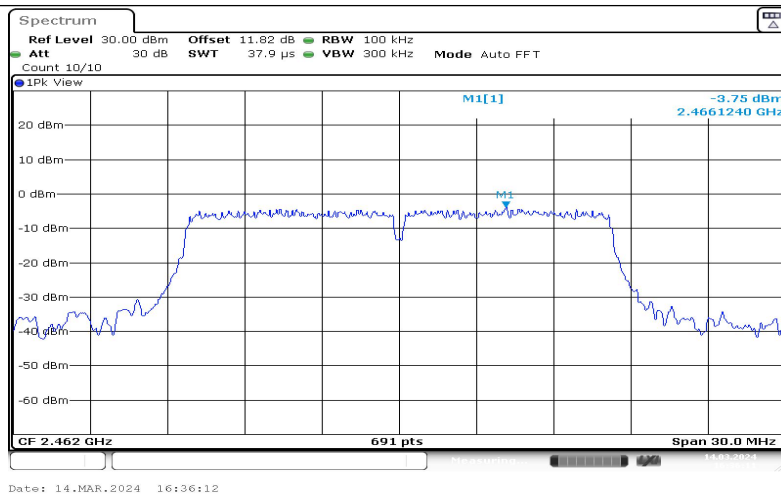
11G-Ant1-2462-0~Reference--3.75
