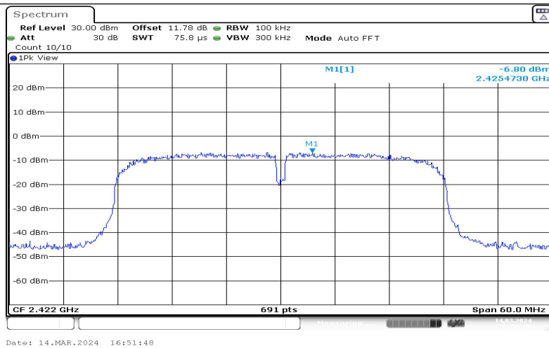
11N40SISO-Ant1-2422-0~Reference--6.80
