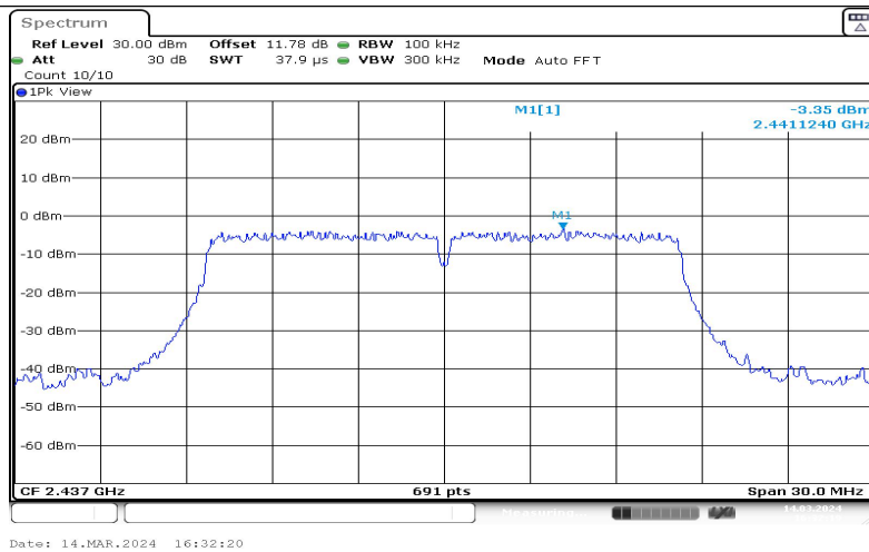
11G-Ant1-2437-0~Reference--3.35
