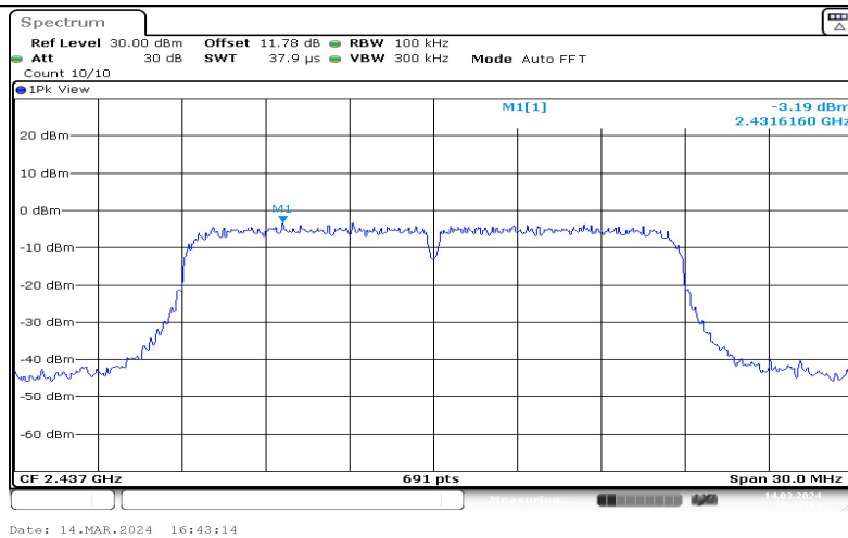
11N20SISO-Ant1-2437-0~Reference--3.19
