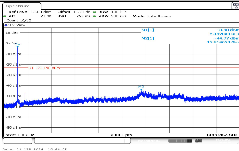
11N20SISO-Ant1-2437-1000~26500--3.19
