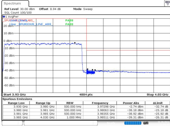
n77(3700-3980) SCS=30kHz DFT_QPSK BW=50MHz HighChannel=663666 RB=128@0
