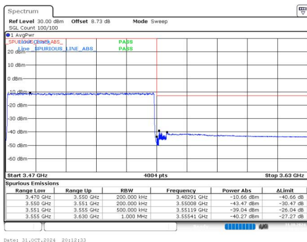
n77(3450-3550) SCS=30kHz DFT_64QAM BW=80MHz HighChannel=634000 RB=216@0
