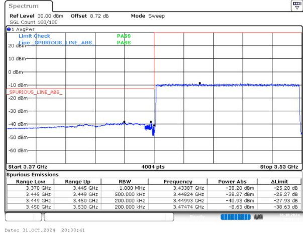
n77(3450-3550) SCS=30kHz DFT_QPSK BW=80MHz LowChannel=632668 RB=216@0
