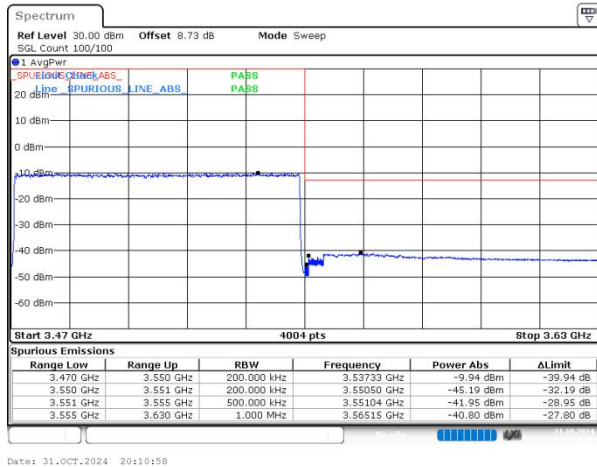
n77(3450-3550) SCS=30kHz DFT_16QAM BW=80MHz HighChannel=634000 RB=216@0
