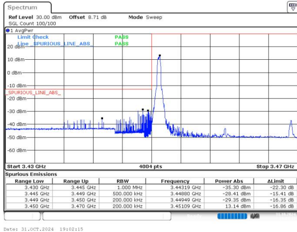
n77(3450-3550) SCS=30kHz DFT_16QAM BW=20MHz LowChannel=630668 RB=1@0
