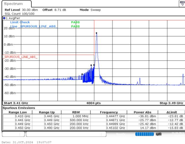
n77(3450-3550) SCS=30kHz DFT_BPSK BW=40MHz LowChannel=631334 RB=1@0
