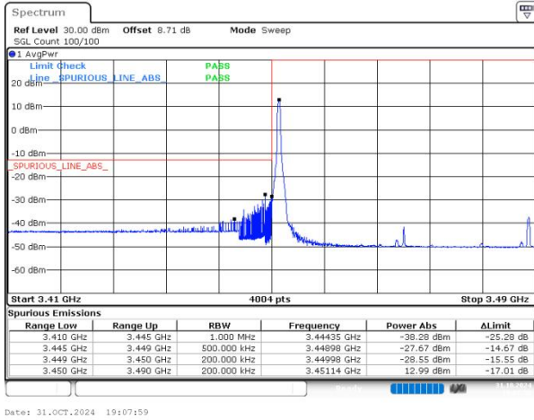
n77(3450-3550) SCS=30kHz DFT_QPSK BW=40MHz LowChannel=631334 RB=1@0
