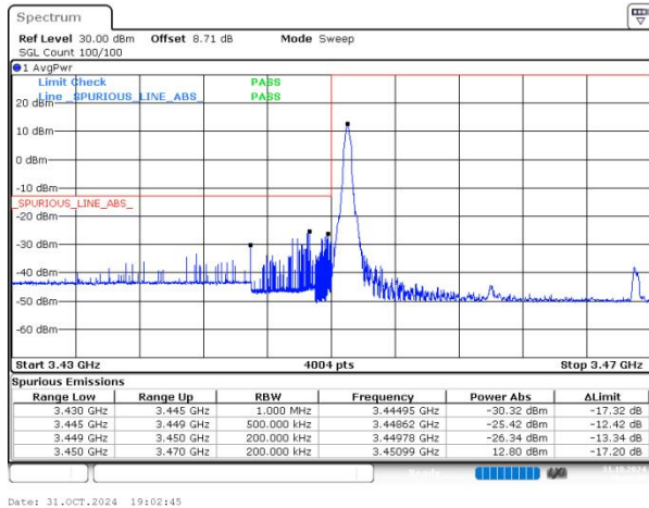
n77(3450-3550) SCS=30kHz DFT_64QAM BW=20MHz LowChannel=630668 RB=1@0
