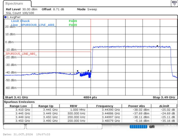
n77(3450-3550) SCS=30kHz DFT_BPSK BW=40MHz LowChannel=631334 RB=100@0
