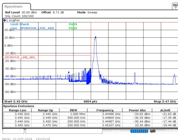
n77(3450-3550) SCS=30kHz DFT_256QAM BW=20MHz LowChannel=630668 RB=1@0
