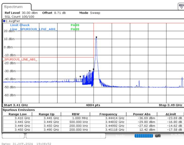
n77(3450-3550) SCS=30kHz DFT_16QAM BW=40MHz LowChannel=631334 RB=1@0
